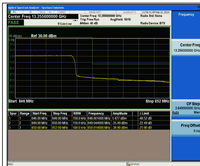
Band26(824-849)-15MHz-QPSK-26965-75RB#0-PASS
