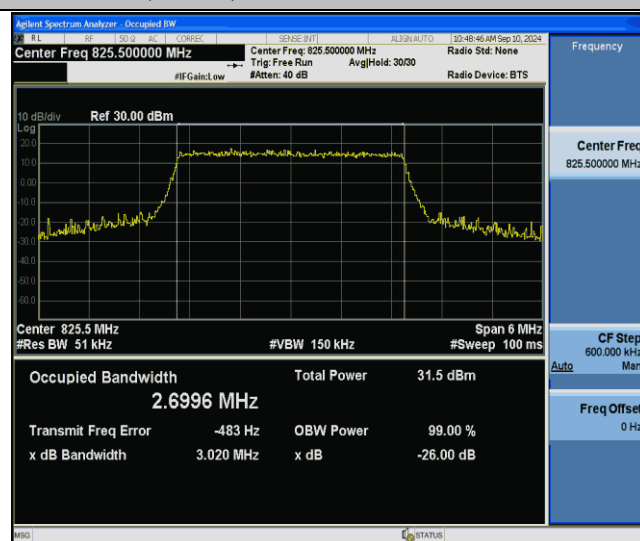
Band26(824-849)-3MHz-16QAM-26805-15RB#0-PASS
