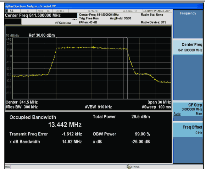
Band26(824-849)-15MHz-256QAM-26965-75RB#0-PASS
