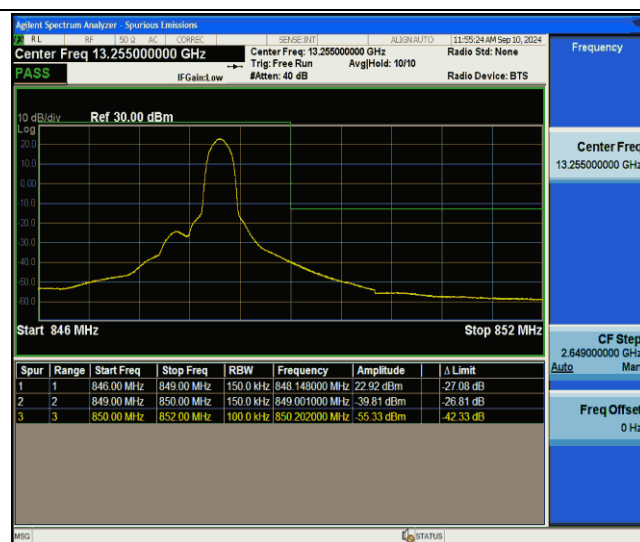
Band26(824-849)-15MHz-QPSK-26965-1RB#74-PASS
