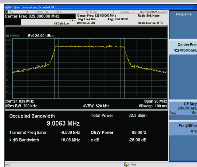
Band26(824-849)-10MHz-16QAM-26840-50RB#0-PASS
