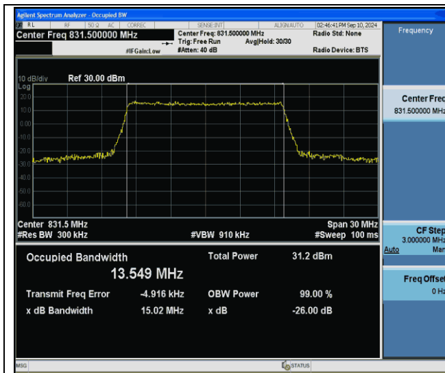
Band26(824-849)-15MHz-64QAM-26865-75RB#0-PASS
