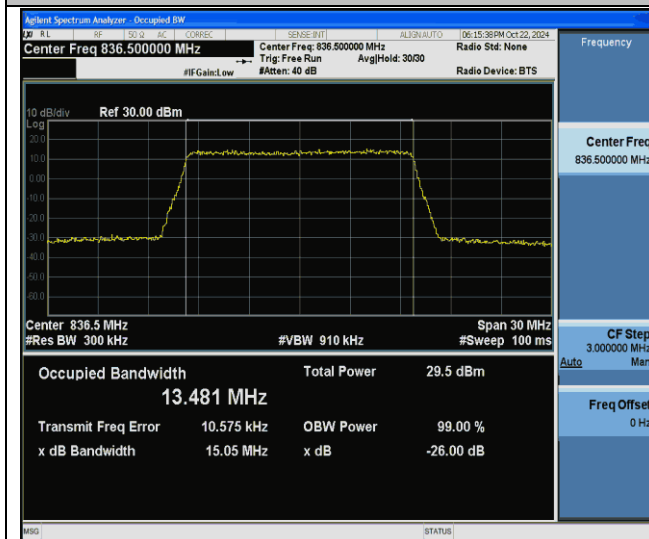
Band26(824-849)-15MHz-256QAM-26915-75RB#0-PASS
