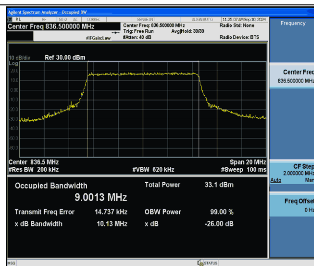
Band26(824-849)-10MHz-QPSK-26915-50RB#0-PASS
