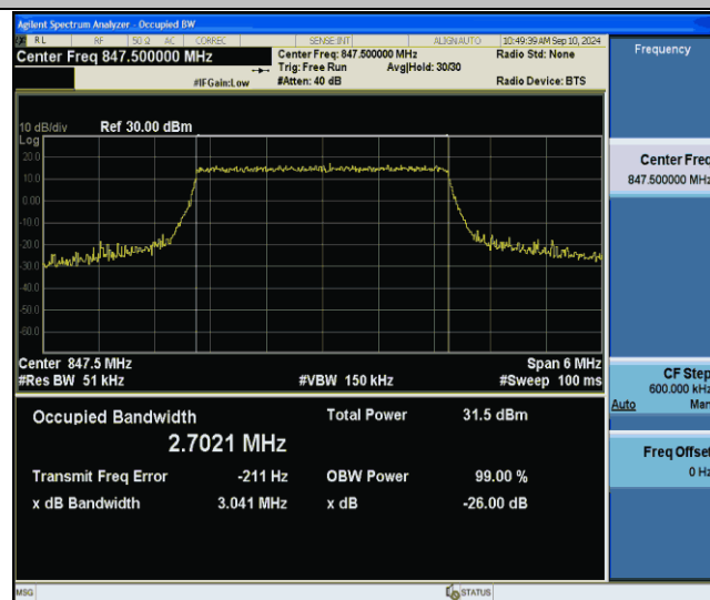
Band26(824-849)-3MHz-16QAM-27025-15RB#0-PASS
