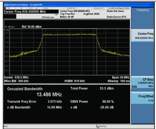
Band26(824-849)-15MHz-QPSK-26915-75RB#0-PASS
