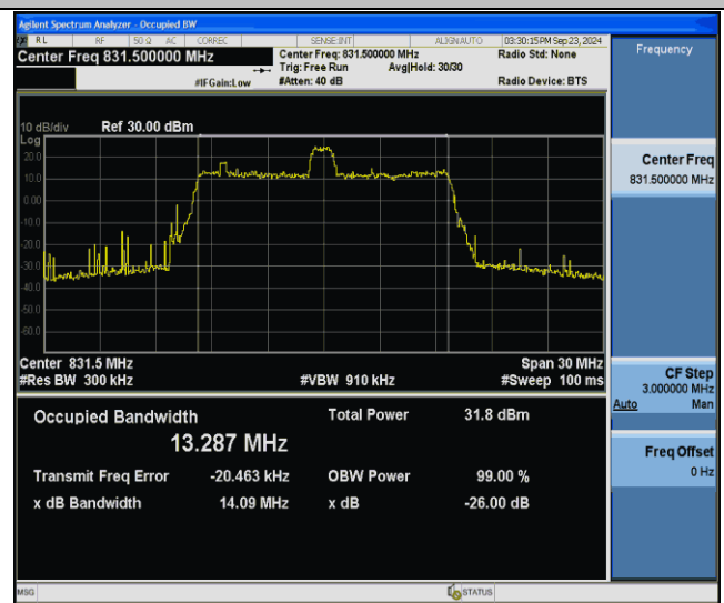
Band26(824-849)-15MHz-256QAM-26865-75RB#0-PASS
