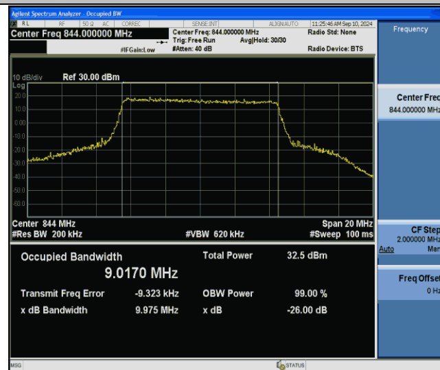
Band26(824-849)-10MHz-16QAM-26990-50RB#0-PASS
