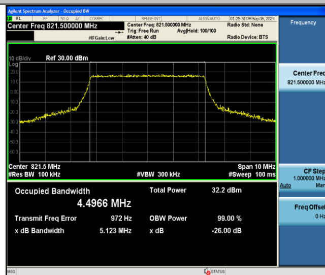
26(814-824)-5MHz-16QAM-26765-25RB#0-PASS
