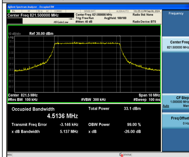
26(814-824)-5MHz-QPSK-26765-25RB#0-PASS
