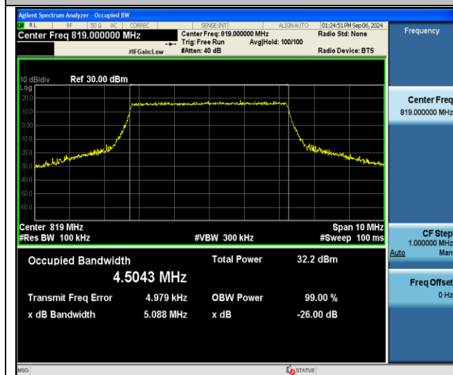
26(814-824)-5MHz-16QAM-26740-25RB#0-PASS
