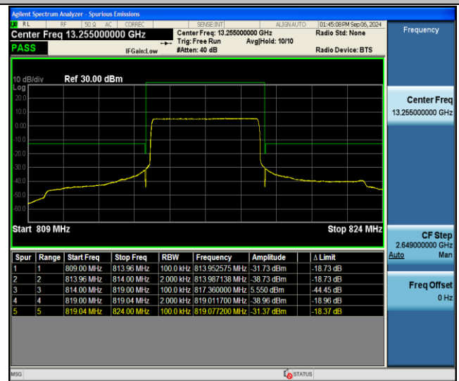
26(814-824)-5MHz-QPSK-26715-25RB#0-PASS
