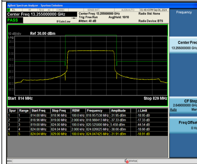
26(814-824)-5MHz-QPSK-26765-25RB#0-PASS
