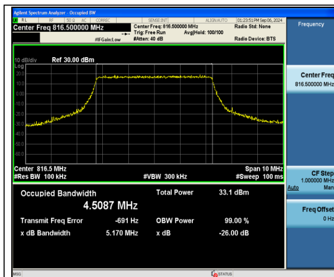
26(814-824)-5MHz-QPSK-26715-25RB#0-PASS
