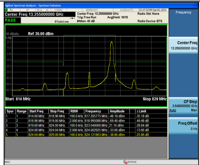
26(814-824)-5MHz-QPSK-26765-1RB#24-PASS
