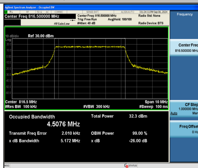
26(814-824)-5MHz-16QAM-26715-25RB#0-PASS
