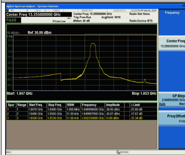
Band25-5MHz-QPSK-26065-1RB#0-PASS
