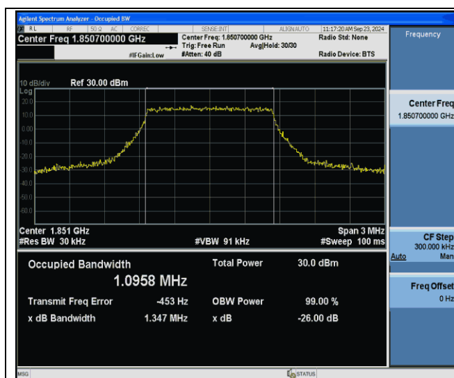
Band25-1.4MHz-64QAM-26047-6RB#0-PASS
