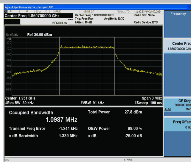
Band25-1.4MHz-256QAM-26047-6RB#0-PASS
