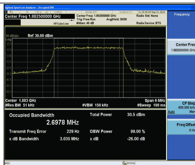
Band25-3MHz-64QAM-26365-15RB#0-PASS
