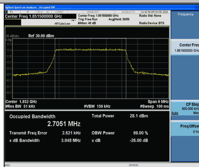
Band25-3MHz-256QAM-26055-15RB#0-PASS
