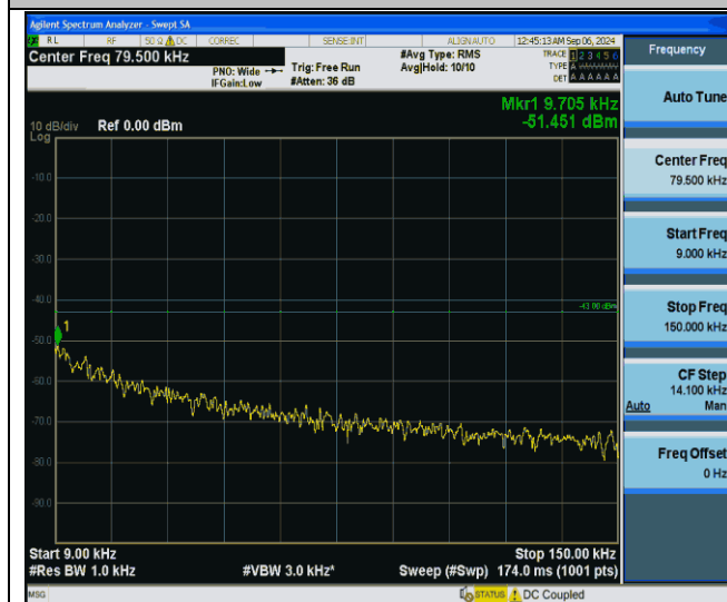
Band25-20MHz-QPSK-26590-1RB#0-0.009~0.15-PASS
