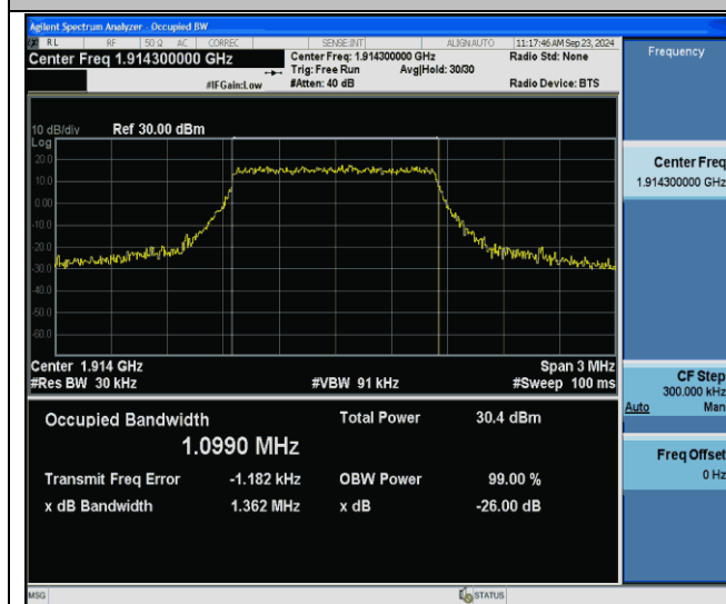
Band25-1.4MHz-64QAM-26683-6RB#0-PASS
