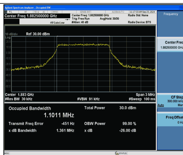
Band25-1.4MHz-64QAM-26365-6RB#0-PASS
