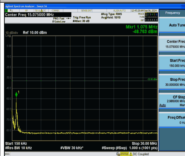
Band25-20MHz-QPSK-26590-1RB#0-0.15~30-PASS
