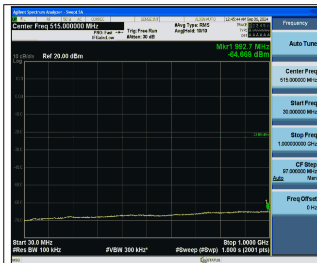
Band25-20MHz-QPSK-26590-1RB#0-30~1000-PASS
