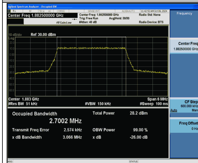
Band25-3MHz-256QAM-26365-15RB#0-PASS
