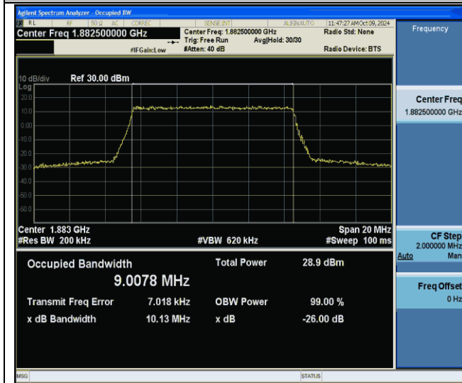
Band25-10MHz-256QAM-26365-50RB#0-PASS
