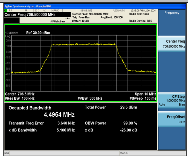
Band17-5MHz-256QAM-23755-25RB#0-PASS
