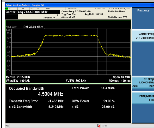
Band17-5MHz-64QAM-23825-25RB#0-PASS
