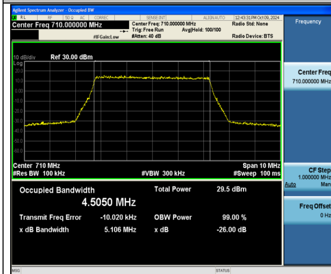
Band17-5MHz-256QAM-23790-25RB#0-PASS
