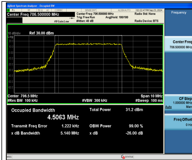
Band17-5MHz-64QAM-23755-25RB#0-PASS
