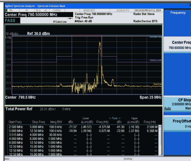
NTNV-Band14-5MHz-256QAM-23305-1RB#24-5.00-12.50-PASS
