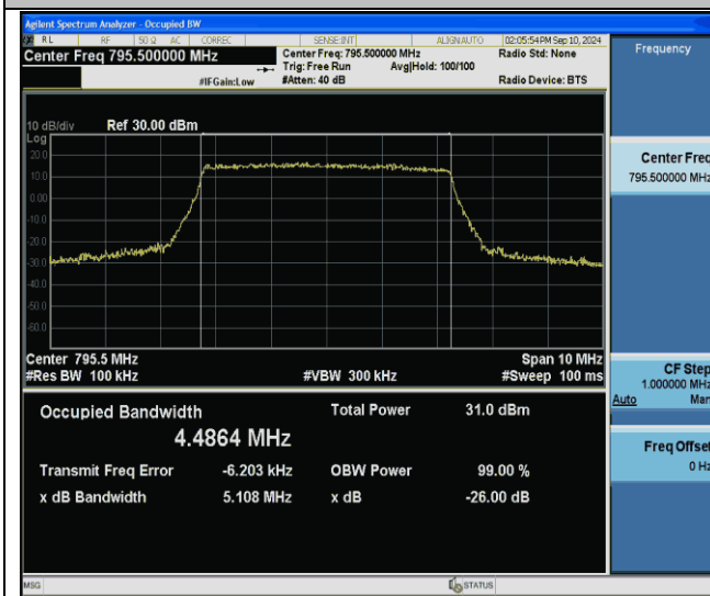
Band14-5MHz-64QAM-23355-25RB#0-PASS
