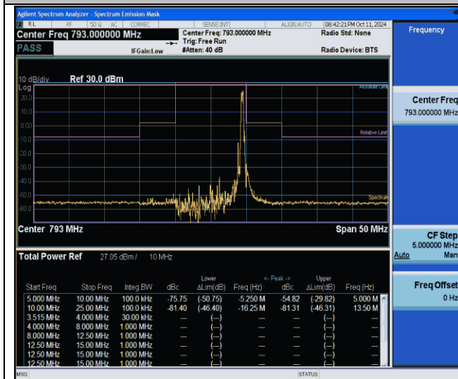
NTVN-Band14-10MHz-QPSK-23330-1RB#49-10.00-5.00-PASS
