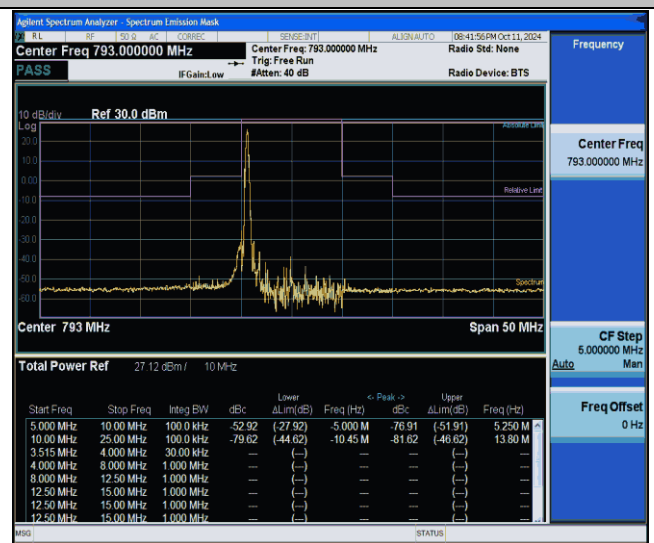
NTNV-Band14-10MHz-QPSK-23330-1RB#0-10.00-25.00-PASS
