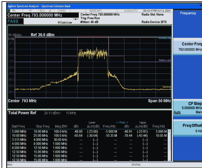
NTVN-Band14-10MHz-QPSK-23330-50RB#0-5.00-5.00-PASS
