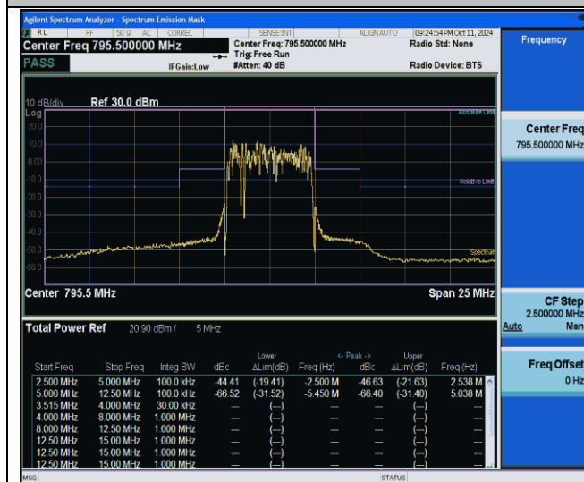
NTNV-Band14-5MHz-256QAM-23355-25RB#0--12.50--5.00-PASS
