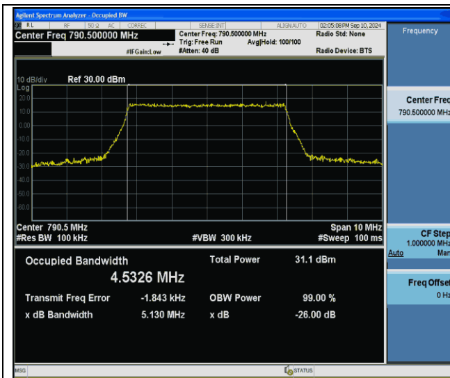
Band14-5MHz-64QAM-23305-25RB#0-PASS
