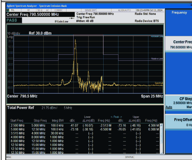
NTNV-Band14-5MHz-256QAM-23305-1RB#0-2.50-5.00-PASS
