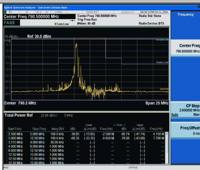
NTNV-Band14-5MHz-16QAM-23305-1RB#0-2.50-5.00-PASS
