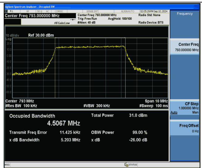
Band14-5MHz-64QAM-23330-25RB#0-PASS
