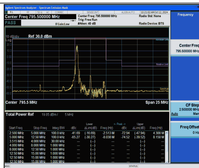
NTNV-Band14-5MHz-256QAM-23355-1RB#0--5.00--2.50-PASS
