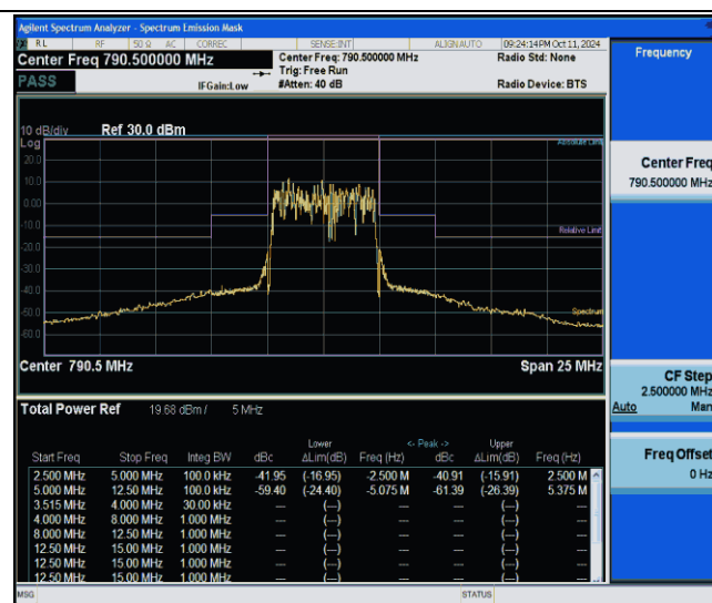
NTNV-Band14-5MHz-256QAM-23305-25RB#0-5.00-12.50-PASS
