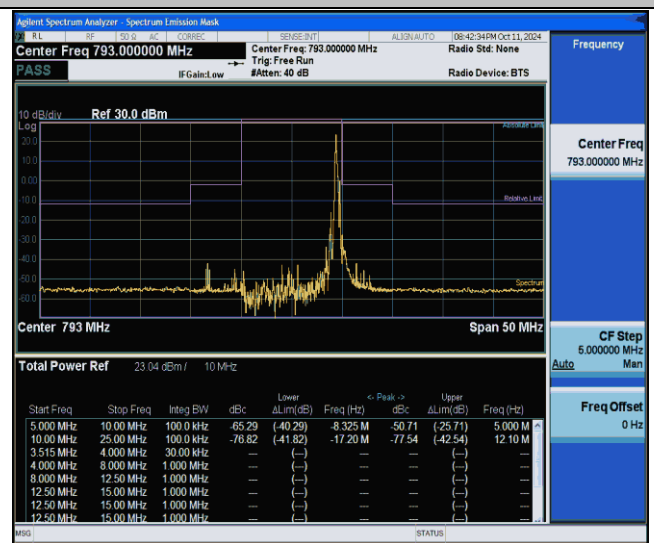
NTNV-Band14-10MHz-16QAM-23330-1RB#49--25.00--10.00-PASS
