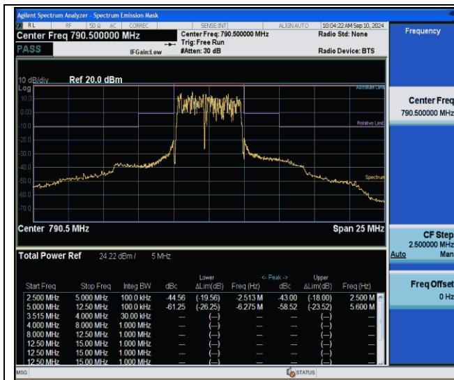
NTNV-Band14-5MHz-QPSK-23305-25RB#0--2.50-2.50-PASS
