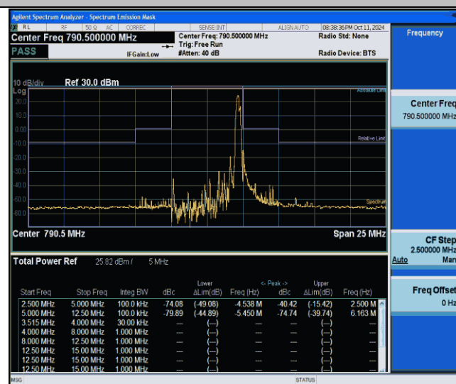
NTNV-Band14-5MHz-16QAM-23305-1RB#24--12.50--5.00-PASS
