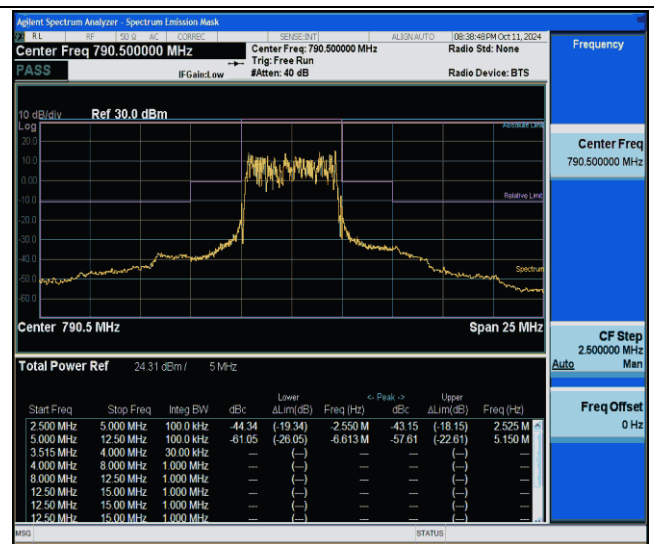
NTNV-Band14-5MHz-QPSK-23305-25RB#0-2.50-5.00-PASS
