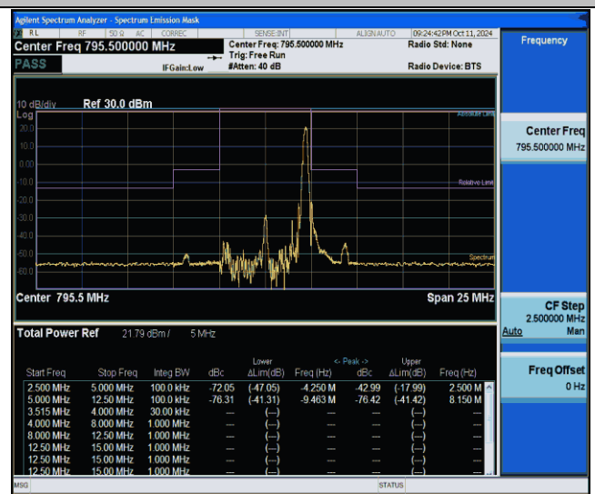
NTNV-Band14-5MHz-256QAM-23355-1RB#24--5.00--2.50-PASS
