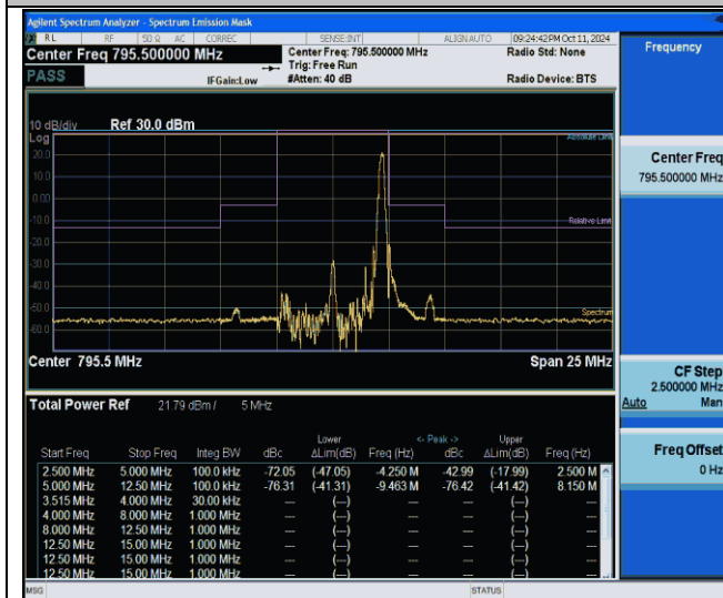
NTNV-Band14-5MHz-256QAM-23355-1RB#24--2.50-2.50-PASS
