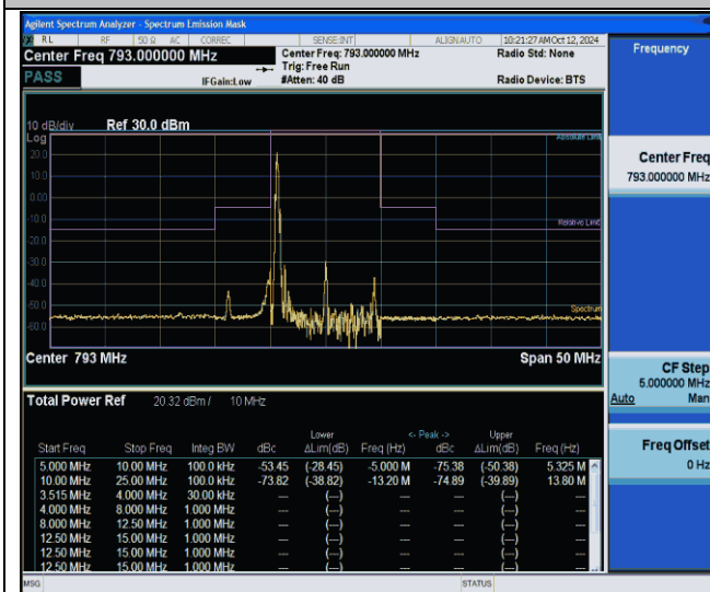
NTNV-Band14-10MHz-256QAM-23330-1RB#0-5.00-10.00-PASS
