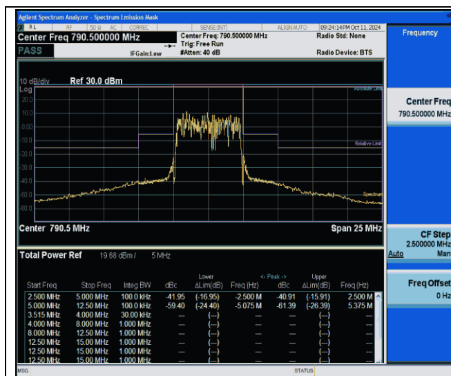
NTNV-Band14-5MHz-256QAM-23305-25RB#0--2.50-2.50-PASS
