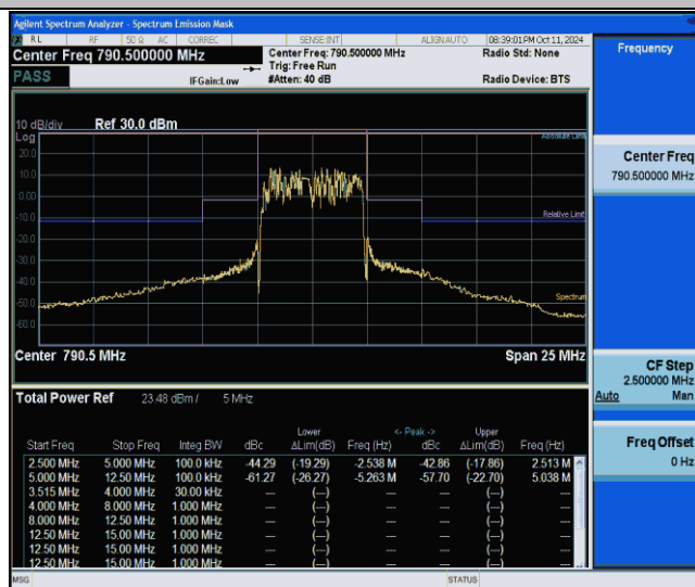
NTNV-Band14-5MHz-16QAM-23305-25RB#0--12.50--5.00-PASS
