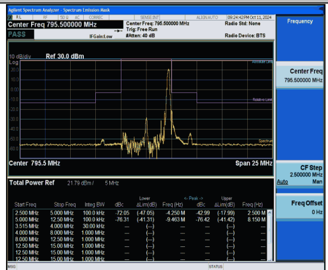
NTNV-Band14-5MHz-256QAM-23355-1RB#24-5.00-12.50-PASS
