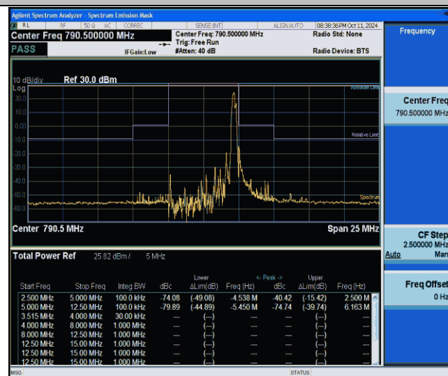
NTNV-Band14-5MHz-16QAM-23305-1RB#24--2.50-2.50-PASS
