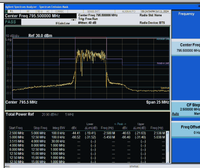
NTNV-Band14-5MHz-256QAM-23355-25RB#0--5.00--2.50-PASS
