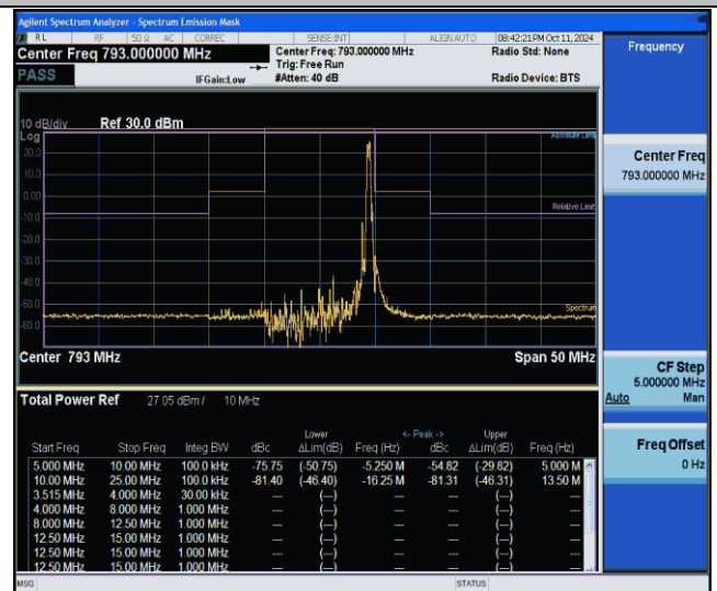
NTVN-Band14-10MHz-QPSK-23330-1RB#49-5.00-5.00-PASS
