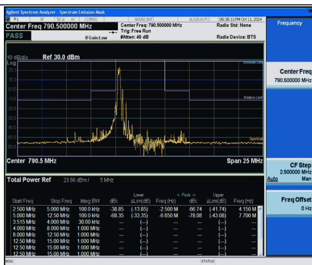
NTNV-Band14-5MHz-16QAM-23305-1RB#0--12.50--5.00-PASS
