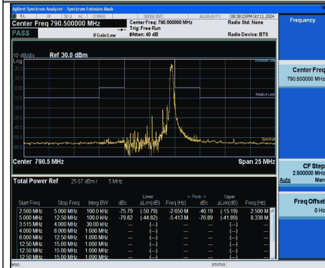
NTNV-Band14-5MHz-QPSK-23305-1RB#24--5.00--2.50-PASS
