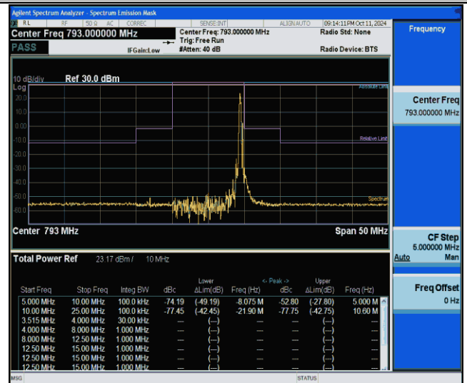
NTNV-Band14-10MHz-64QAM-23330-1RB#49--10.00--5.00-PASS
