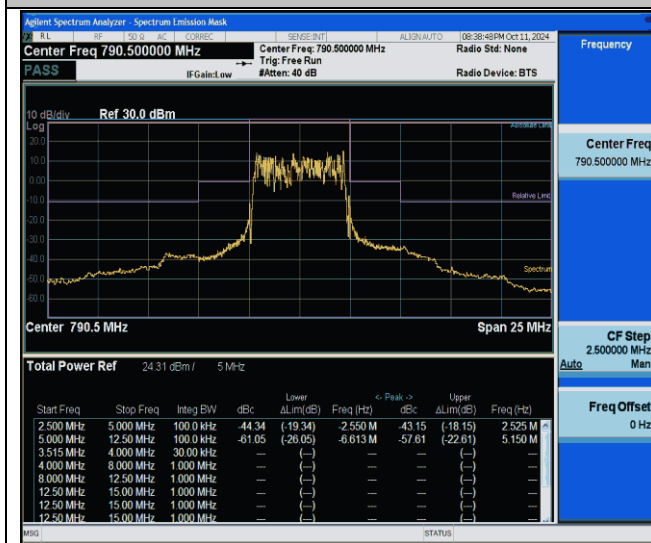
NTNV-Band14-5MHz-QPSK-23305-25RB#0-5.00-12.50-PASS
