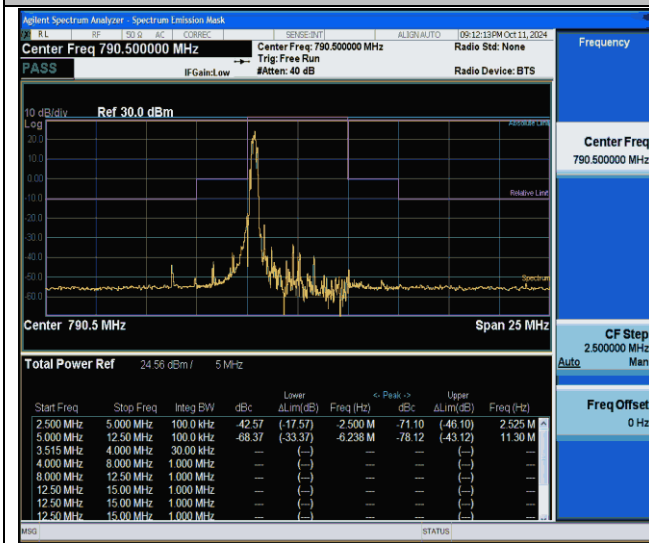
NTVN-Band14-5MHz-64QAM-23305-1RB#0--5.00--2.50-PASS
