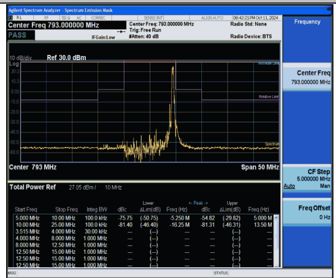
NTVN-Band14-10MHz-QPSK-23330-1RB#49-25.00-10.00-PASS
