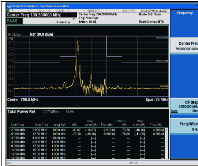
NTNV-Band14-5MHz-256QAM-23305-1RB#0--12.50--5.00-PASS
