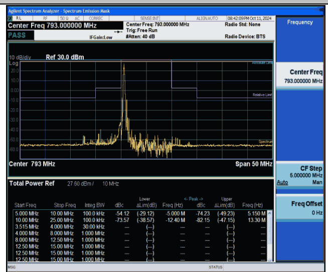
NTNV-Band14-10MHz-16QAM-23330-1RB#0-5.00-10.00-PASS
