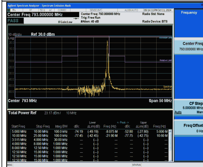
NTNV-Band14-10MHz-64QAM-23330-1RB#49--25.00--10.00-PASS
