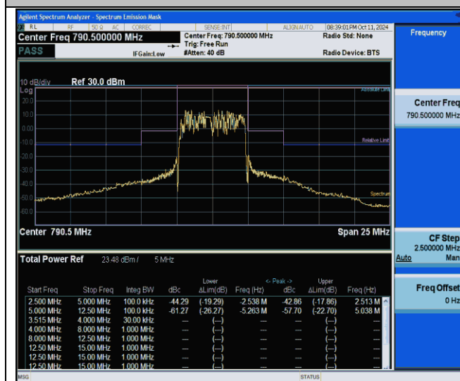
NTNV-Band14-5MHz-16QAM-23305-25RB#0-5.00-12.50-PASS
