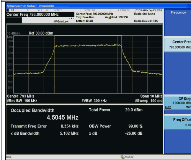
Band14-5MHz-256QAM-23330-25RB#0-PASS
