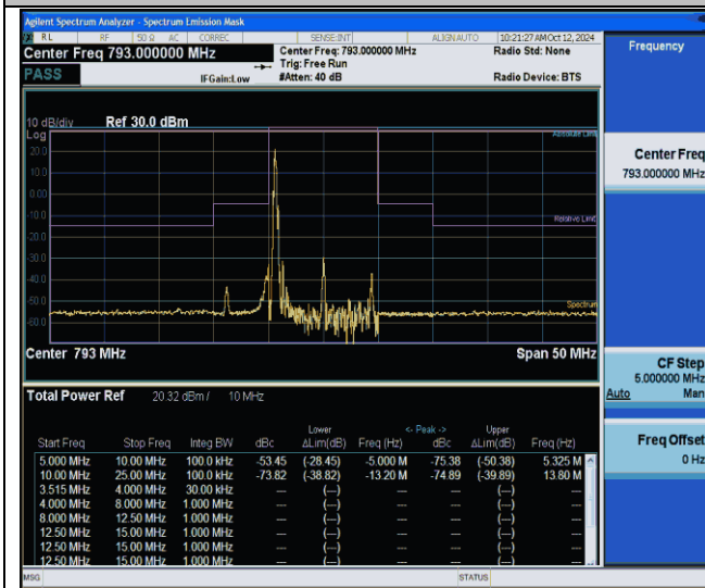
NTNV-Band14-10MHz-256QAM-23330-1RB#0--25.00--10.00-PASS
