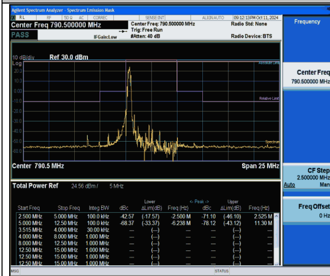
NTVN-Band14-5MHz-64QAM-23305-1RB#0-5.00-12.50-PASS
