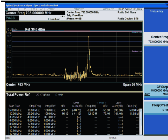
NTVN-Band14-10MHz-256QAM-23330-1RB#49--25.00--10.00-
