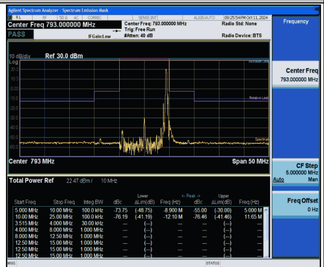
NTVN-Band14-10MHz-256QAM-23330-1RB#49--10.00--5.00-
