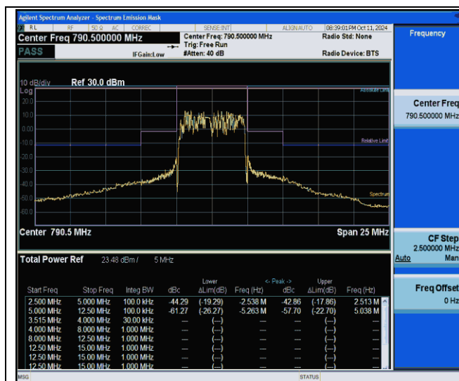
NTNV-Band14-5MHz-16QAM-23305-25RB#0--5.00--2.50-PASS
