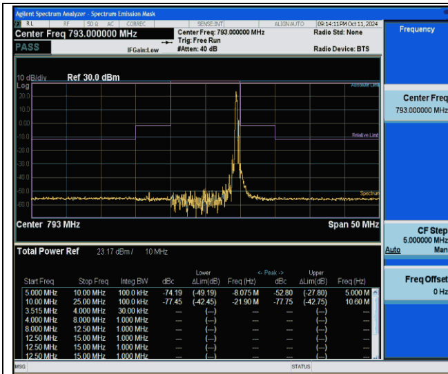
NTNV-Band14-10MHz-64QAM-23330-1RB#49--5.00-5.00-PASS
