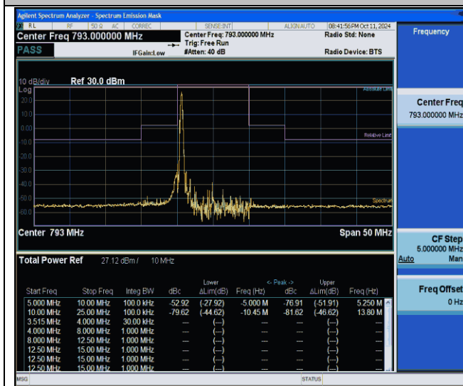
NTNV-Band14-10MHz-QPSK-23330-1RB#0-5.00-10.00-PASS
