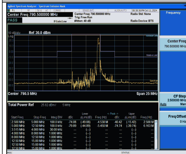
NTNV-Band14-5MHz-16QAM-23305-1RB#24--5.00--2.50-PASS
