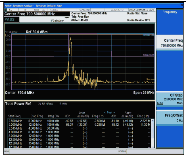
NTVN-Band14-5MHz-64QAM-23305-1RB#0--12.50--5.00-PASS
