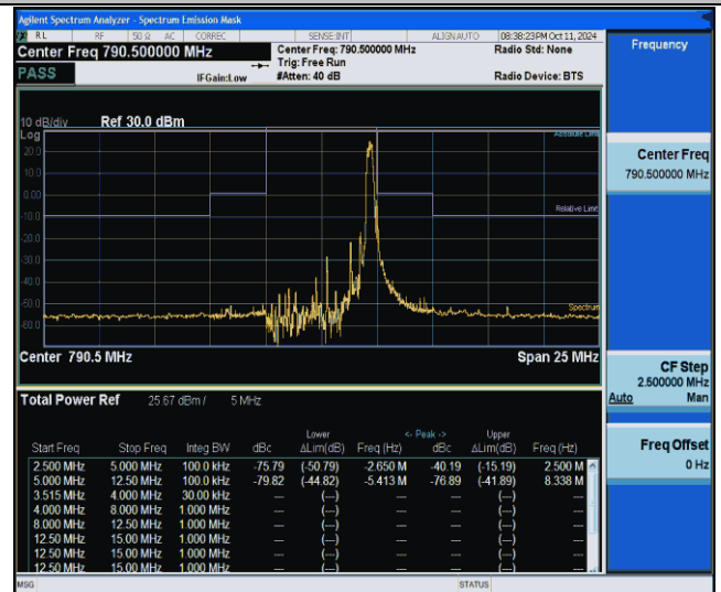
NTNV-Band14-5MHz-QPSK-23305-1RB#24--2.50-2.50-PASS
