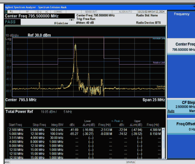
NTNV-Band14-5MHz-256QAM-23355-1RB#0-5.00-12.50-PASS
