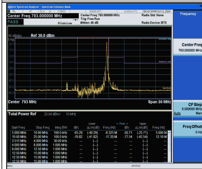
NTNV-Band14-10MHz-16QAM-23330-1RB#49--10.00--5.00-PASS
