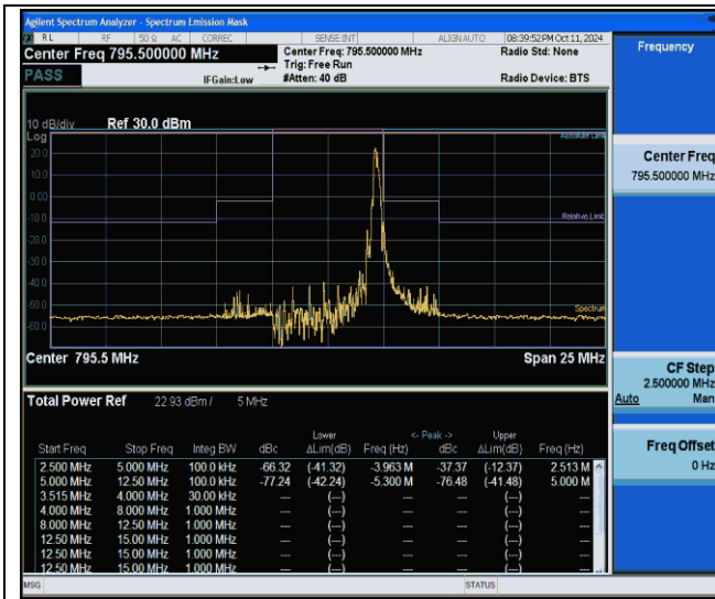
NTVN-Band14-5MHz-16QAM-23355-1RB#24-2.50-5.00-PASS
