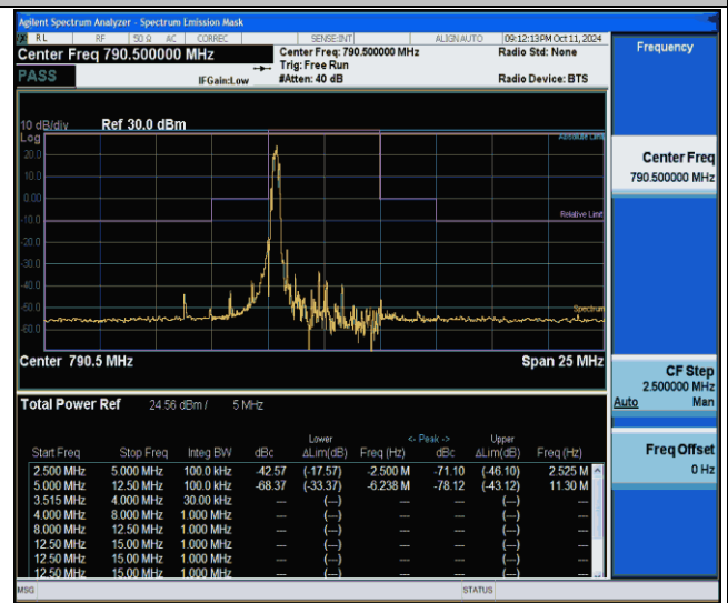
NTVN-Band14-5MHz-64QAM-23305-1RB#0-2.50-5.00-PASS
