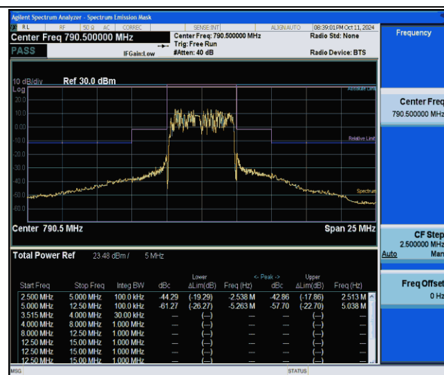
NTNV-Band14-5MHz-16QAM-23305-25RB#0-2.50-5.00-PASS
