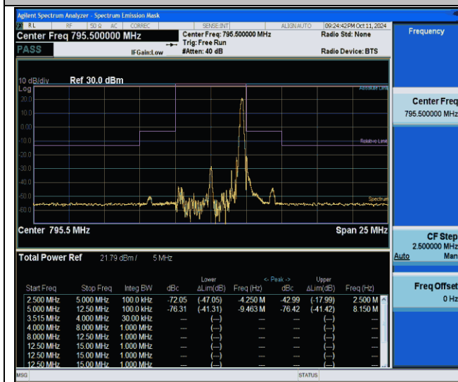
NTNV-Band14-5MHz-256QAM-23355-1RB#24--12.50--5.00-PASS
