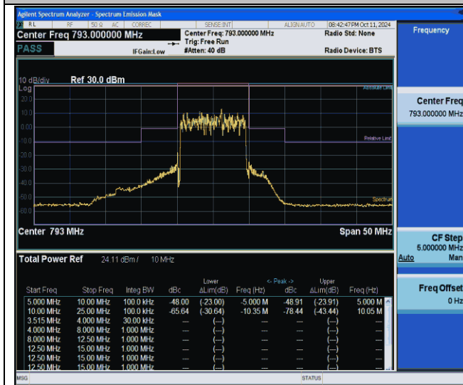
NTVN-Band14-10MHz-QPSK-23330-50RB#0-10.00-25.00-PASS
