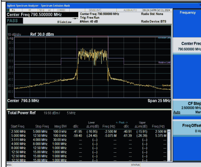
NTNV-Band14-5MHz-256QAM-23305-25RB#0--12.50--5.00-PASS
