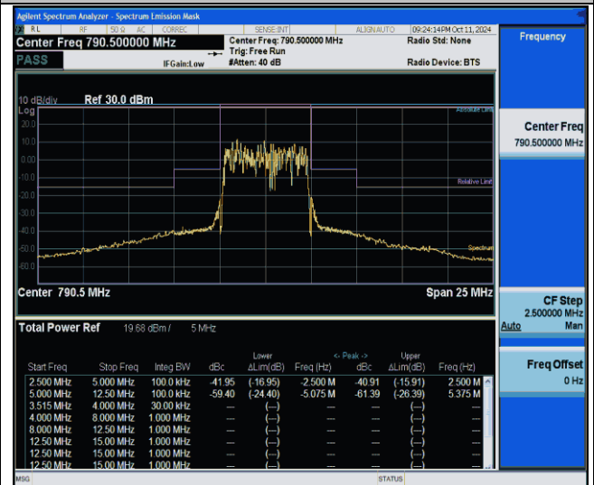
NTNV-Band14-5MHz-256QAM-23305-25RB#0--5.00--2.50-PASS
