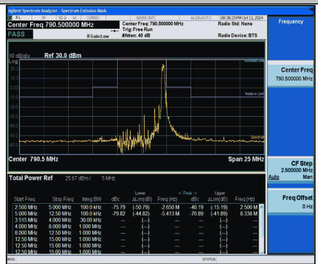
NTNV-Band14-5MHz-QPSK-23305-1RB#24--12.50--5.00-PASS
