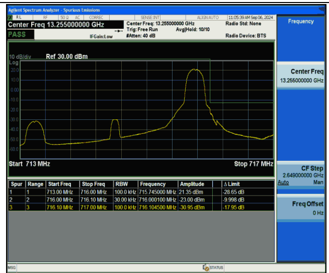
Band12-3MHz-QPSK-23165-1RB#14-PASS
