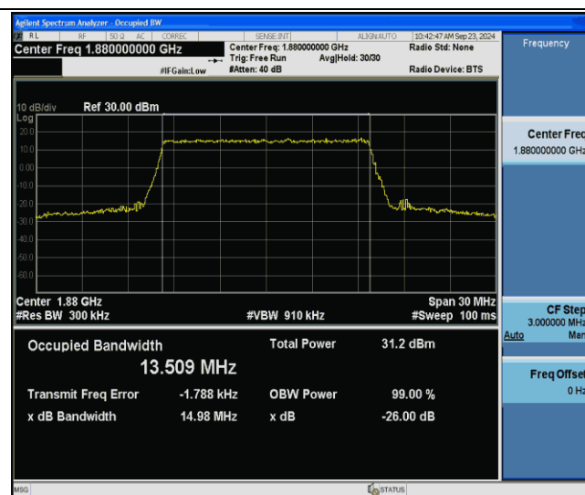
Band2-15MHz-64QAM-18900-75RB#0-PASS
