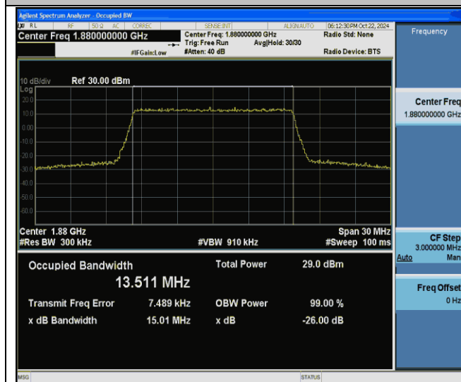
Band2-15MHz-256QAM-18900-75RB#0-PASS
