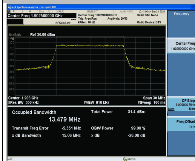
Band2-15MHz-64QAM-19125-75RB#0-PASS
