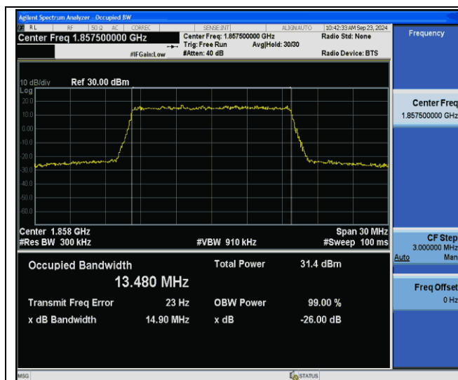
Band2-15MHz-64QAM-18675-75RB#0-PASS
