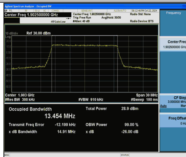
Band2-15MHz-256QAM-19125-75RB#0-PASS
