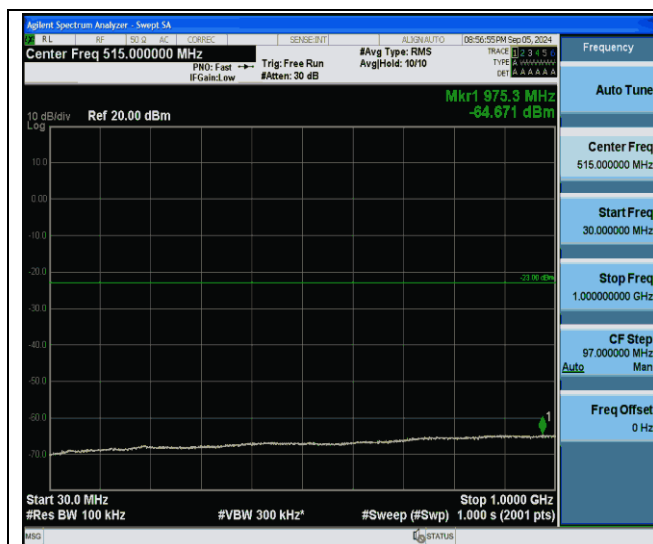
Band2-20MHz-QPSK-19100-1RB#0-30~1000-PASS
