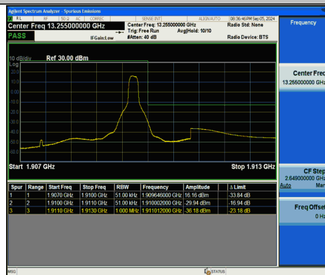
Band2-5MHz-QPSK-19175-1RB#24-PASS
