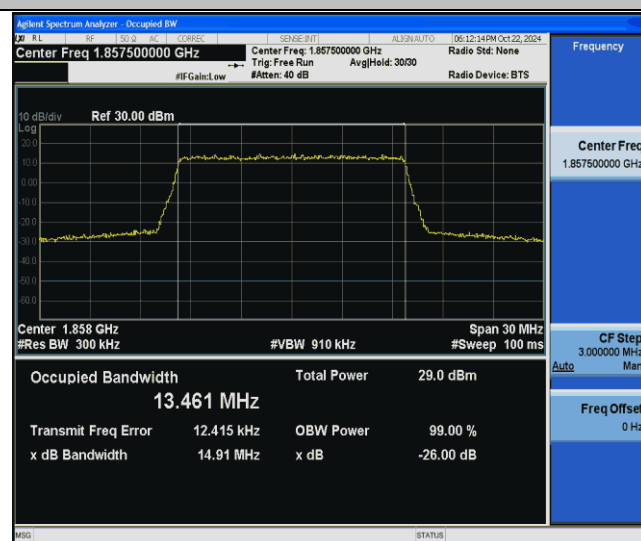
Band2-15MHz-256QAM-18675-75RB#0-PASS
