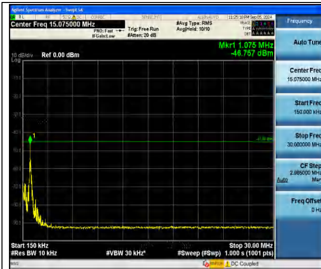
Band7-20MHz-QPSK-21100-1RB#0-0.15~30-PASS
