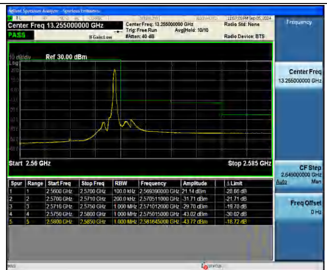
Band7-10MHz-QPSK-21400-1RB#49-PASS
