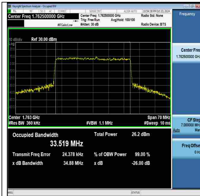
NTNV-n66-PC3-15-35-H-CP-256QAM-Outer_Full-Ant1- PASS
