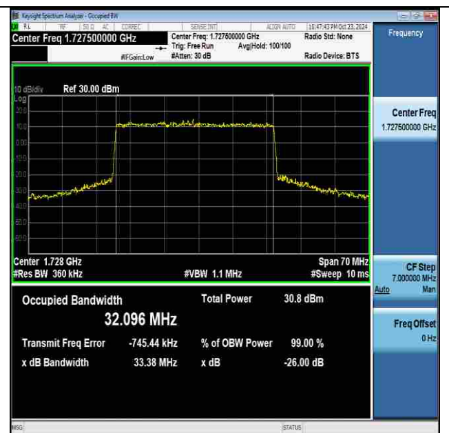
NTNV-n66-PC3-15-35-L-DFT-16QAM-Outer_Full-Ant1- PASS
