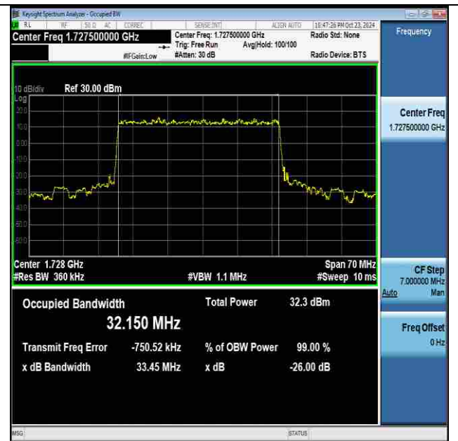
NTNV-n66-PC3-15-35-L-DFT-BPSK-Outer_Full-Ant1- PASS
