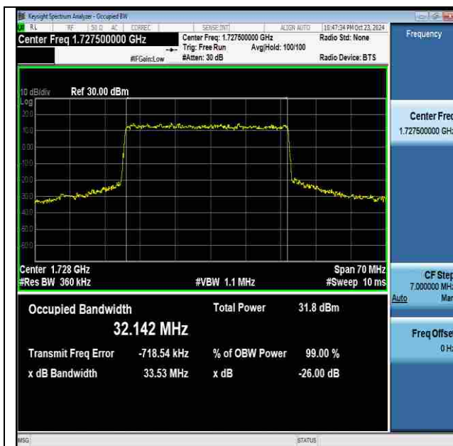
NTNV-n66-PC3-15-35-L-DFT-QPSK-Outer_Full-Ant1- PASS
