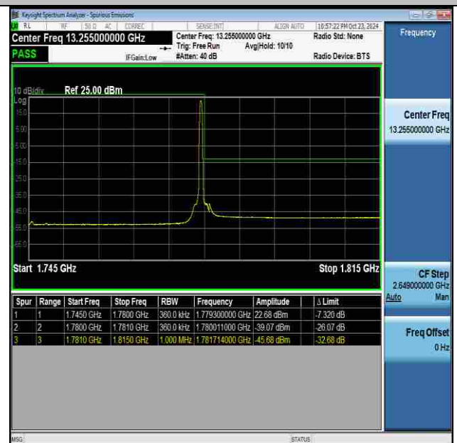
NTNV-n66-PC3-15-35-H-DFT-BPSK-Edge_1RB_Right-PASS
