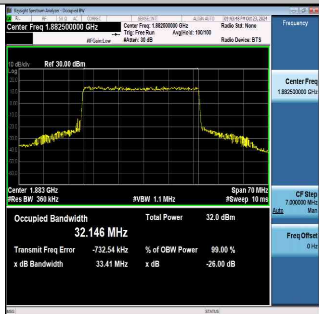
NTNV-n25-PC3-15-35-M-DFT-QPSK-Outer_Full-Ant1- PASS
