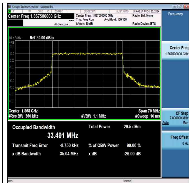
NTNV-n25-PC3-15-35-L-CP-64QAM-Outer_Full-Ant1- PASS
