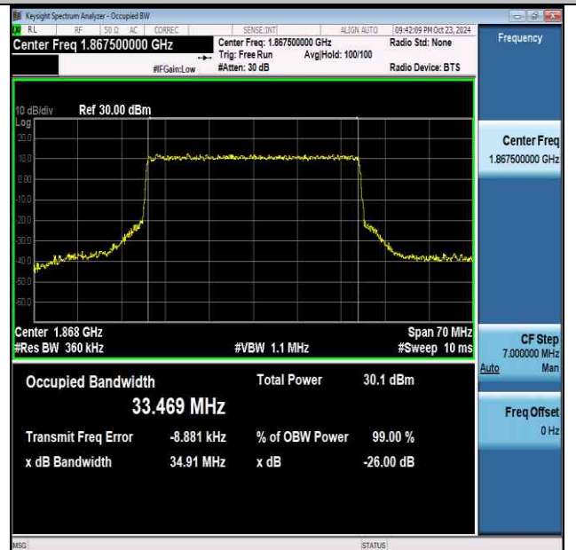
NTNV-n25-PC3-15-35-L-CP-16QAM-Outer_Full-Ant1- PASS
