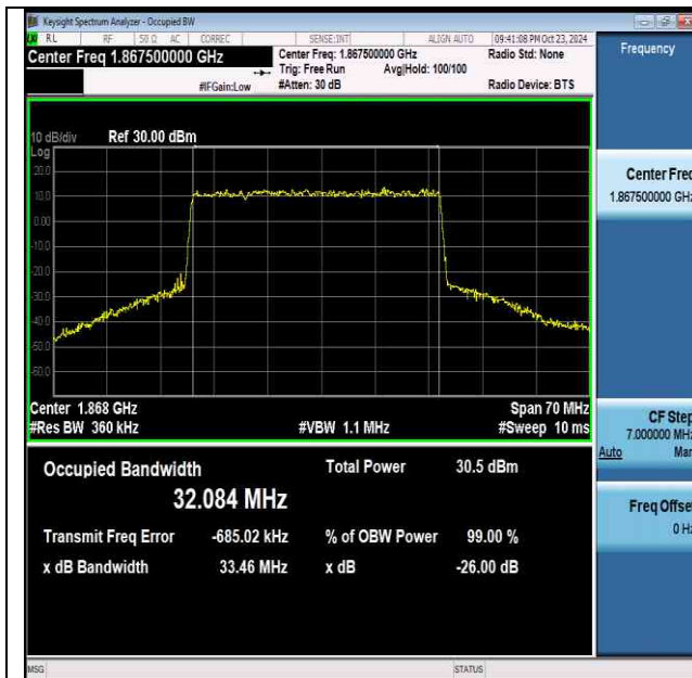
NTNV-n25-PC3-15-35-L-DFT-64QAM-Outer_Full-Ant1- PASS
