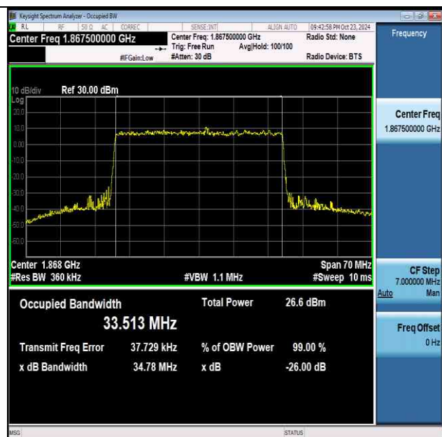
NTNV-n25-PC3-15-35-L-CP-256QAM-Outer_Full-Ant1- PASS
