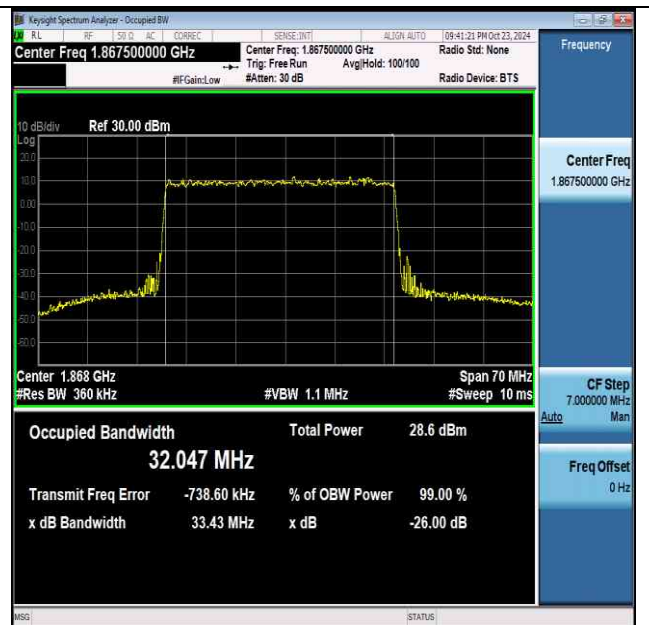
NTNV-n25-PC3-15-35-L-DFT-256QAM-Outer_Full-Ant1- PASS
