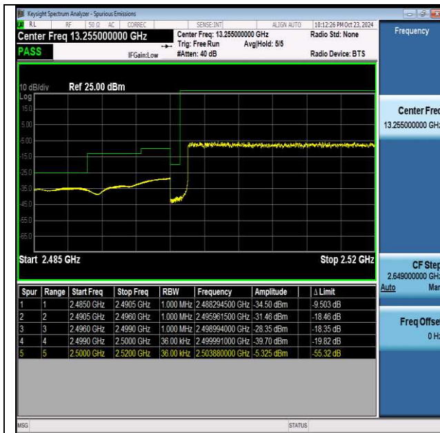
NTNV-n7-PC3-15-35-L-DFT-PI2BPSK-Outer_Full-PASS
