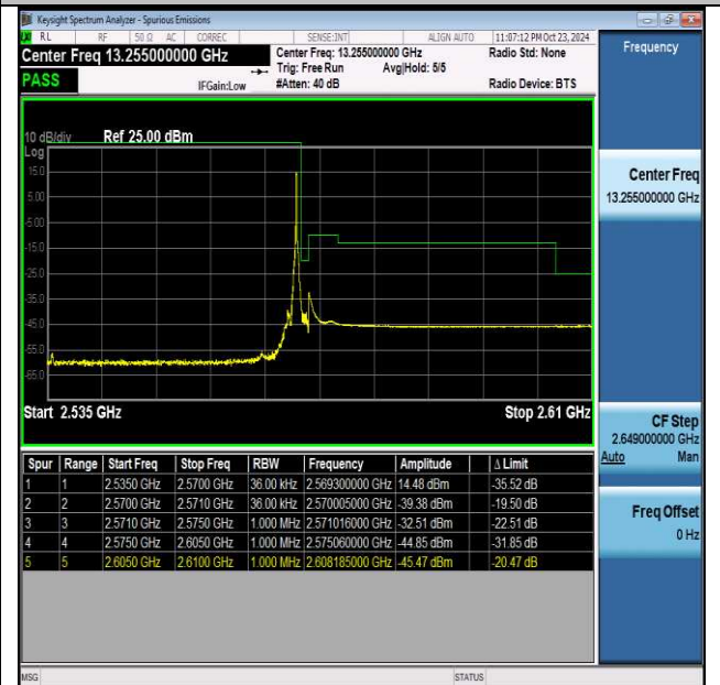
NTNV-n7-PC3-15-35-H-DFT-PI2BPSK-Edge_1RB_Right-PASS
