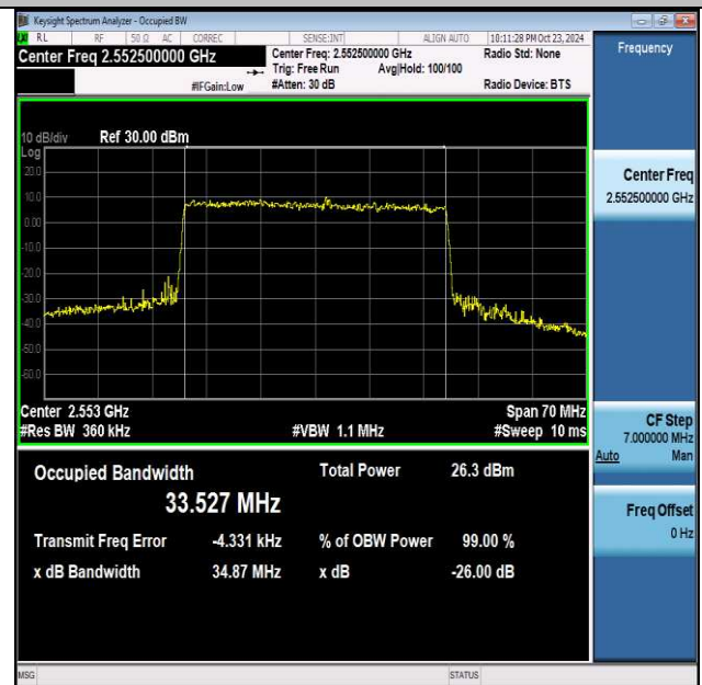
NTNV-n7-PC3-15-35-H-CP-256QAM-Outer_Full-Ant1-PASS
