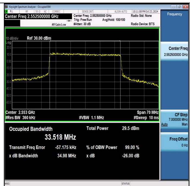
NTNV-n7-PC3-15-35-H-CP-16QAM-Outer_Full-Ant1-PASS
