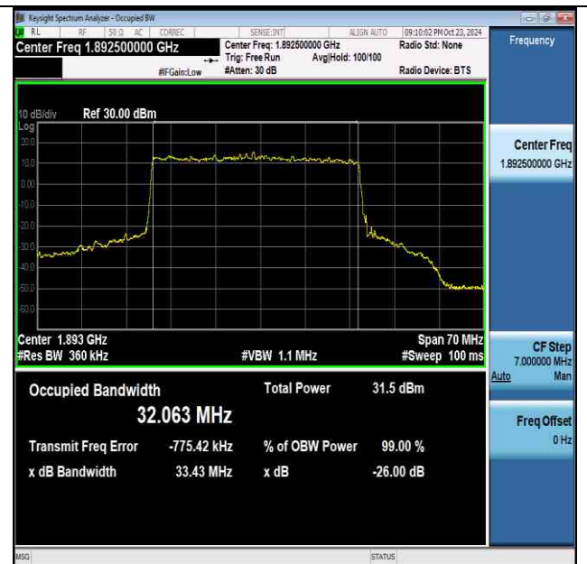
NTNV-n2-PC3-15-35-H-DFT-16QAM-Outer_Full-Ant1-PASS
