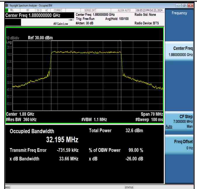
NTNV-n2-PC3-15-35-L-CP-256QAM-Outer_Full-Ant1-PASS
