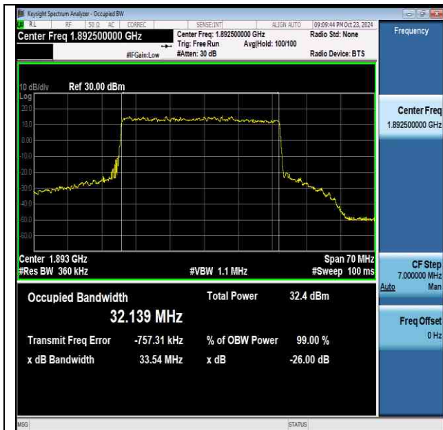
NTNV-n2-PC3-15-35-H-DFT-QPSK-Outer_Full-Ant1-PASS
