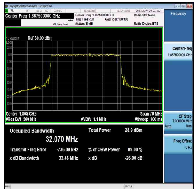
NTNV-n2-PC3-15-35-L-DFT-256QAM-Outer_Full-Ant1- PASS
