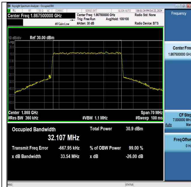
NTNV-n2-PC3-15-35-L-DFT-64QAM-Outer_Full-Ant1- PASS
