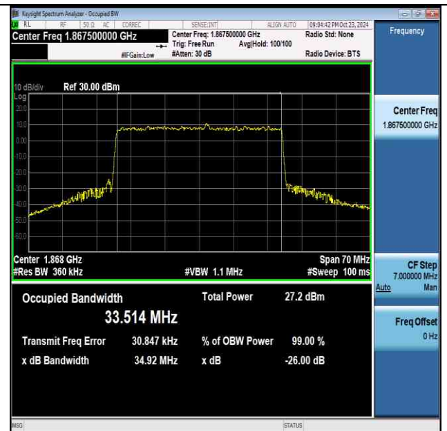
NTNV-n2-PC3-15-35-L-CP-256QAM-Outer_Full-Ant1-PASS
