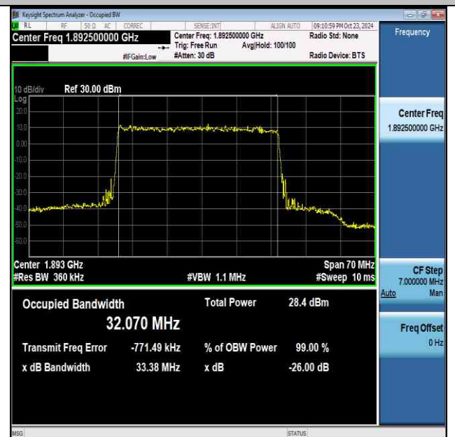
NTNV-n2-PC3-15-35-H-DFT-256QAM-Outer_Full-Ant1-PASS
