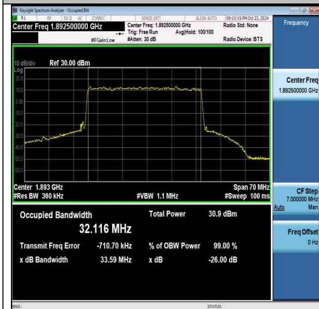
NTNV-n2-PC3-15-35-H-DFT-64QAM-Outer_Full-Ant1-PASS
