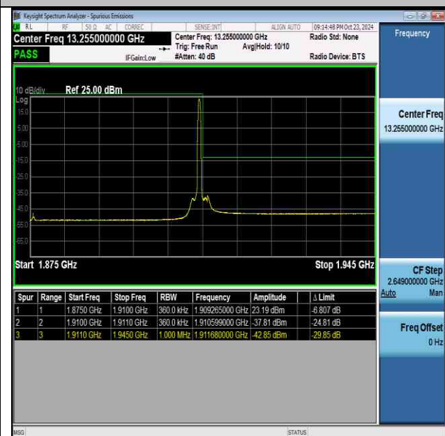
NTNV-n2-PC3-15-35-H-DFT-PI2BPSK-Edge_1RB_Right-PASS
