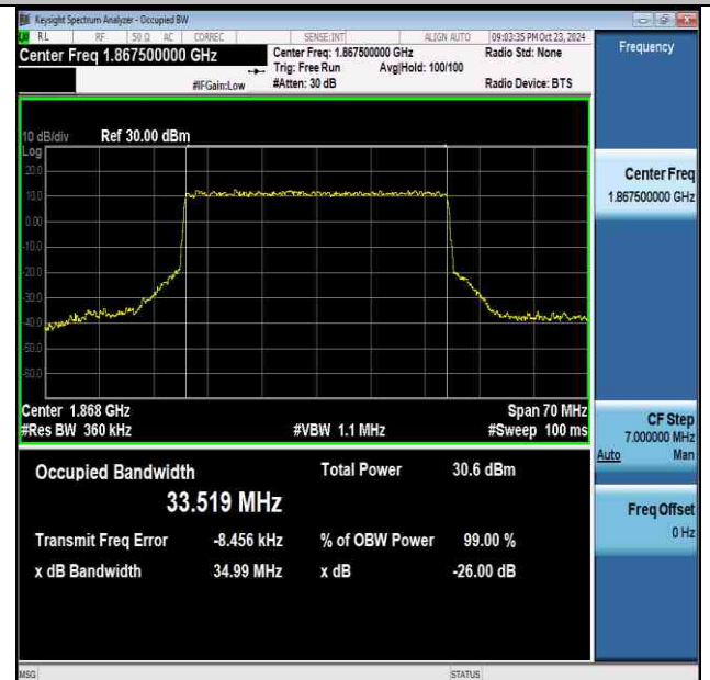
NTNV-n2-PC3-15-35-L-CP-16QAM-Outer_Full-Ant1-PASS
