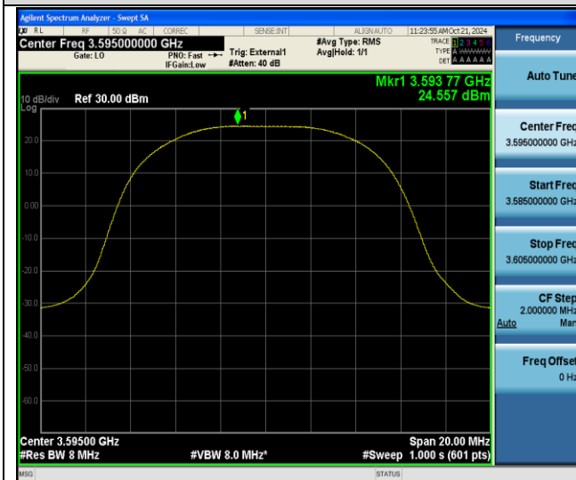
42(3550-3600)-10MHz-QPSK-43540-1RB#24-PASS
