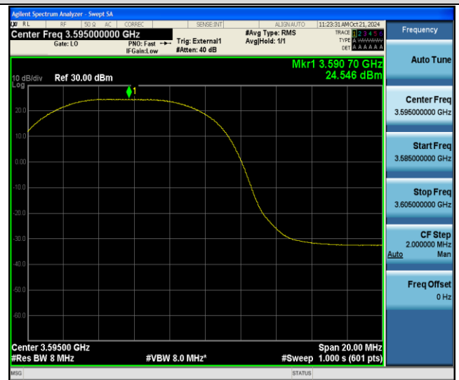
42(3550-3600)-10MHz-QPSK-43540-1RB#0-PASS
