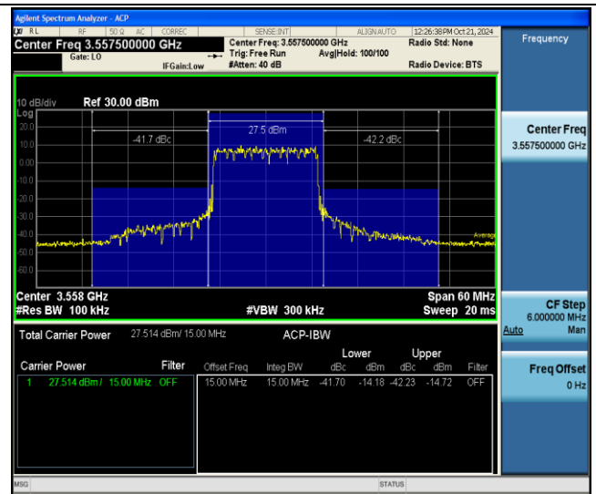
42(3550-3600)-15MHz-QPSK-43165-75RB#0-PASS
