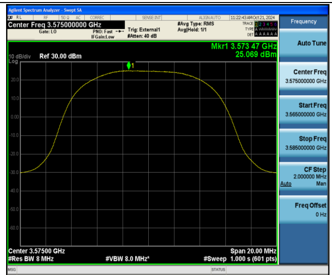
42(3550-3600)-10MHz-QPSK-43340-1RB#24-PASS
