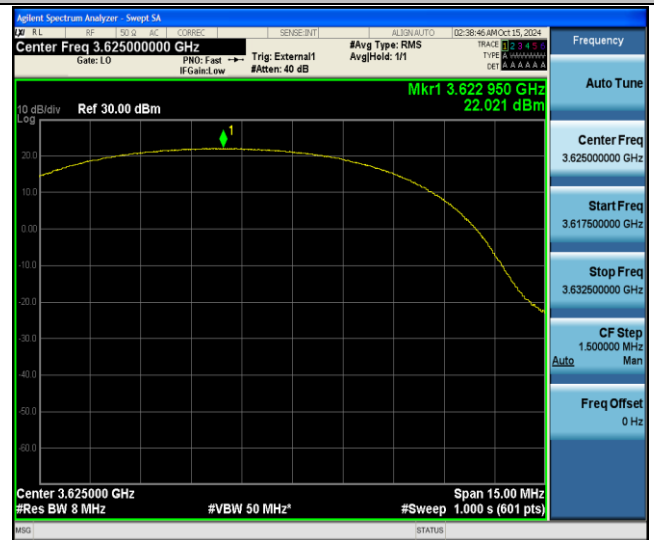
Band48-10MHz-QPSK-55990-25RB#0-PASS
