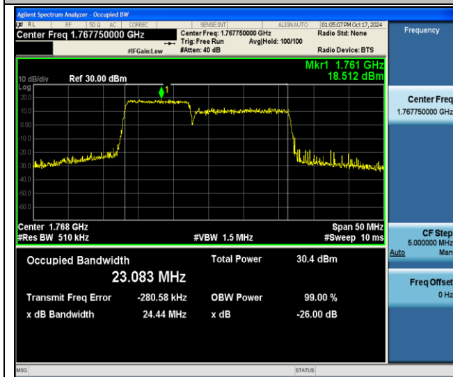
66-66-10MHz-15MHz-64QAM-64QAM-132477-132597-50RB#0-75RB#0-PASS
