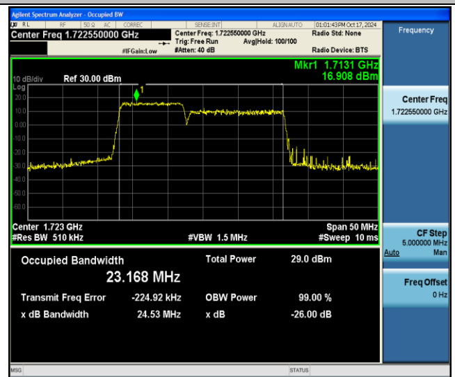
66-66-10MHz-15MHz-256QAM-256QAM-132025-132145-50RB#0-75RB#0-PASS
