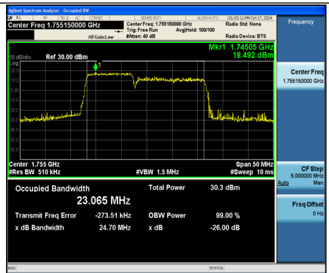
66-66-10MHz-15MHz-64QAM-64QAM-132351-132471-50RB#0-75RB#0-PASS
