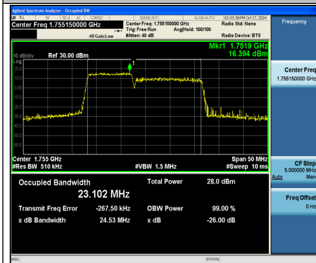
66-66-10MHz-15MHz-256QAM-256QAM-132351-132471-50RB#0-75RB#0-PASS
