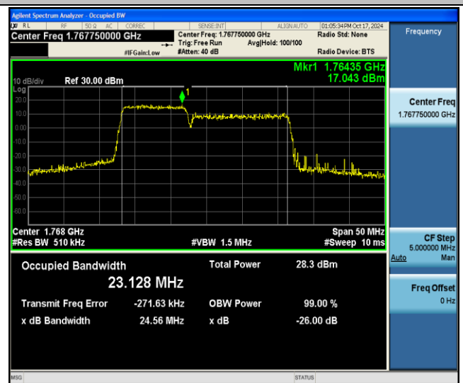
66-66-10MHz-15MHz-256QAM-256QAM-132477-132597-50RB#0-75RB#0-PASS
