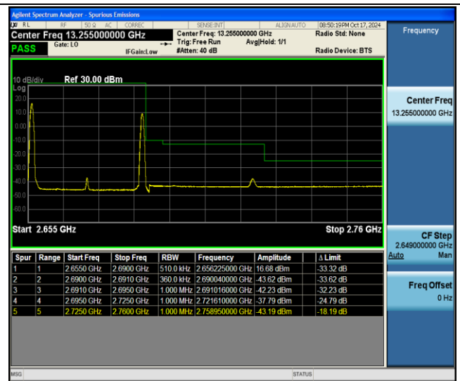
41-41-15MHz-20MHz-QPSK@QPSK-QPSK@QPSK-41319- 41490-1RB#0@75RB#0-1RB#99@100RB#0-PASS
