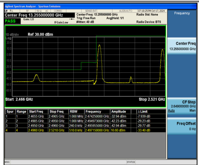
41-41-5MHz-20MHz-16QAM@16QAM-16QAM@16QAM-39683-39800-1RB#0@25RB#0-1RB#99@100RB#0-PASS
