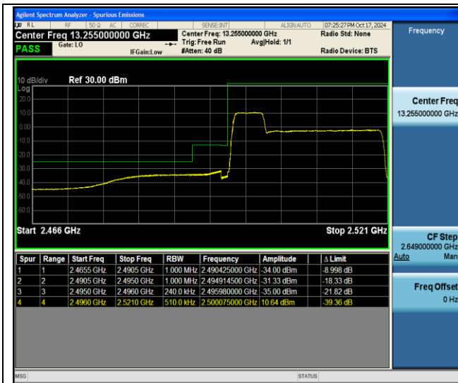
41-41-5MHz-20MHz-64QAM@64QAM-64QAM@64QAM-39683-39800-25RB#0@25RB#0-100RB#0@100RB#0-PASS
