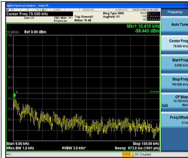
41-41-20MHz-20MHz-QPSK-QPSK-39750-39948-1RB#0-ORB#0-0.009~0.15MHz-PASS
