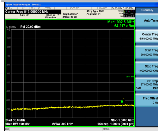
41-41-20MHz-20MHz-QPSK-QPSK-39750-39948-1RB#0-ORB#0-30~1000MHz-PASS
