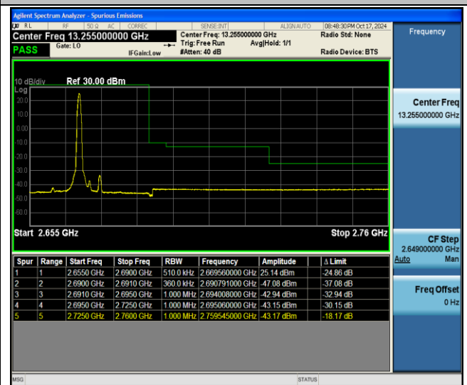
41-41-15MHz-20MHz-QPSK@QPSK-QPSK@QPSK-41319-41490-1RB#74@75RB#0-0RB#0@100RB#0-PASS
