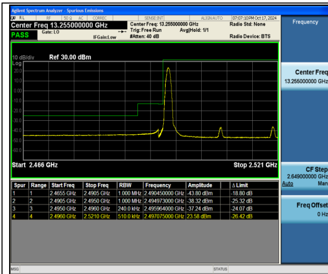
41-41-5MHz-20MHz-16QAM@16QAM-16QAM@16QAM-39683-39800-1RB#0@25RB#0-0RB#0@100RB#0-PASS
