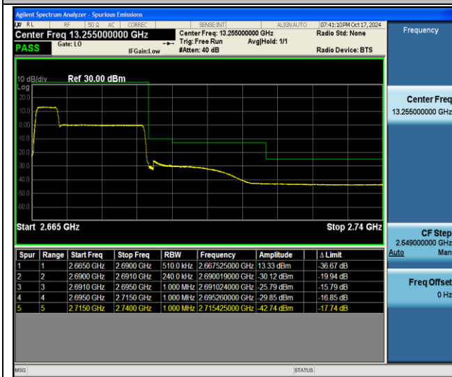
41-41-5MHz-20MHz-QPSK@QPSK-QPSK@QPSK-41373-41490-25RB#0@25RB#0-100RB#0@100RB#0-PASS
