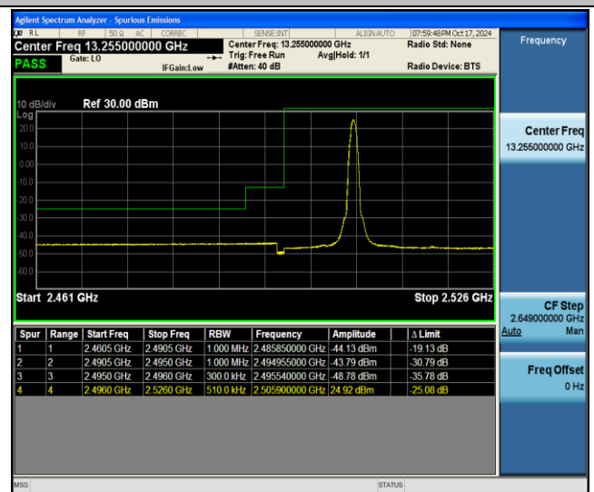
41-41-10MHz-20MHz-QPSK@QPSK-QPSK@QPSK-39705-39849-1RB#49@50RB#0-0RB#0@100RB#0-PASS
