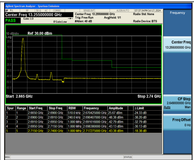
41-41-5MHz-20MHz-QPSK@QPSK-QPSK@QPSK-41373-41490-1RB#24@25RB#0-0RB#0@100RB#0-PASS
