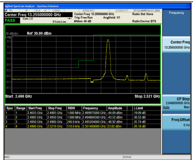
41-41-5MHz-20MHz-16QAM@16QAM-16QAM@16QAM-39683-39800-1RB#24@25RB#0-0RB#0@100RB#0-PASS
