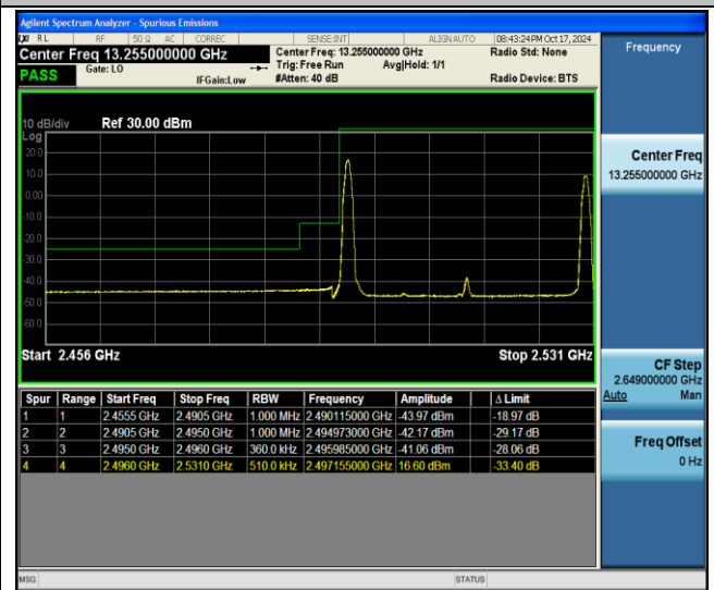
41-41-15MHz-20MHz-QPSK@QPSK-QPSK@QPSK-39728-39899-1RB#0@75RB#0-1RB#99@100RB#0-PASS
