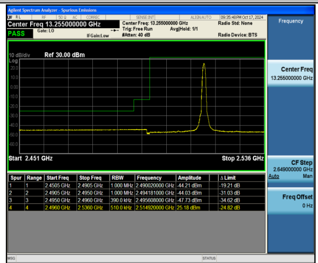
41-41-20MHz-20MHz-QPSK@QPSK-QPSK@QPSK-39750- 39948-1RB#99@100RB#0-0RB#0@100RB#0-PASS
