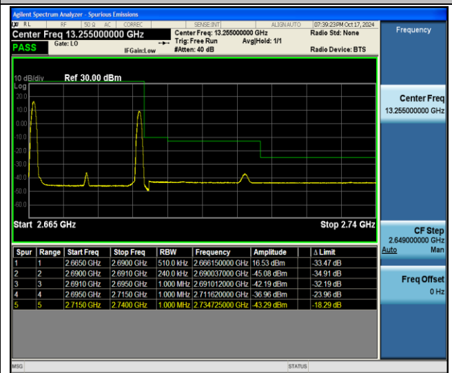
41-41-5MHz-20MHz-QPSK@QPSK-QPSK@QPSK-41373-41490-1RB#0@25RB#0-1RB#99@100RB#0-PASS
