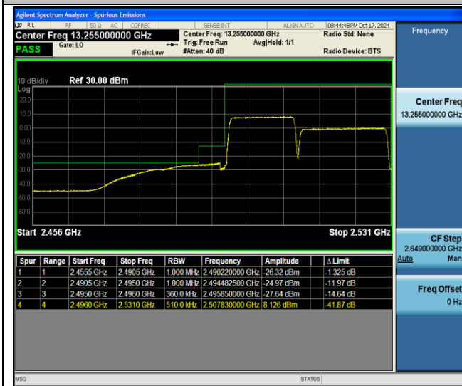
41-41-15MHz-20MHz-QPSK@QPSK-QPSK@QPSK-39728-39899-75RB#0@75RB#0-100RB#0@100RB#0-PASS
