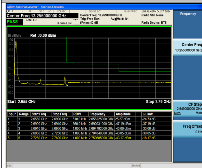
41-41-15MHz-20MHz-QPSK@QPSK-QPSK@QPSK-41319-41490-1RB#0@75RB#0-0RB#0@100RB#0-PASS
