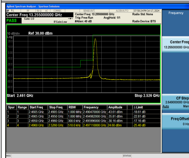
41-41-10MHz-20MHz-QPSK@QPSK-QPSK@QPSK-39705-39849-1RB#0@50RB#0-0RB#0@100RB#0-PASS
