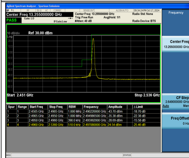
41-41-20MHz-20MHz-QPSK@QPSK-QPSK@QPSK-39750- 39948-1RB#0@100RB#0-0RB#0@100RB#0-PASS
