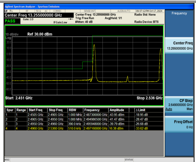
41-41-20MHz-20MHz-QPSK@QPSK-QPSK@QPSK-39750- 39948-1RB#0@100RB#0-1RB#99@100RB#0-PASS
