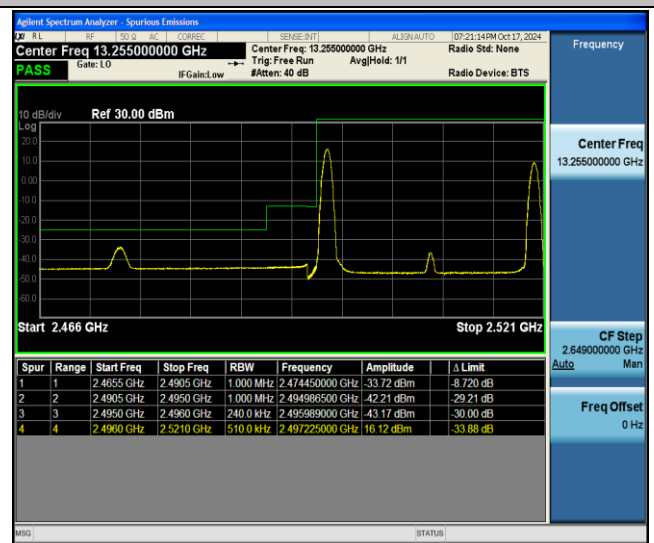
41-41-5MHz-20MHz-256QAM@256QAM-256QAM@256QAM-39683-39800-1RB#0@25RB#0-1RB#99@100RB#0-PASS
