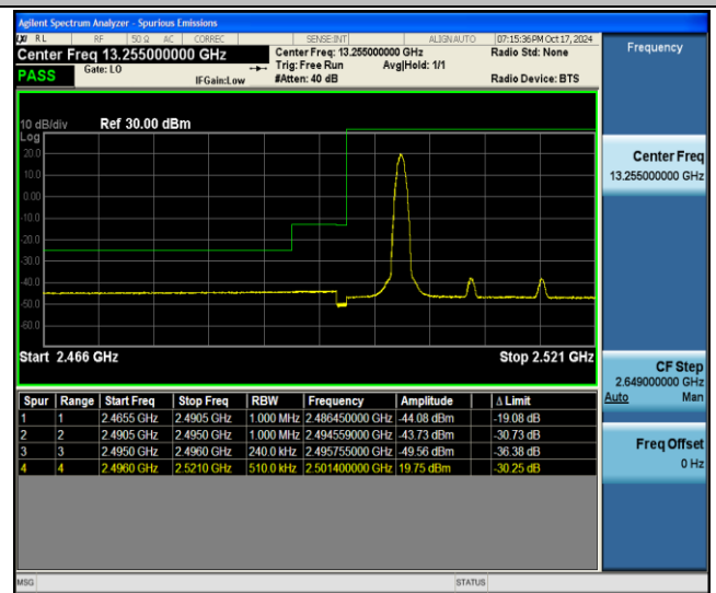
41-41-5MHz-20MHz-256QAM@256QAM-256QAM@256QAM-39683-39800-1RB#24@25RB#0-0RB#0@100RB#0-PASS
