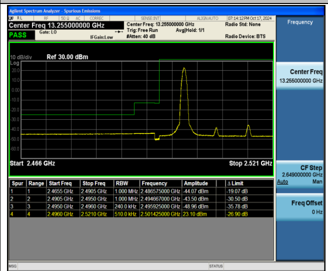
41-41-5MHz-20MHz-64QAM@64QAM-64QAM@64QAM-39683-39800-1RB#24@25RB#0-0RB#0@100RB#0-PASS
