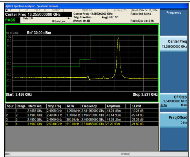
41-41-15MHz-20MHz-QPSK@QPSK-QPSK@QPSK-39728-39899-1RB#74@75RB#0-0RB#0@100RB#0-PASS
