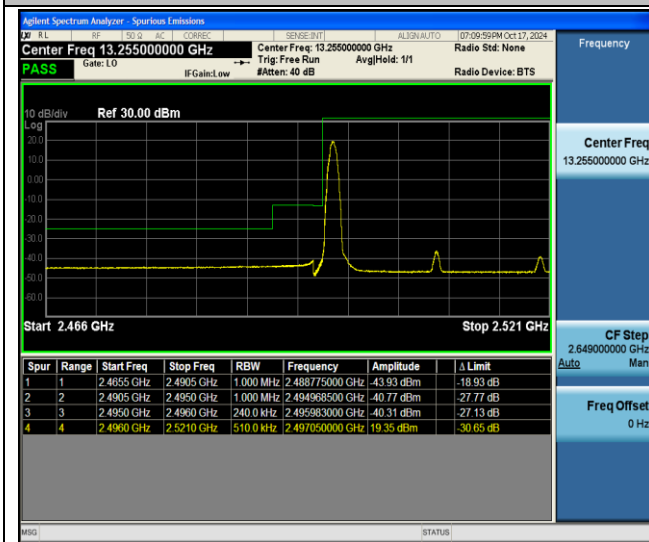
41-41-5MHz-20MHz-256QAM@256QAM-256QAM@256QAM-39683-39800-1RB#0@25RB#0-0RB#0@100RB#0-PASS
