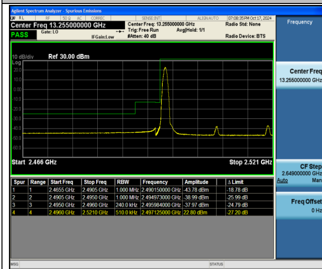
41-41-5MHz-20MHz-64QAM@64QAM-64QAM@64QAM-39683-39800-1RB#0@25RB#0-0RB#0@100RB#0-PASS
