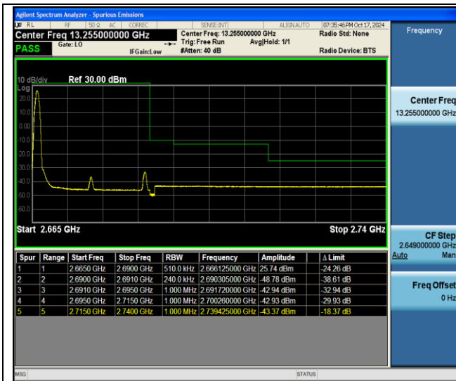
41-41-5MHz-20MHz-QPSK@QPSK-QPSK@QPSK-41373-41490-1RB#0@25RB#0-0RB#0@100RB#0-PASS
