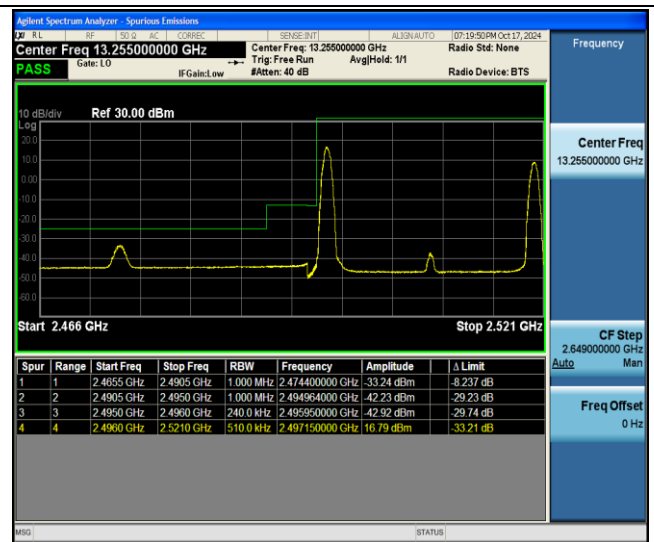
41-41-5MHz-20MHz-64QAM@64QAM-64QAM@64QAM-39683-39800-1RB#0@25RB#0-1RB#99@100RB#0-PASS
