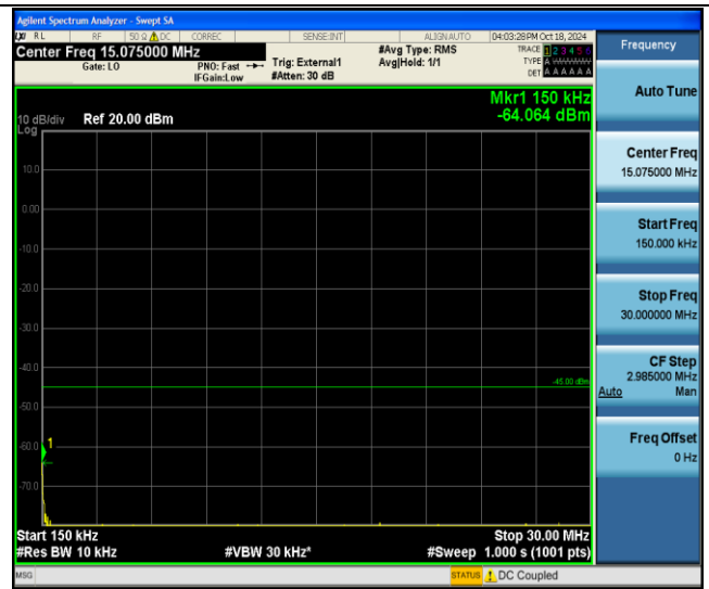
41-41-20MHz-20MHz-QPSK-QPSK-39750-39948-1RB#0-ORB#0-0.15~30MHz-PASS
