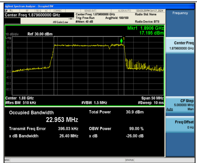
2-2-20MHz-5MHz-64QAM-64QAM-18875-18992-100RB#0- 25RB#0-PASS
