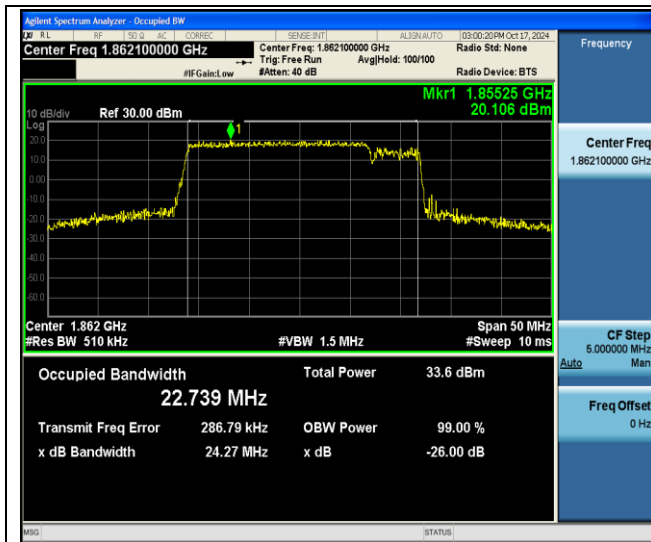
2-2-20MHz-5MHz-64QAM-64QAM-18700-18817-100RB#0- 25RB#0-PASS
