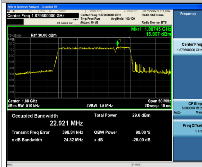
2-2-20MHz-5MHz-256QAM-256QAM-18875-18992-100RB#0- 25RB#0-PASS
