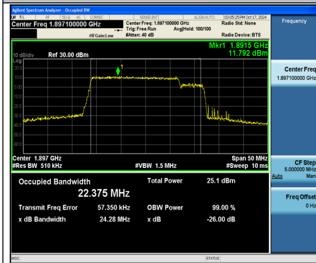
2-2-20MHz-5MHz-64QAM-64QAM-19050-19167-100RB#0- 25RB#0-PASS
