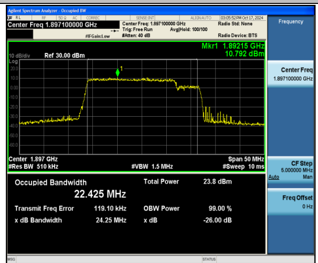
2-2-20MHz-5MHz-256QAM-256QAM-19050-19167-100RB#0- 25RB#0-PASS
