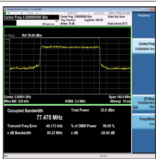
NTNV_N77-3450-3550_PC2_30_80_M_TID6_Ant1#1
