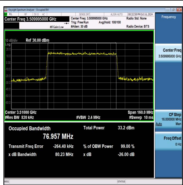
NTNV_N77-3450-3550_PC2_30_80_H_TID4_Ant1#1
