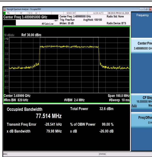
NTNV_N77-3450-3550_PC2_30_80_L_TID8_Ant1#1
