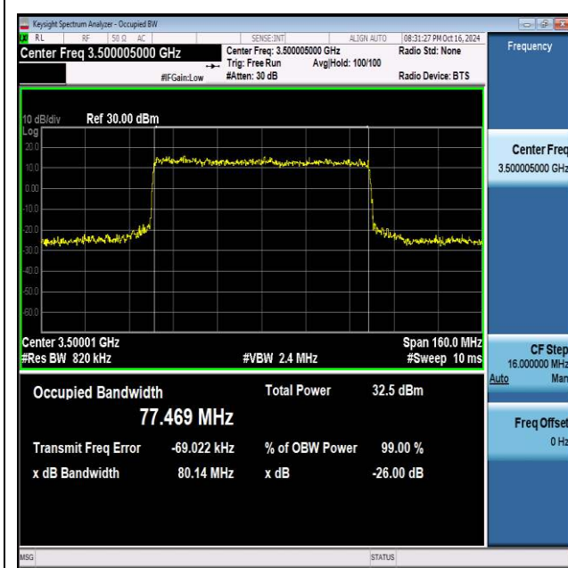
NTNV_N77-3450-3550_PC2_30_80_M_TID7_Ant1#1
