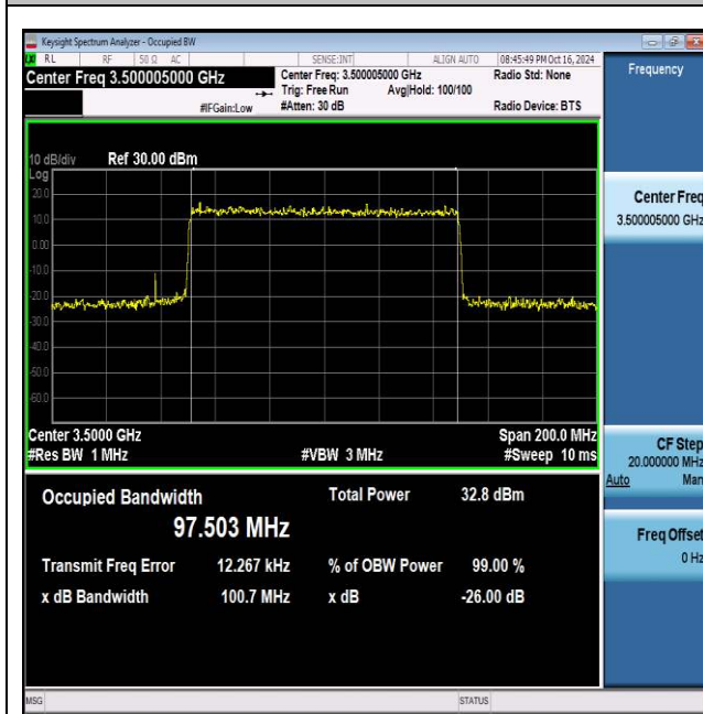
NTNV_N77-3450-3550_PC2_30_100_M_TID7_Ant1#1
