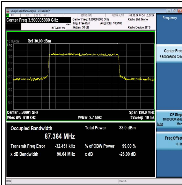
NTVN_N77-3450-3550_PC2_30_90_M_TID5_Ant1#1
