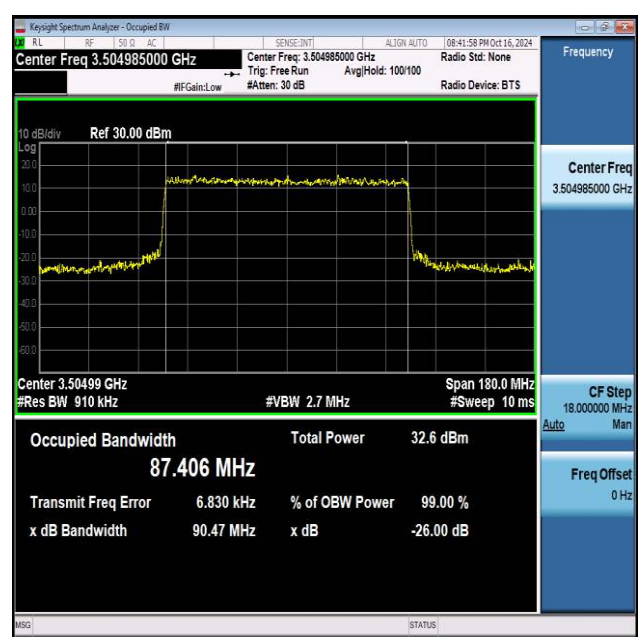
NTNV_N77-3450-3550_PC2_30_90_H_TID8_Ant1#1
