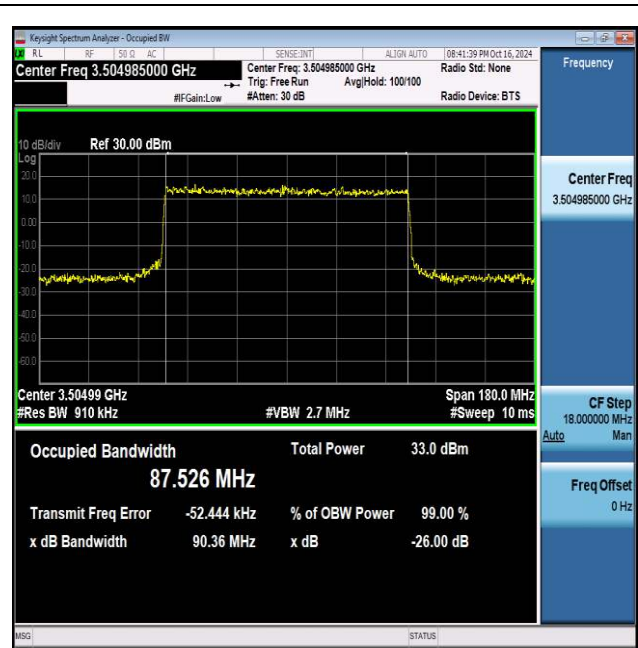
NTNV_N77-3450-3550_PC2_30_90_H_TID6_Ant1#1
