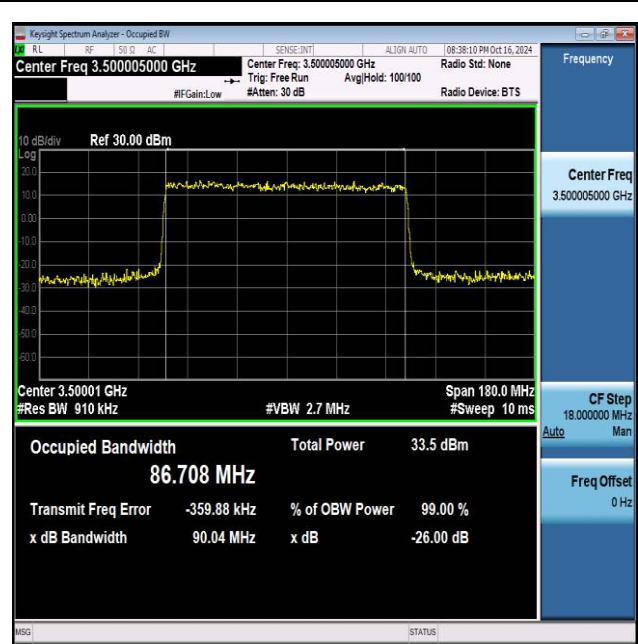
NTNV_N77-3450-3550_PC2_30_90_M_TID4_Ant1#1
