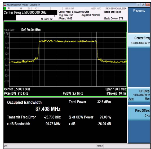
NTVN_N77-3450-3550_PC2_30_90_M_TID8_Ant1#1
