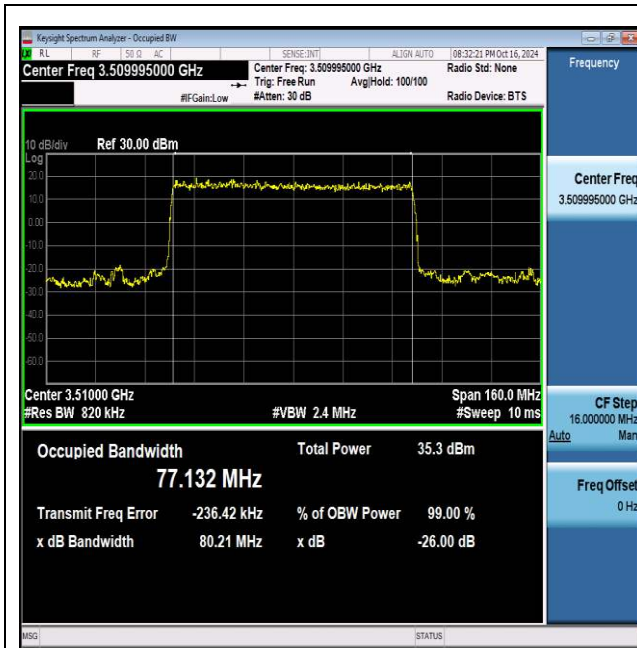
NTNV_N77-3450-3550_PC2_30_80_H_TID1_Ant1#1
