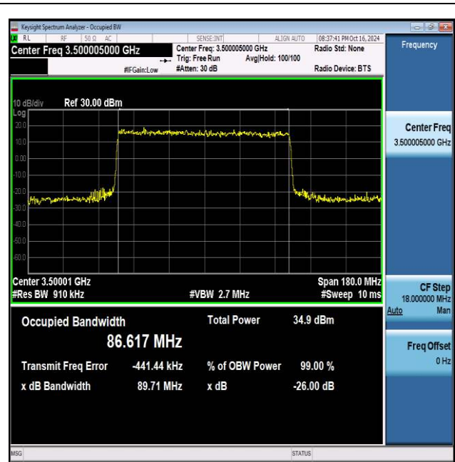
NTNV_N77-3450-3550_PC2_30_90_M_TID2_Ant1#1
