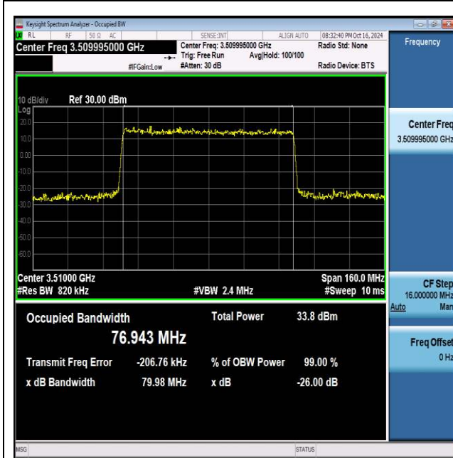
NTNV_N77-3450-3550_PC2_30_80_H_TID3_Ant1#1
