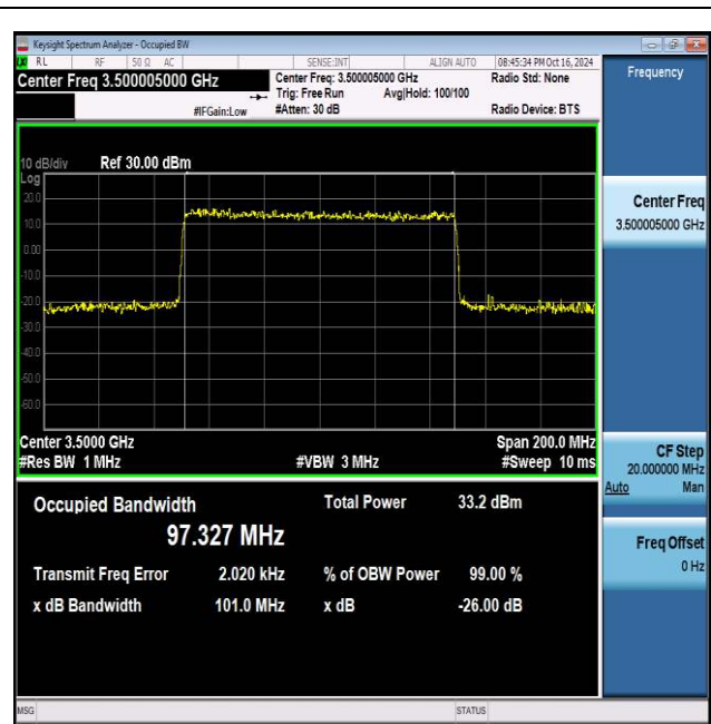
NTNV_N77-3450-3550_PC2_30_100_M_TID6_Ant1#1
