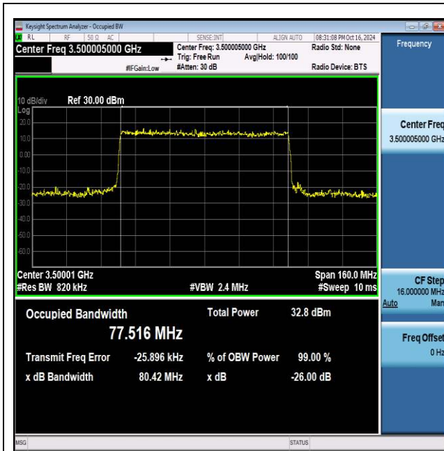
NTNV_N77-3450-3550_PC2_30_80_M_TID5_Ant1#1
