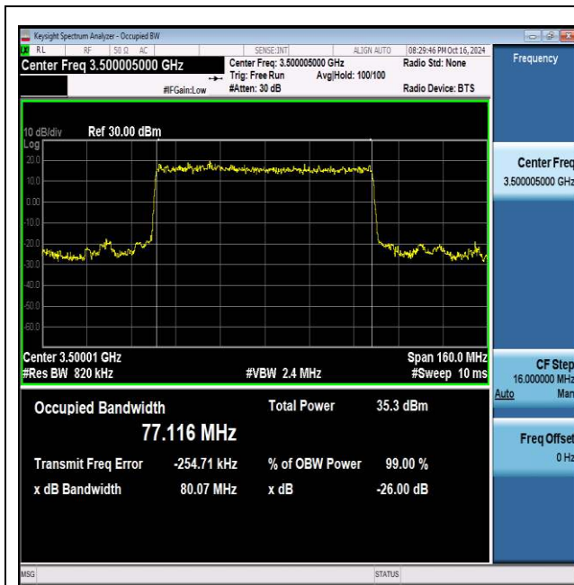
NTNV_N77-3450-3550_PC2_30_80_M_TID1_Ant1#1
