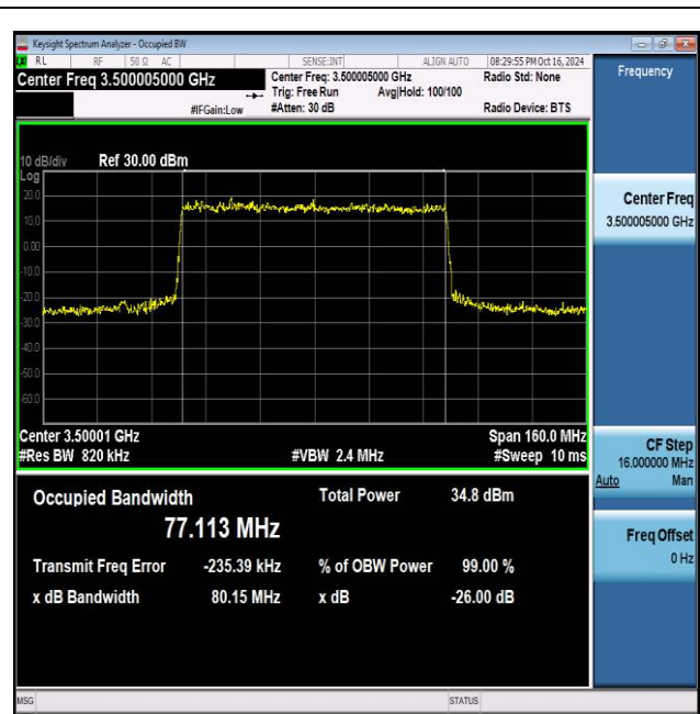
NTNV_N77-3450-3550_PC2_30_80_M_TID2_Ant1#1
