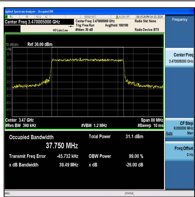
NTNV_N77-3450-3550_PC2_30_40_L_TID8_Ant1#1
