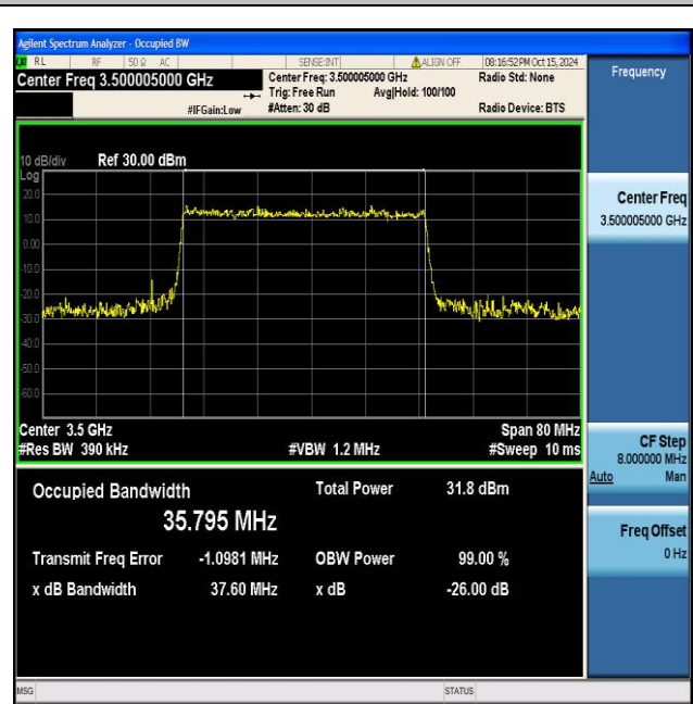
NTNV_N77-3450-3550_PC2_30_40_M_TID2_Ant1#1
