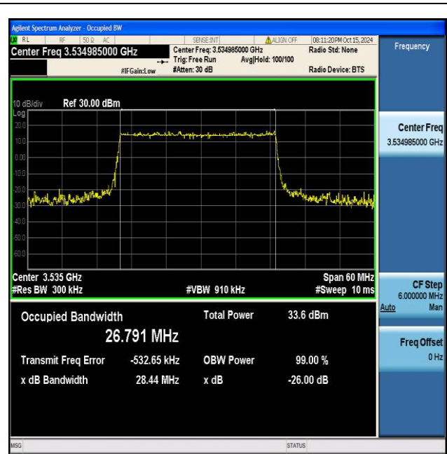
NTNV_N77-3450-3550_PC2_30_30_H_TID2_Ant1#1
