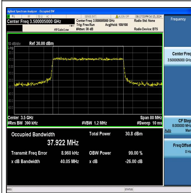
NTNV_N77-3450-3550_PC2_30_40_M_TID7_Ant1#1
