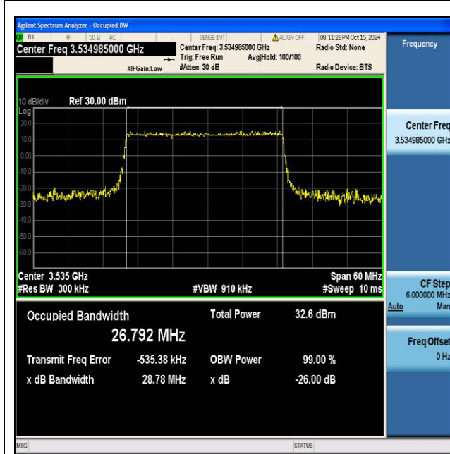
NTNV_N77-3450-3550_PC2_30_30_H_TID3_Ant1#1
