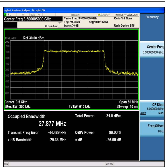
NTNV_N77-3450-3550_PC2_30_30_M_TID6_Ant1#1
