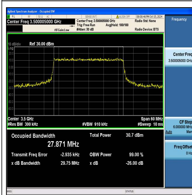
NTNV_N77-3450-3550_PC2_30_30_M_TID7_Ant1#1
