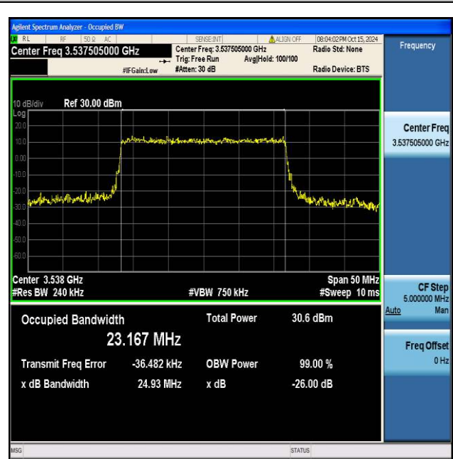
NTNV_N77-3450-3550_PC2_30_25_H_TID8_Ant1#1
