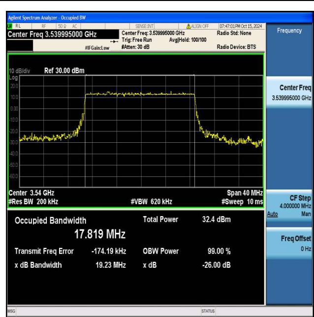
NTNV_N77-3450-3550_PC2_30_20_H_TID4_Ant1#1
