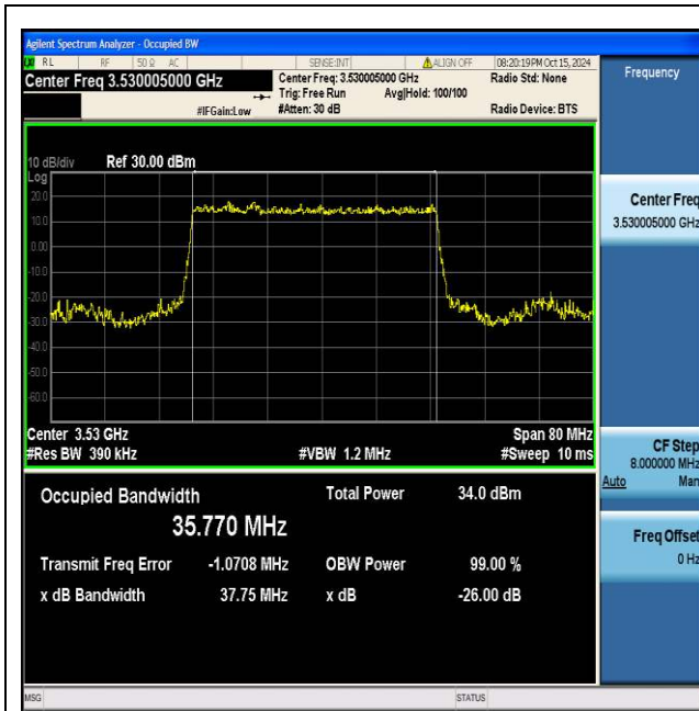
NTNV_N77-3450-3550_PC2_30_40_H_TID1_Ant1#1
