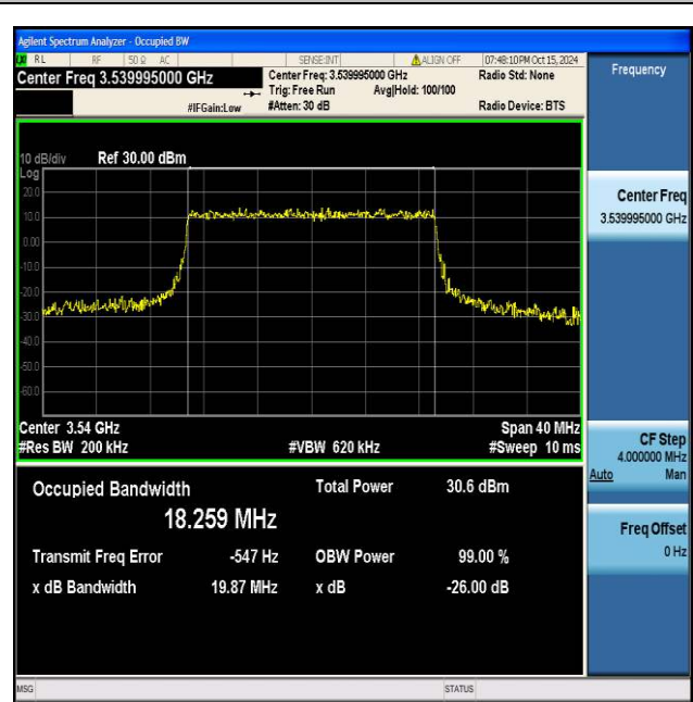
NTNV_N77-3450-3550_PC2_30_20_H_TID8_Ant1#1
