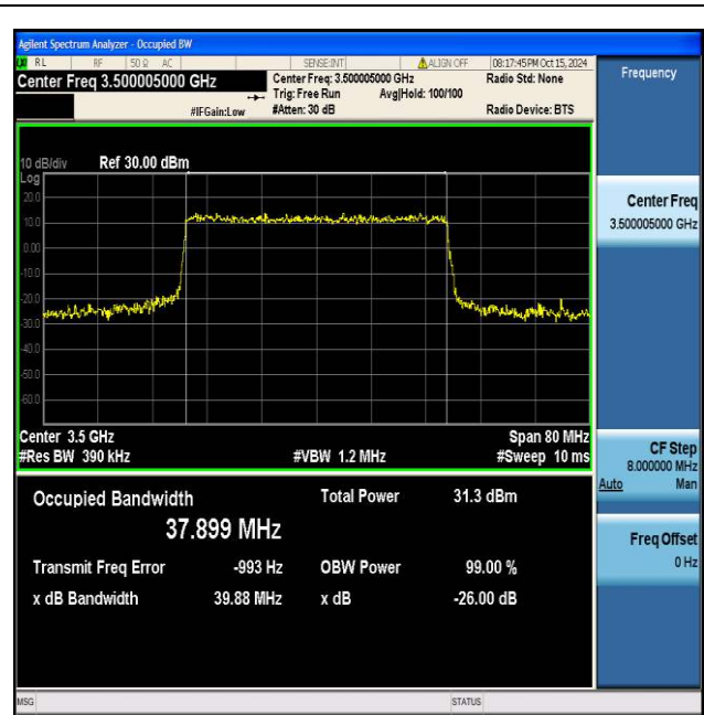
NTNV_N77-3450-3550_PC2_30_40_M_TID6_Ant1#1
