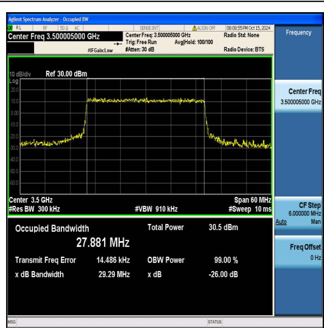
NTNV_N77-3450-3550_PC2_30_30_M_TID8_Ant1#1
