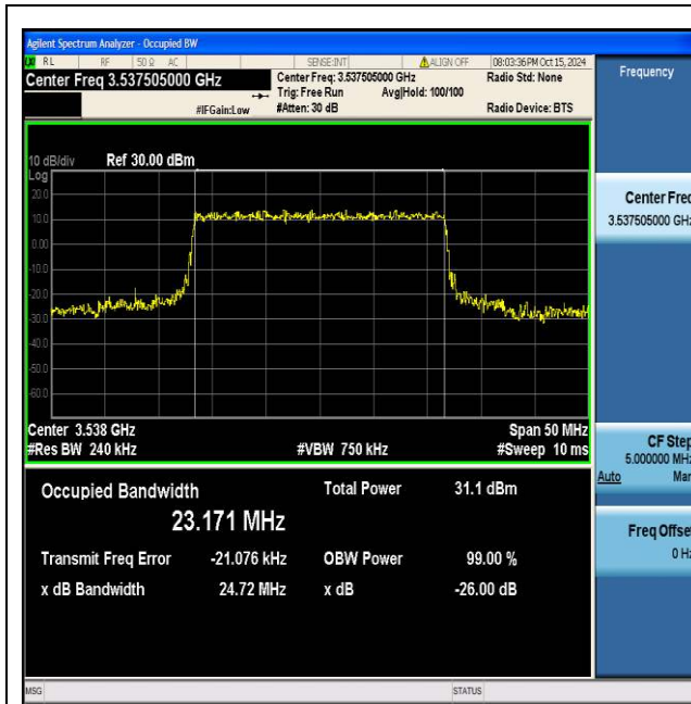
NTNV_N77-3450-3550_PC2_30_25_H_TID5_Ant1#1
