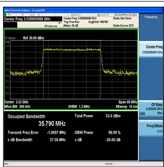
NTNV_N77-3450-3550_PC2_30_40_H_TID2_Ant1#1
