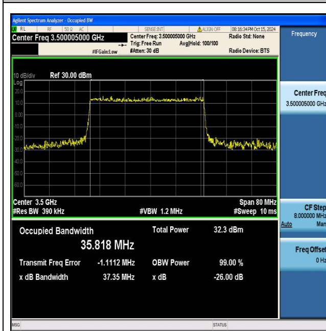
NTNV_N77-3450-3550_PC2_30_40_M_TID1_Ant1#1
