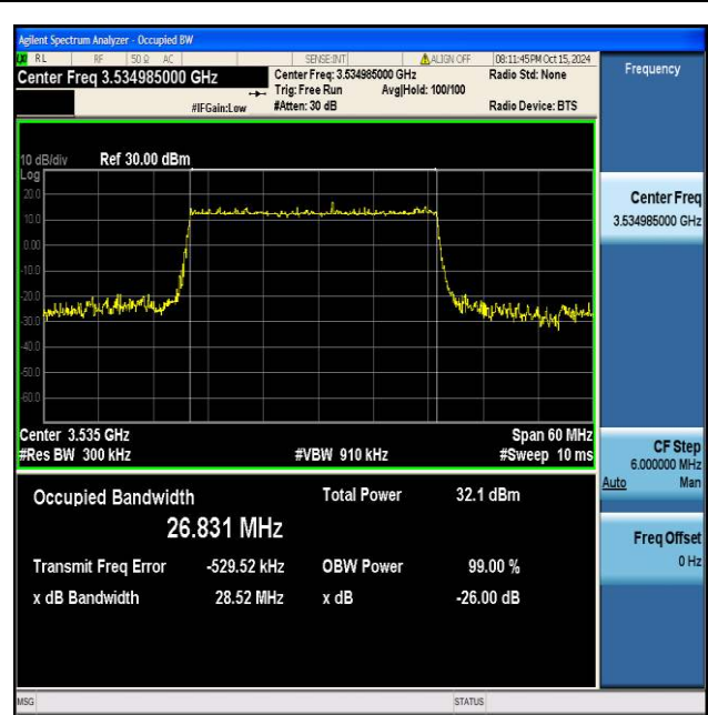
NTNV_N77-3450-3550_PC2_30_30_H_TID4_Ant1#1
