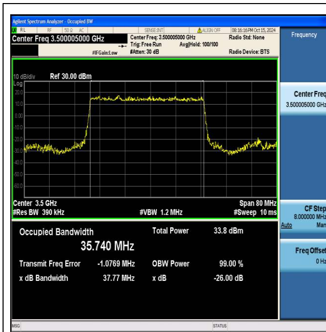
NTNV_N77-3450-3550_PC2_30_40_M_TID1_Ant1#1
