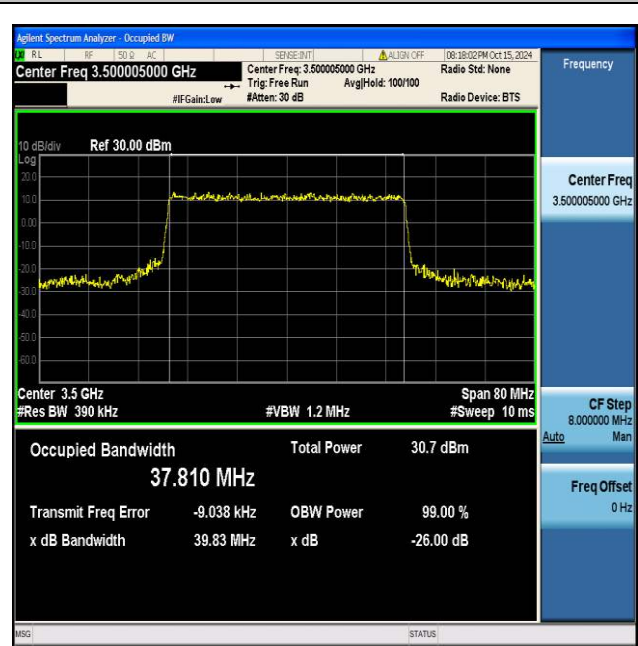
NTNV_N77-3450-3550_PC2_30_40_M_TID8_Ant1#1
