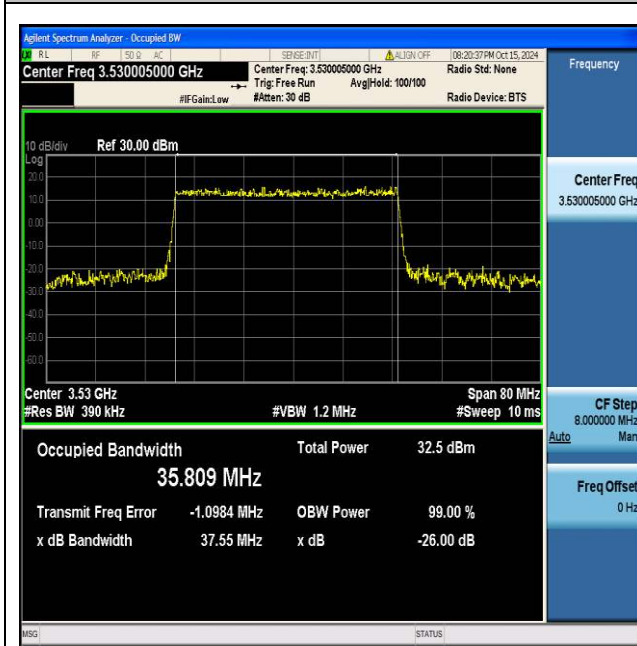
NTNV_N77-3450-3550_PC2_30_40_H_TID3_Ant1#1
