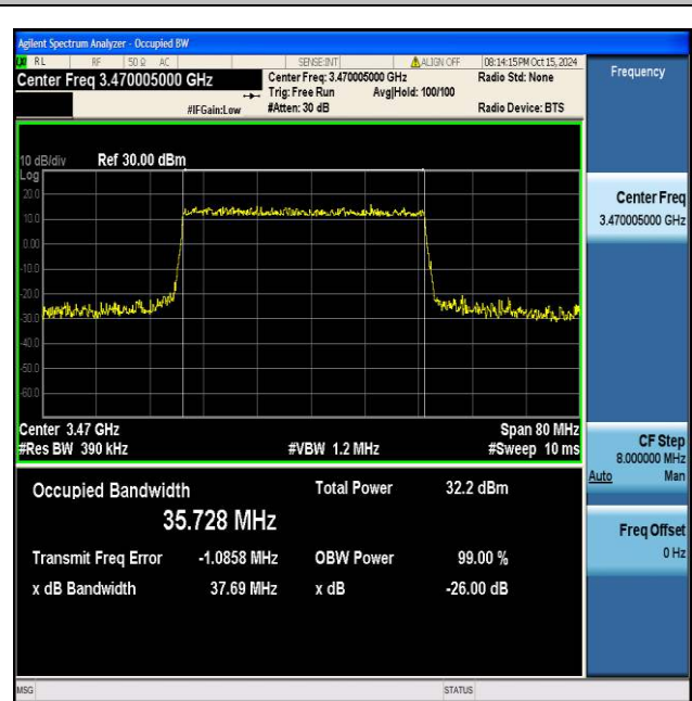
NTNV_N77-3450-3550_PC2_30_40_L_TID4_Ant1#1
