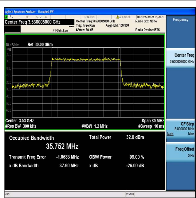
NTNV_N77-3450-3550_PC2_30_40_H_TID4_Ant1#1
