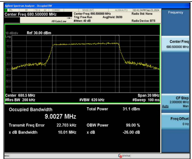
Band71-10MHz-64QAM-133297-50RB#0-PASS
