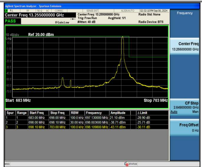
Band71-15MHz-QPSK-133397-1RB#74-PASS
