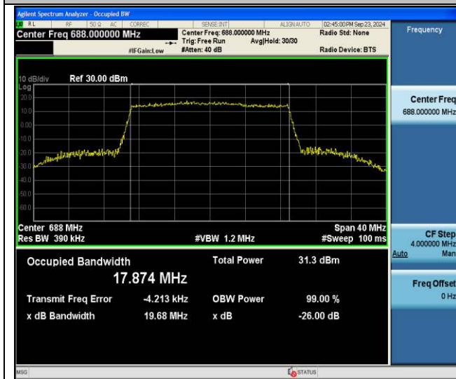
Band71-20MHz-64QAM-133372-100RB#0-PASS
