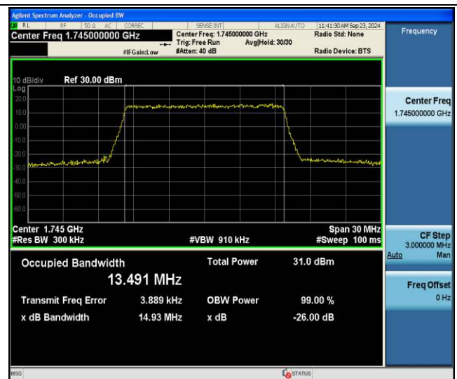
Band66-15MHz-64QAM-132322-75RB#0-PASS
