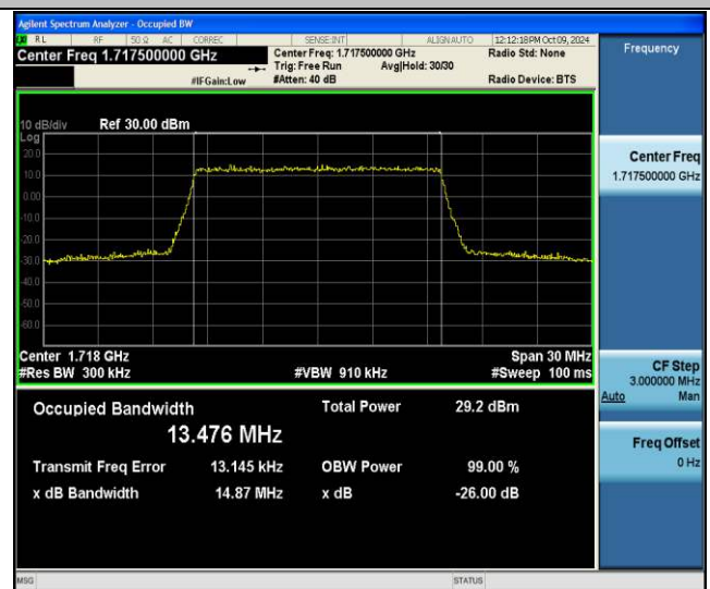
Band66-15MHz-256QAM-132047-75RB#0-PASS
