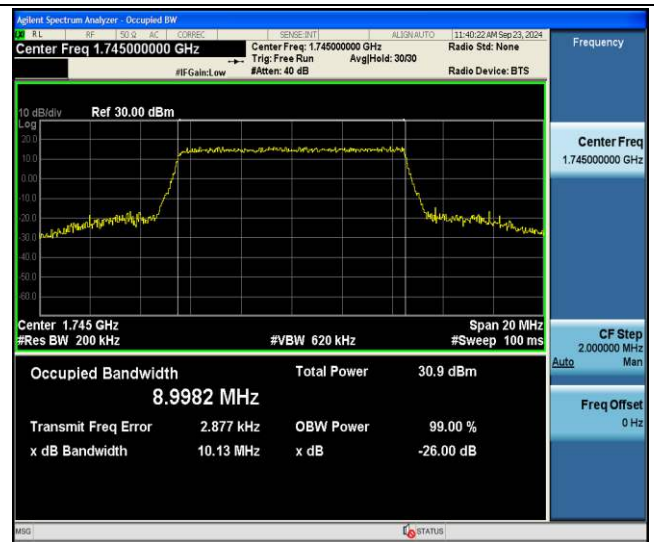
Band66-10MHz-64QAM-132322-50RB#0-PASS
