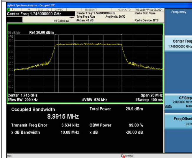
Band66-10MHz-16QAM-132322-50RB#0-PASS
