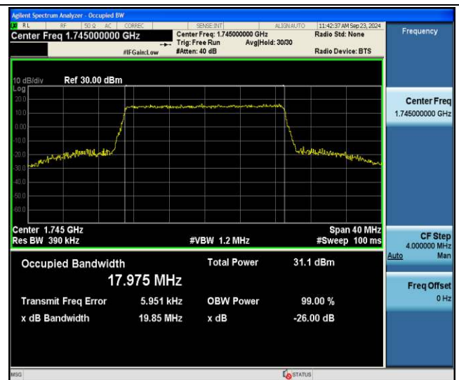
Band66-20MHz-64QAM-132322-100RB#0-PASS
