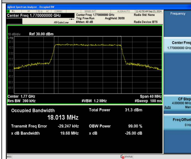
Band66-20MHz-64QAM-132572-100RB#0-PASS
