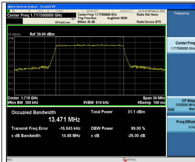
Band66-15MHz-64QAM-132047-75RB#0-PASS
