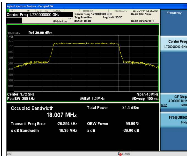
Band66-20MHz-64QAM-132072-100RB#0-PASS
