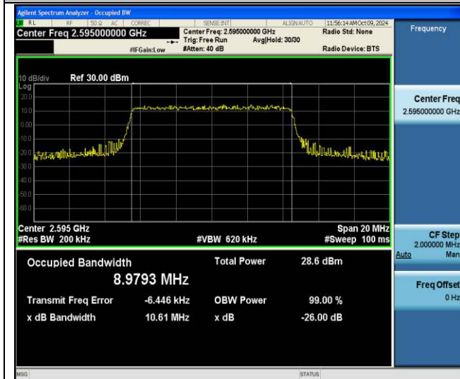
Band38-10MHz-256QAM-38000-50RB#0-PASS
