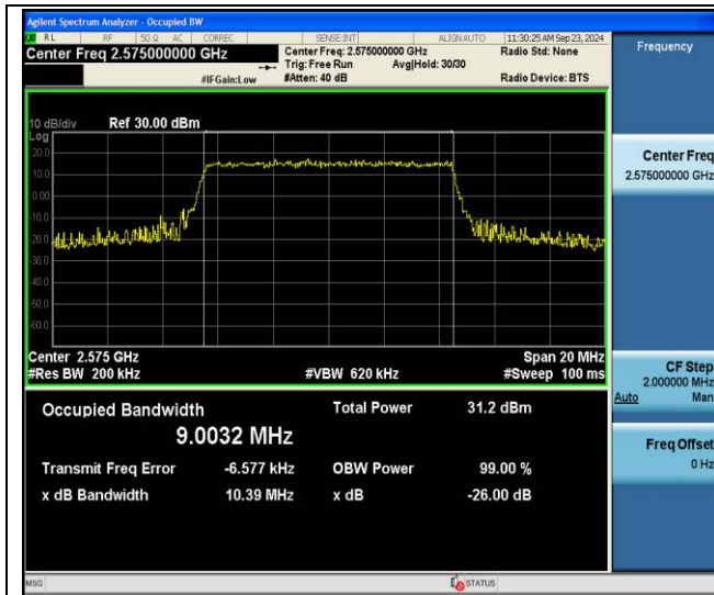
Band38-10MHz-64QAM-37800-50RB#0-PASS
