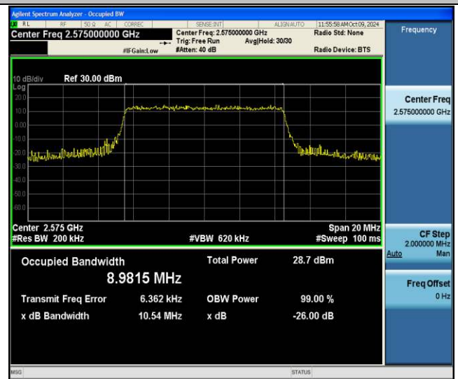
Band38-10MHz-256QAM-37800-50RB#0-PASS
