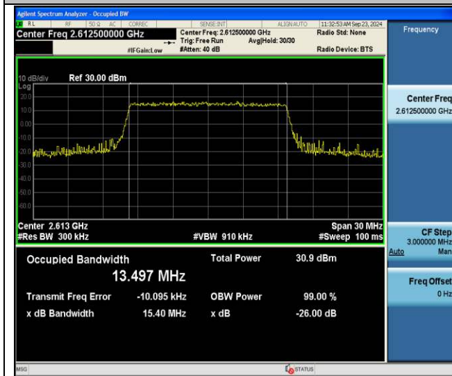
Band38-15MHz-64QAM-38175-75RB#0-PASS
