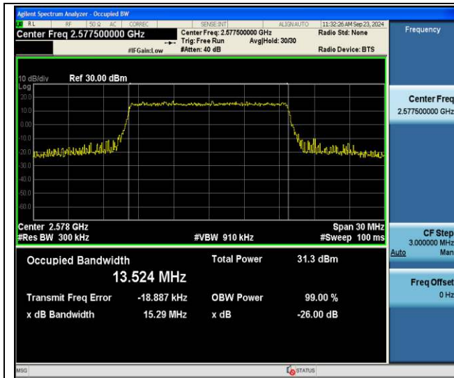
Band38-15MHz-64QAM-37825-75RB#0-PASS
