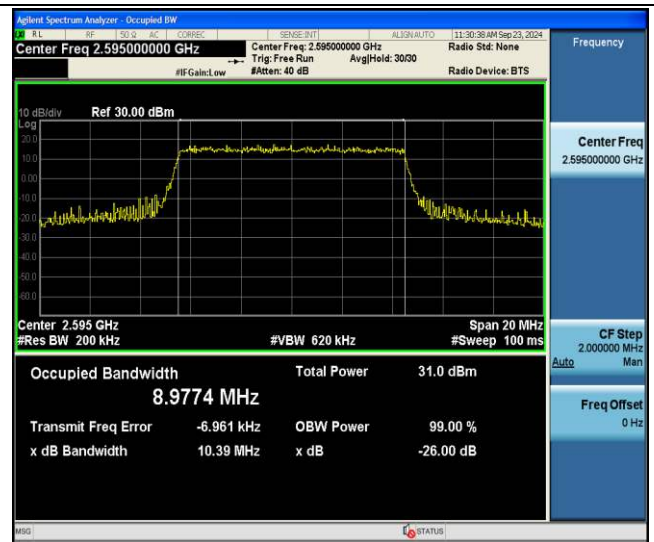
Band38-10MHz-64QAM-38000-50RB#0-PASS
