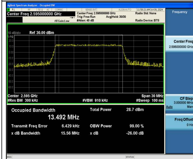
Band38-15MHz-256QAM-38000-75RB#0-PASS
