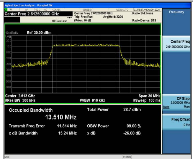
Band38-15MHz-256QAM-38175-75RB#0-PASS
