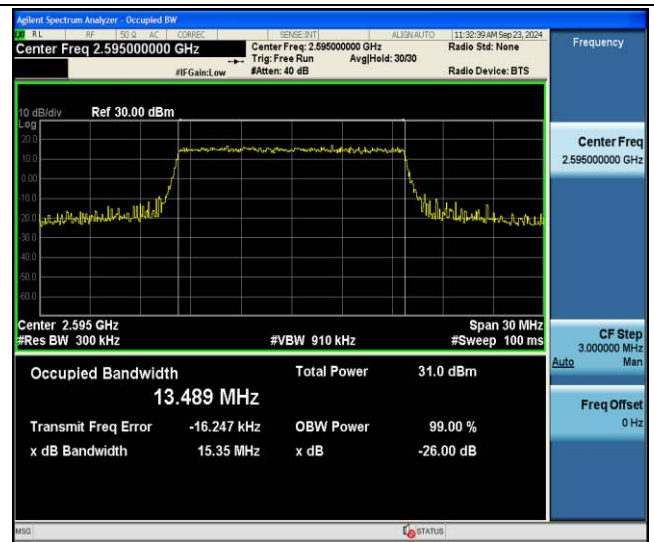
Band38-15MHz-64QAM-38000-75RB#0-PASS
