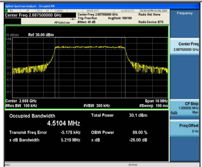
Band41-5MHz-256QAM-41565-25RB#0-PASS
