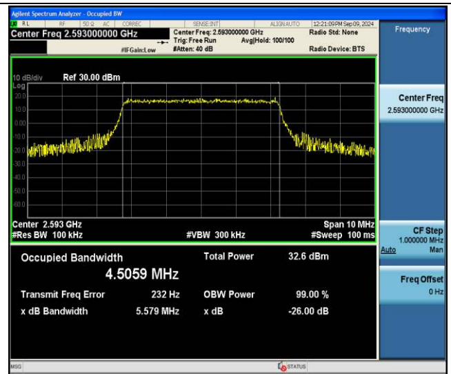
Band41-5MHz-64QAM-40620-25RB#0-PASS
