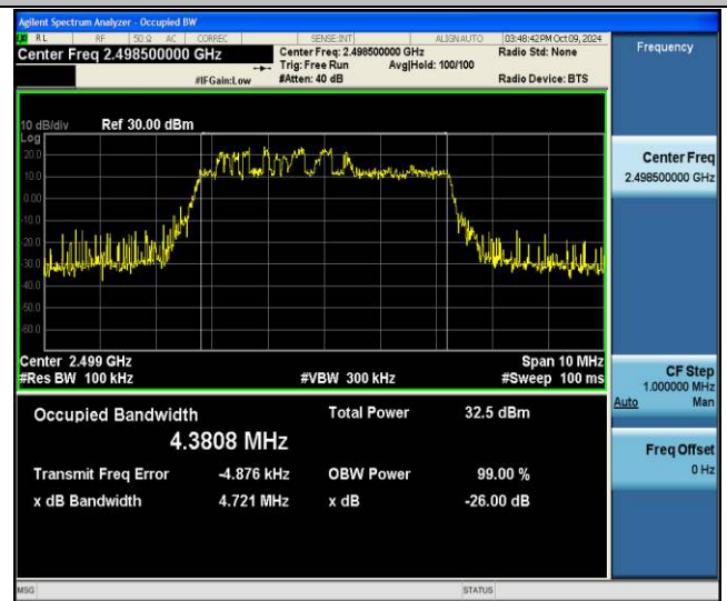
Band41-5MHz-256QAM-39675-25RB#0-PASS
