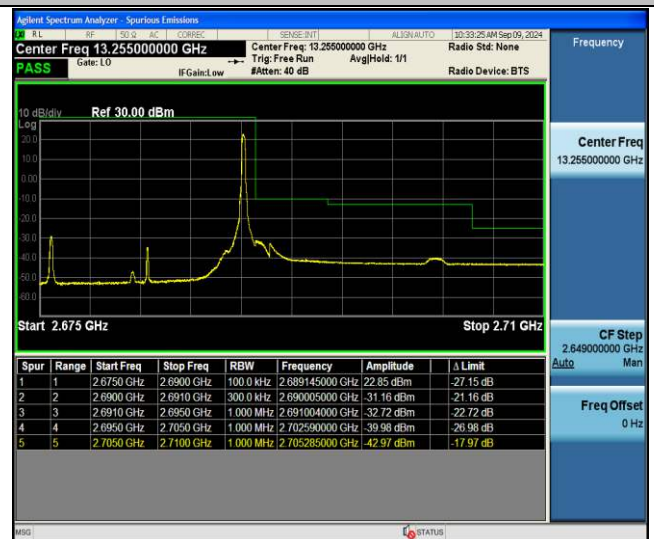
Band41-15MHz-QPSK-41515-1RB#74-PASS
