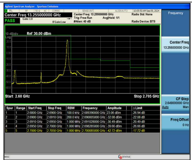
Band41-10MHz-QPSK-41540-1RB#49-PASS
