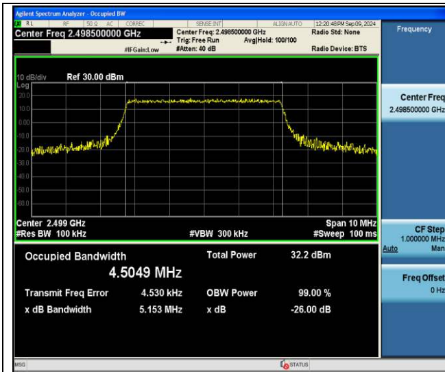
Band41-5MHz-64QAM-39675-25RB#0-PASS
