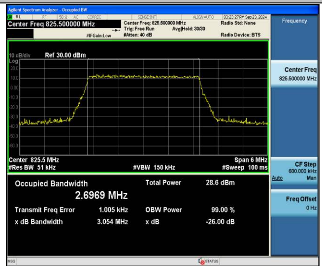
Band26(824-849)-3MHz-256QAM-26805-15RB#0-PASS
