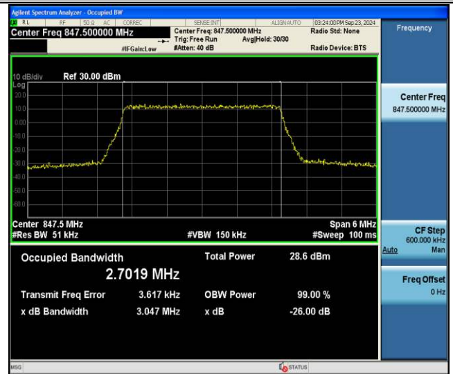
Band26(824-849)-3MHz-256QAM-27025-15RB#0-PASS
