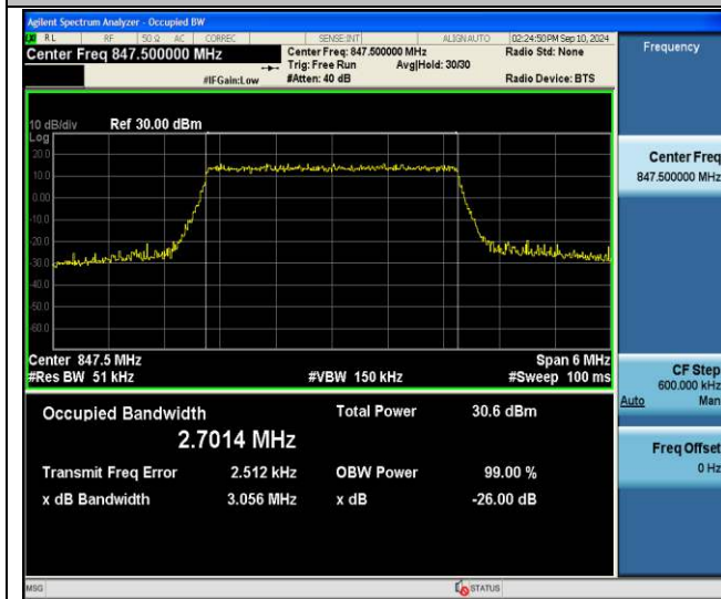
Band26(824-849)-3MHz-64QAM-27025-15RB#0-PASS
