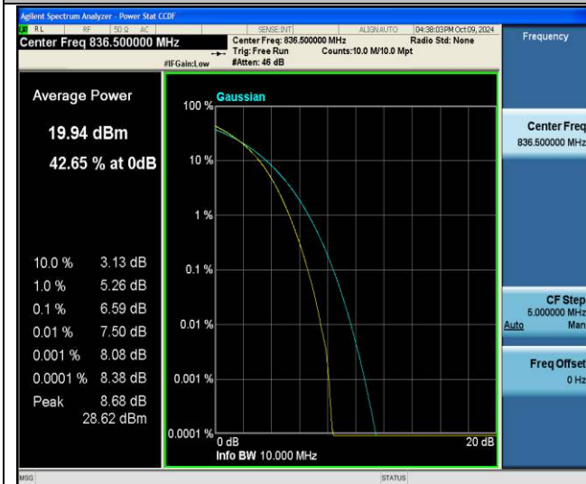
Band26(824-849)-15MHz-256QAM-26915-75RB#0-PASS
