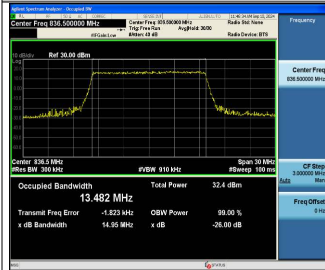
Band26(824-849)-15MHz-16QAM-26915-75RB#0-PASS
