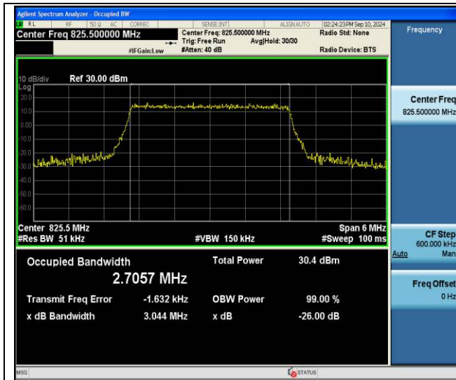
Band26(824-849)-3MHz-64QAM-26805-15RB#0-PASS
