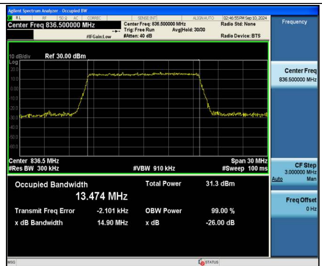
Band26(824-849)-15MHz-64QAM-26915-75RB#0-PASS
