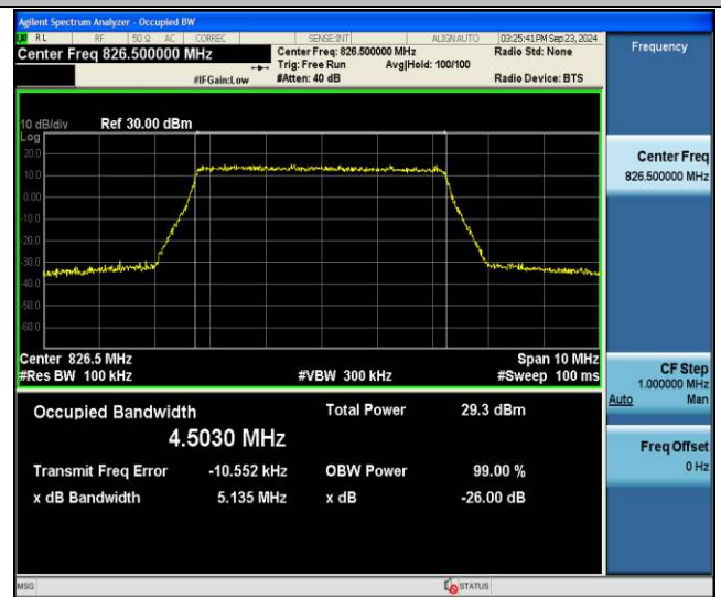
Band26(824-849)-5MHz-256QAM-26815-25RB#0-PASS
