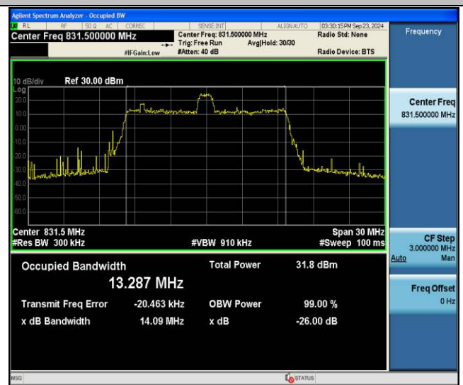
Band26(824-849)-15MHz-256QAM-26865-75RB#0-PASS
