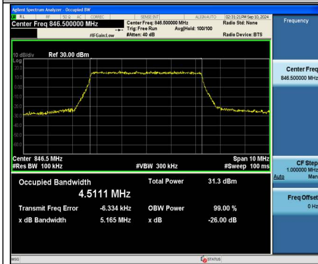
Band26(824-849)-5MHz-64QAM-27015-25RB#0-PASS
