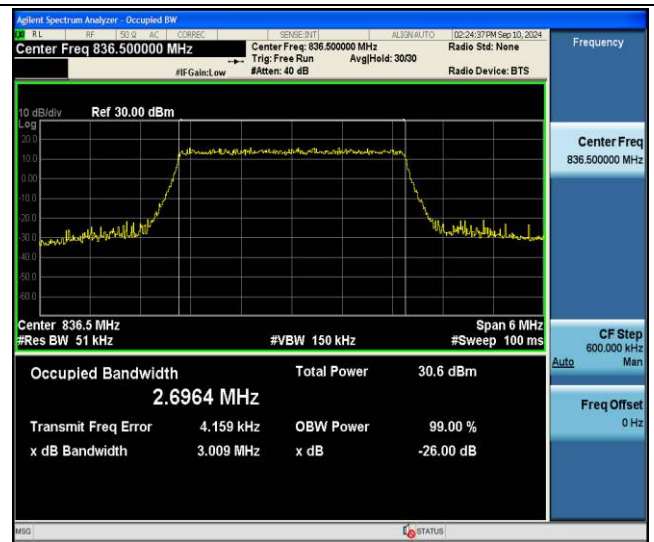
Band26(824-849)-3MHz-64QAM-26915-15RB#0-PASS
