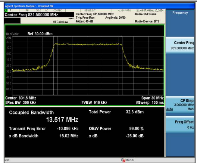
Band26(824-849)-15MHz-16QAM-26865-75RB#0-PASS
