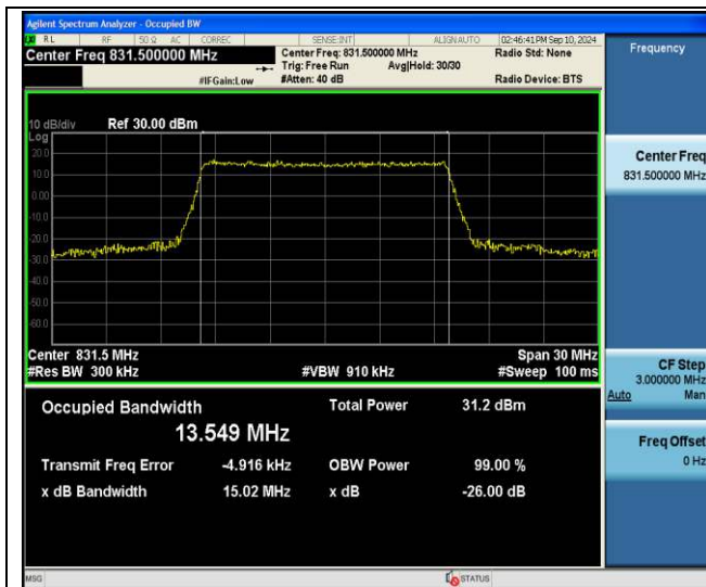
Band26(824-849)-15MHz-64QAM-26865-75RB#0-PASS
