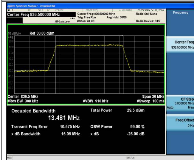
Band26(824-849)-15MHz-256QAM-26915-75RB#0-PASS
