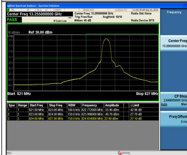
Band26(824-849)-15MHz-QPSK-26865-1RB#0-PASS
