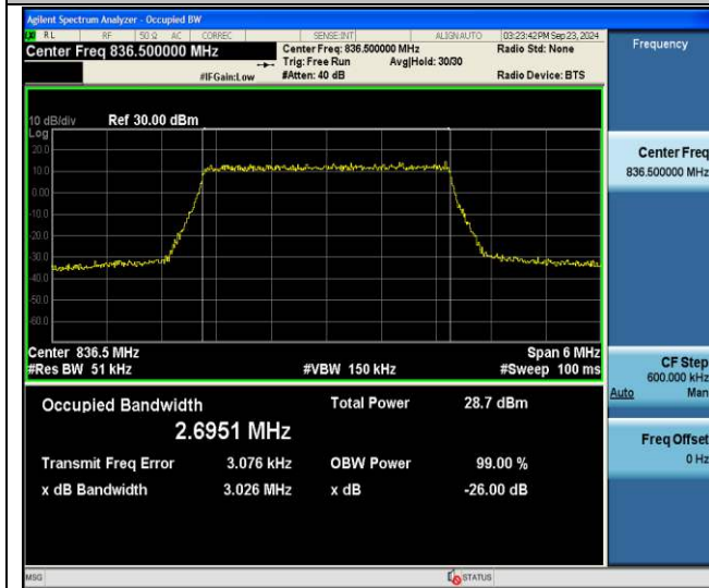
Band26(824-849)-3MHz-256QAM-26915-15RB#0-PASS
