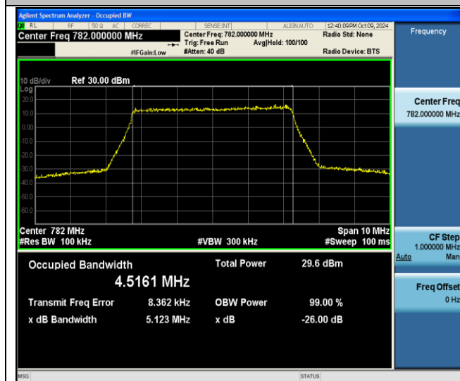
Band13-5MHz-256QAM-23230-25RB#0-PASS
