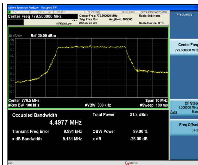
Band13-5MHz-64QAM-23205-25RB#0-PASS
