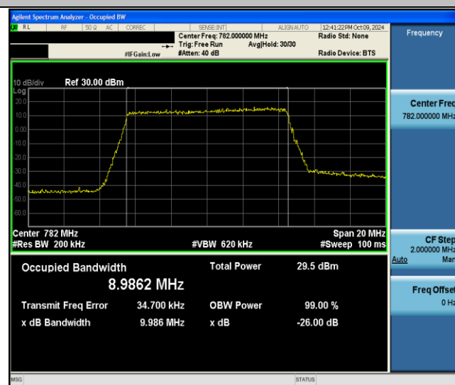
Band13-10MHz-256QAM-23230-50RB#0-PASS
