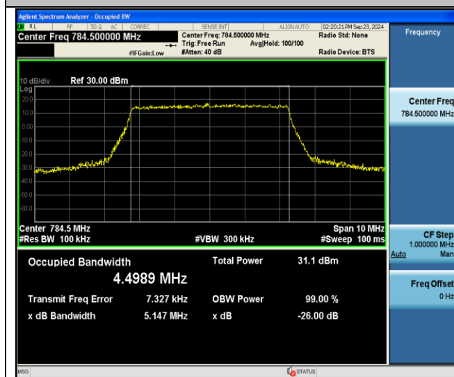
Band13-5MHz-64QAM-23255-25RB#0-PASS
