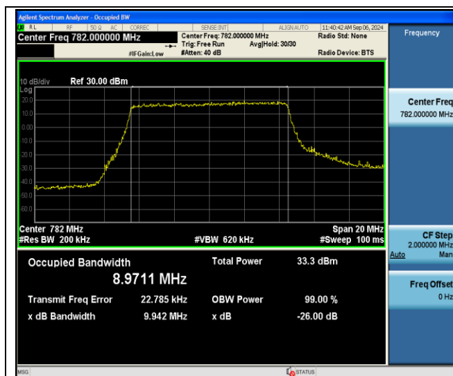
Band13-10MHz-QPSK-23230-50RB#0-PASS
