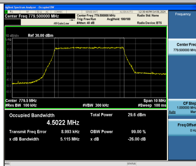
Band13-5MHz-256QAM-23205-25RB#0-PASS
