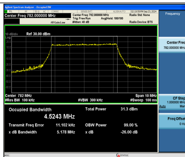
Band13-5MHz-64QAM-23230-25RB#0-PASS
