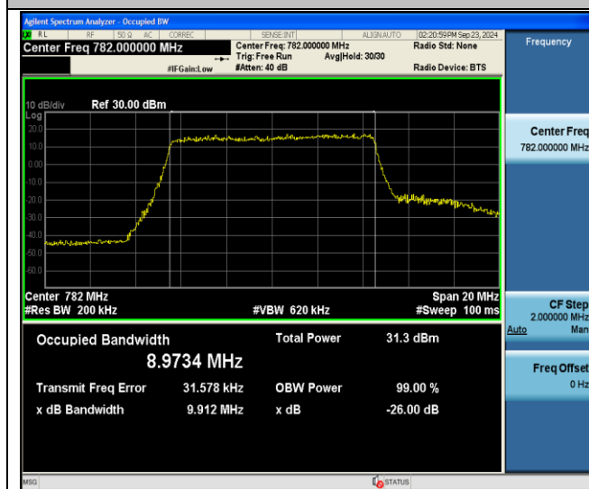
Band13-10MHz-64QAM-23230-50RB#0-PASS
