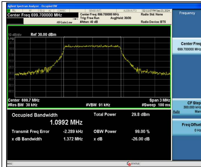
Band12-1.4MHz-64QAM-23017-6RB#0-PASS
