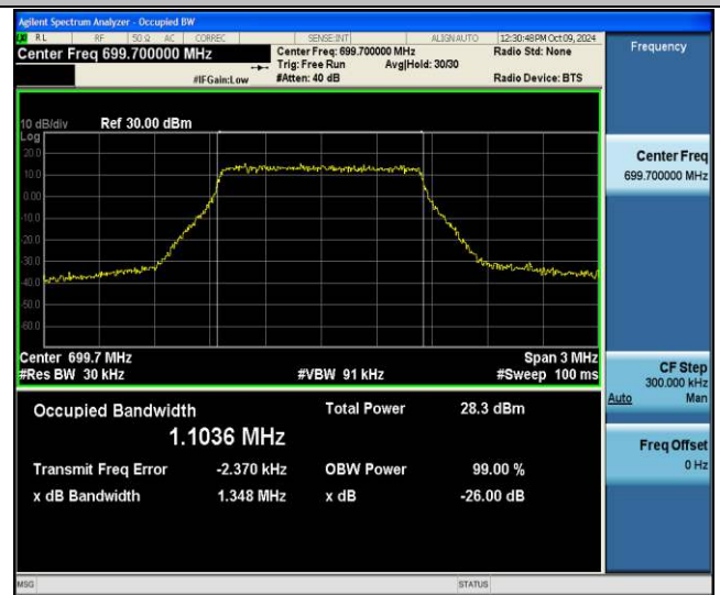
Band12-1.4MHz-256QAM-23017-6RB#0-PASS
