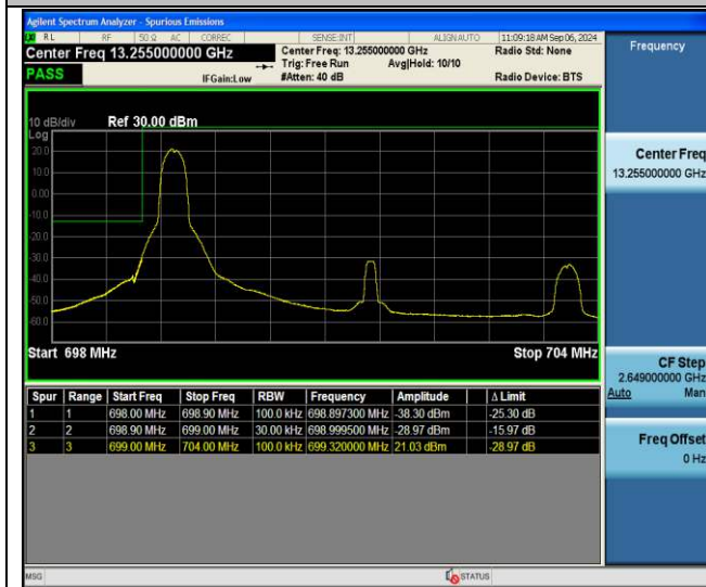
Band12-5MHz-QPSK-23035-1RB#0-PASS
