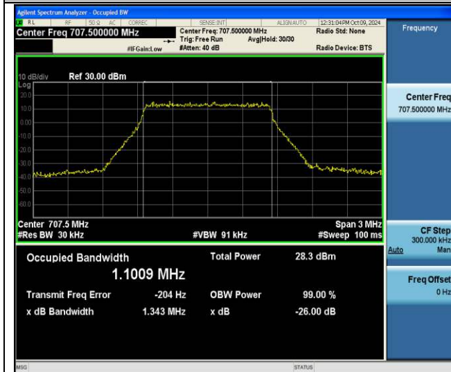
Band12-1.4MHz-256QAM-23095-6RB#0-PASS
