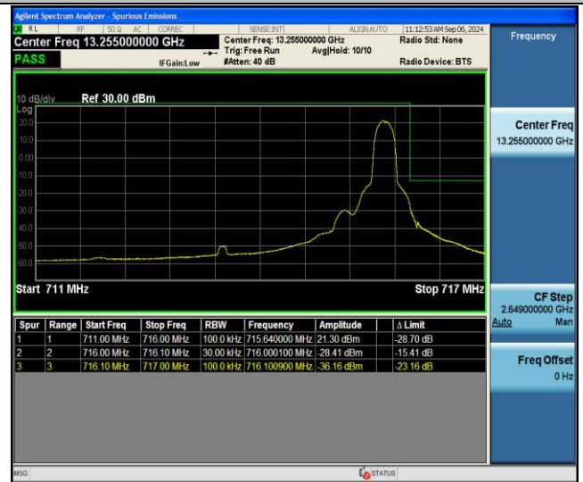
Band12-5MHz-QPSK-23155-1RB#24-PASS
