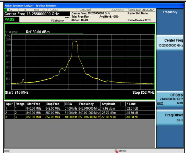
Band5-5MHz-QPSK-20625-1RB#24-PASS
