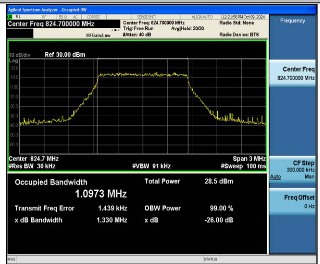
Band5-1.4MHz-256QAM-20407-6RB#0-PASS
