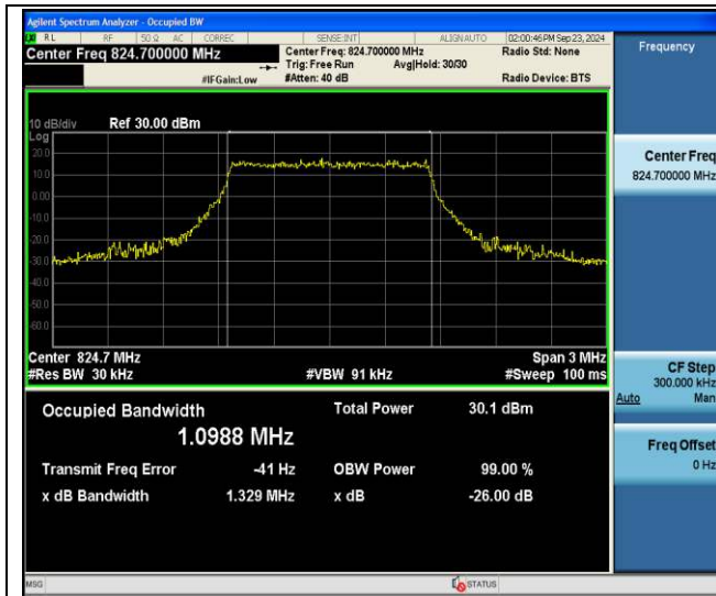
Band5-1.4MHz-64QAM-20407-6RB#0-PASS
