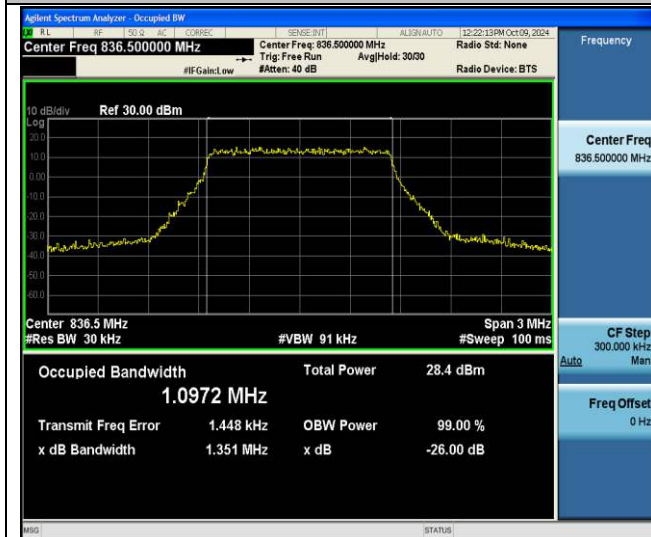
Band5-1.4MHz-256QAM-20525-6RB#0-PASS
