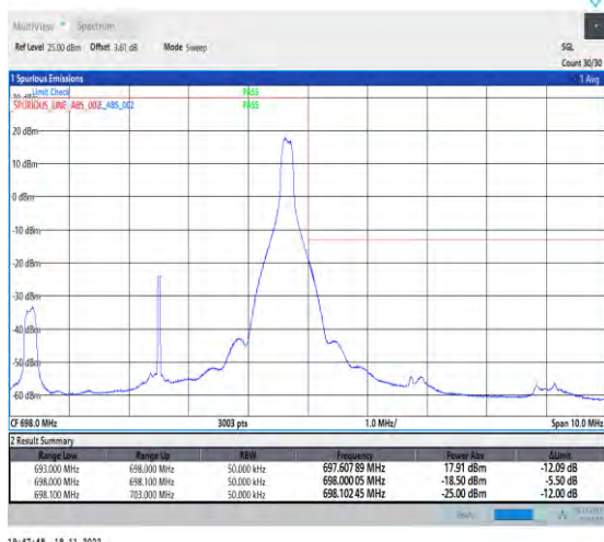
1-N71-PC3-15-5-H-2-DFT-PI2BPSK-Edge_1RB_Right-1@24-Ant1-1--PASS-see graph
