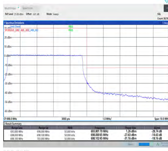
1-N71-PC3-15-5-H-6-CP-QPSK-Outer_Full-25@0-Ant1-1--PASS-see graph
