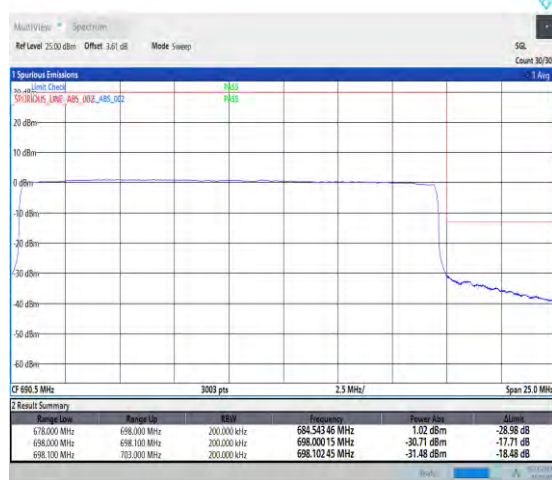
1-N71-PC3-15-20-H-6-CP-QPSK-Outer_Full-106@0-Ant1-1--PASS-see graph
