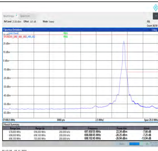
1-N71-PC3-15-20-H-2-DFT-PI2BPSK-Edge_1RB_Right-t-1@105-Ant1-1--PASS-see graph
