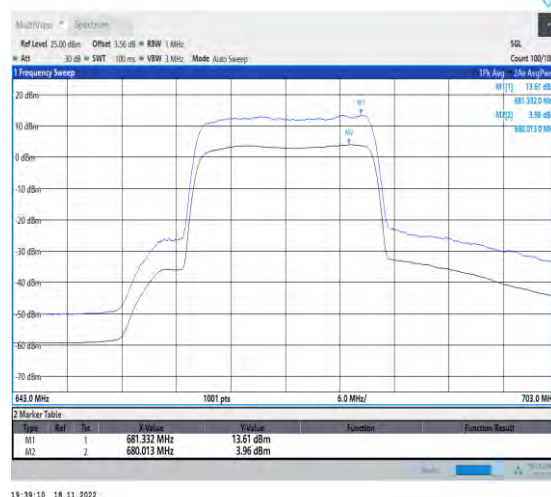
1-N71-PC3-15-20-L-2-CP-256QAM-Outer_Full-106 @0-Ant1-9.65-100%-0.00-9.65-PASS-≤13
