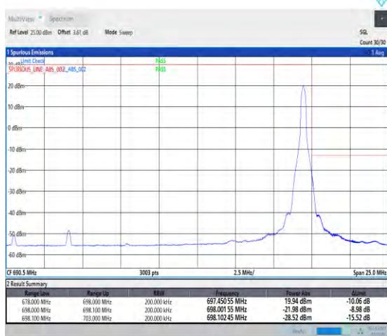
1-N71-PC3-15-20-H-5-CP-QPSK-Edge_1RB_Right-1@105-Ant1-1--PASS-see graph
