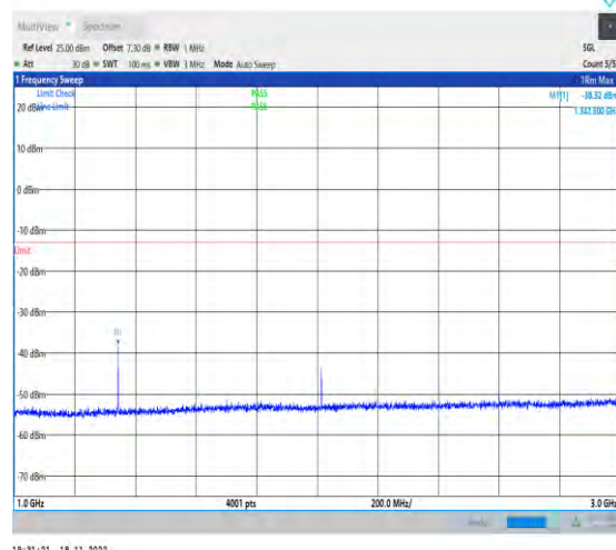
1-N71-PC3-15-20-M-1-DFT-PI2BPSK-Inner_1RB_Lef t-1@1-1000-3000-Ant1-1342.50--38.32--13-PASS
