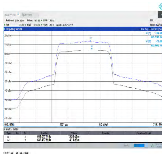
1-N71-PC3-15-20-M-2-CP-256QAM-Outer_Full-106 @0-Ant1-9.21-100%-0.00-9.21-PASS-≤13
