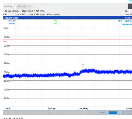
1-N71-PC3-15-20-M-1-DFT-PI2BPSK-Inner_1RB_Lef t-1@1-12000-20000-Ant1-16916.80--44.61--13-PASS
