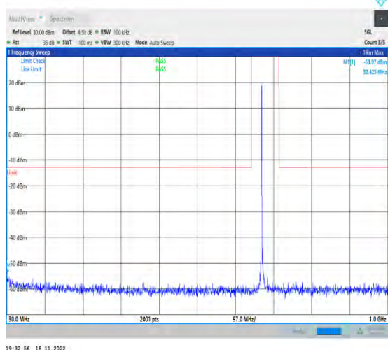
1-N71-PC3-15-20-H-1-DFT-PI2BPSK-Inner_1RB_L eft-1@1-30-1000-Ant1-32.43--53.97--13-PASS
