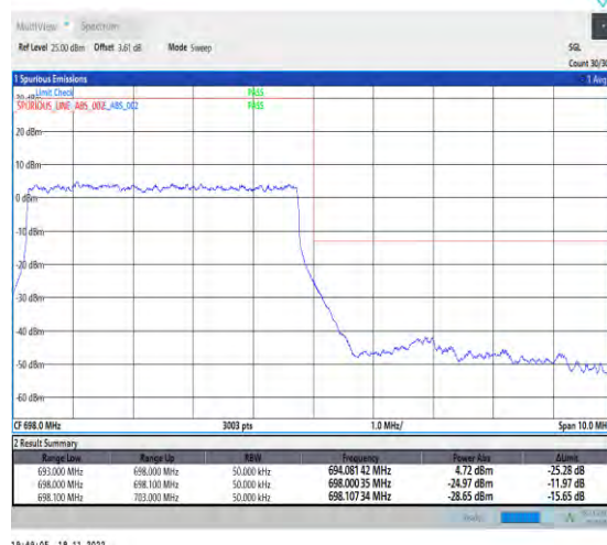
1-N71-PC3-15-5-H-3-DFT-PI2BPSK-Outer_Full-25@0-Ant1-1--PASS-see graph
