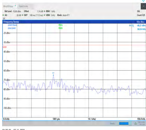
1-N71-PC3-15-20-H-1-DFT-PI2BPSK-Inner_1RB_L eft-1@1-0.009-0.15-Ant1-0.06--66.21--33-PASS
