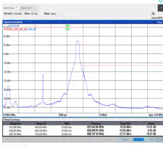
1-N71-PC3-15-5-H-5-CP-QPSK-Edge_1RB_Right-1@24-Ant1-1--PASS-see graph
