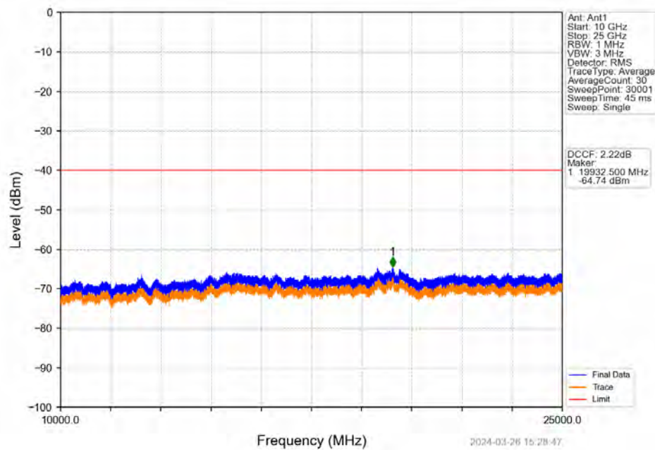
Band48_5MHz_QPSK_MCH_3625MHz_RB_1_0_NTNV
