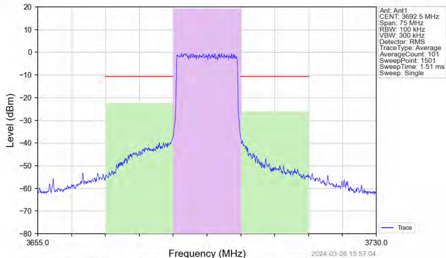
Band48_15MHz_QPSK_HCH_3692.5MHz_RB_75_0_NTNV
