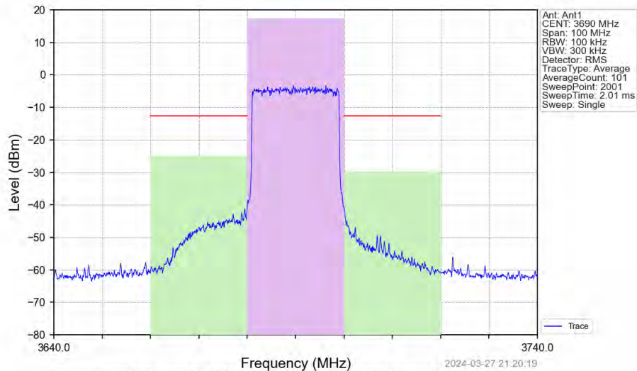
Band48_20MHz_64QAM_HCH_3690MHz_RB_100_0_NTNV
