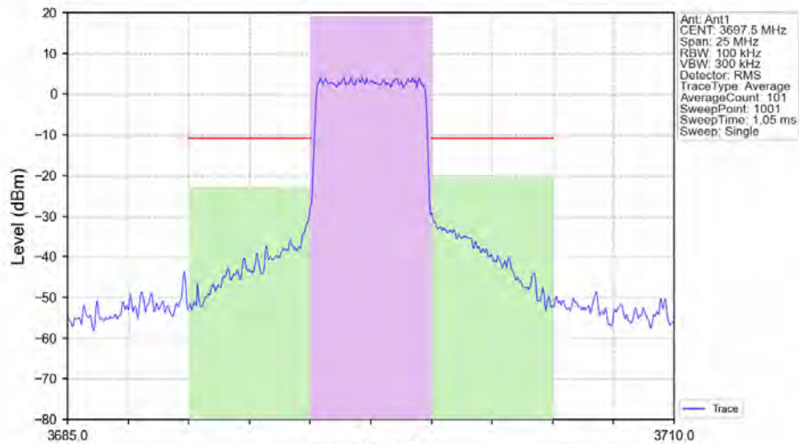
Band48_5MHz_QPSK_HCH_3697.5MHz_RB_25_0_NTNV
