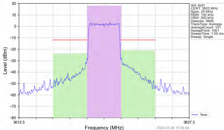
Band48_5MHz_16QAM_MCH_3625MHz_RB_25_0_NTNV
