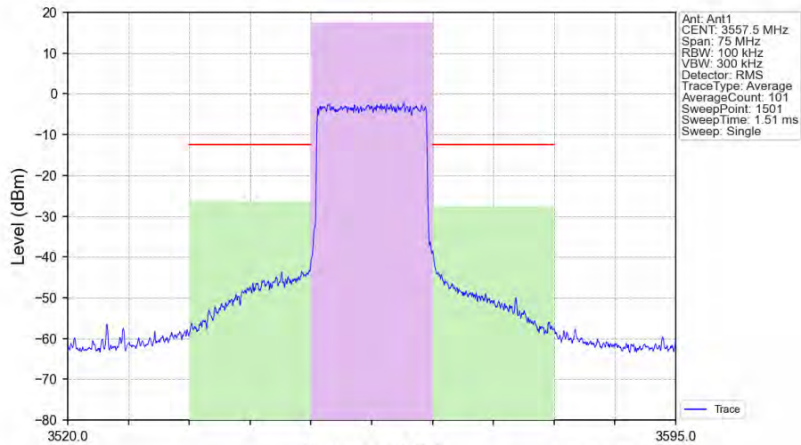
Band48_15MHz_64QAM_LCH_3557.5MHz_RB_75_0_NTNV
