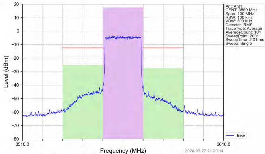
Band48_20MHz_64QAM_LCH_3560MHz_RB_100_0_NTNV
