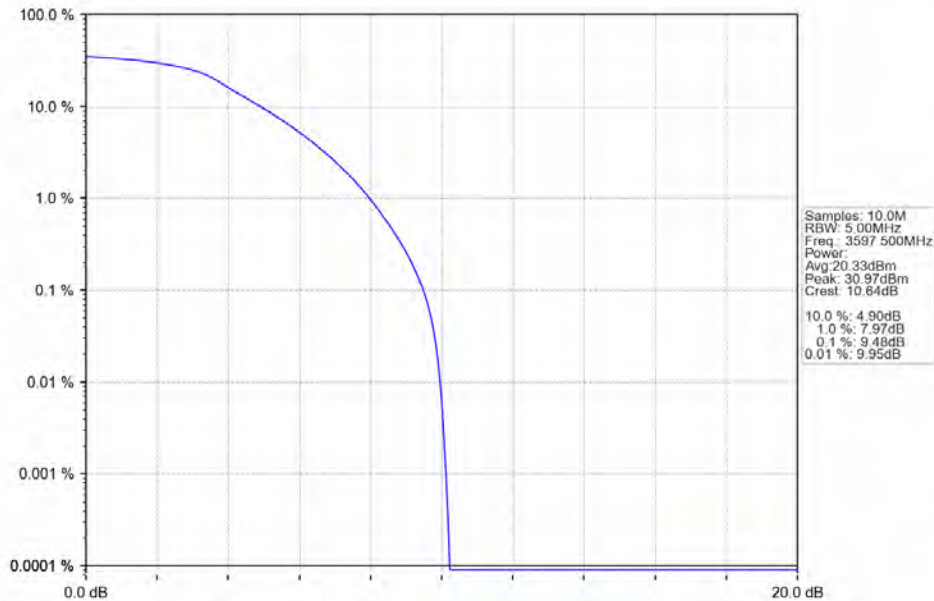
Band42c 5MHz_QPSK_HCH_3597.5MHz_RB_25_0_NTNV
