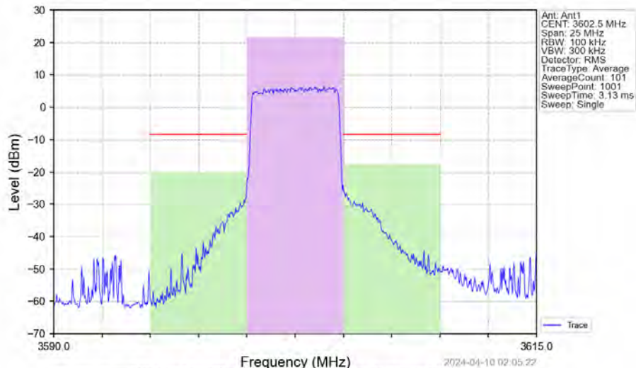
Band43c_5MHz_64QAM_LCH_3602.5MHz_RB_25_0_NTNV
