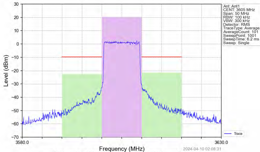
Band43c_10MHz_64QAM_LCH_3605MHz_RB_50_0_NTNV
