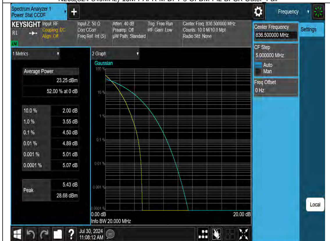
N26a(824-849MHz)-15M-PAPR-M-CP-OFDM-QPSK-Outer Full
