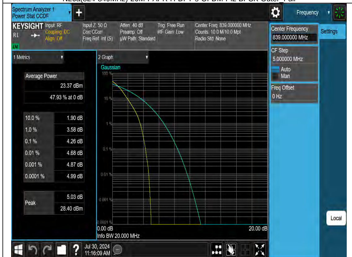
N26a(824-849MHz)-20M-PAPR-H-CP-OFDM-QPSK-Outer Full
