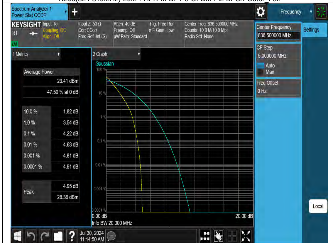
N26a(824-849MHz)-20M-PAPR-M-CP-OFDM-QPSK-Outer Full
