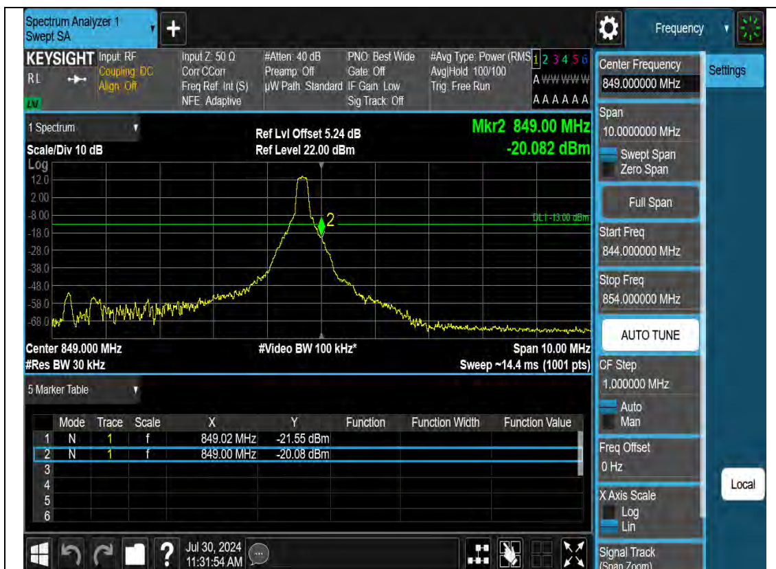
N26a(824-849MHz)-10M-Bandedge-L-DFT-s-OFDM-Pi2 BPSK-Outer_Full
