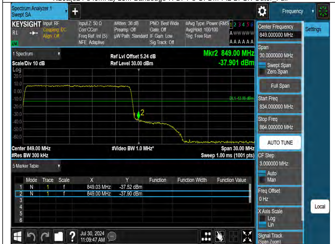
N26a(824-849MHz)-15M-Bandedge-H-DFT-s-OFDM-Pi2 BPSK-1RB MAX
