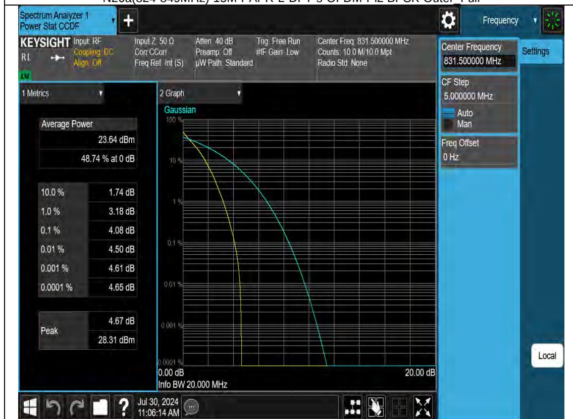
N26a(824-849MHz)-15M-PAPR-L-CP-OFDM-QPSK-Outer Full
