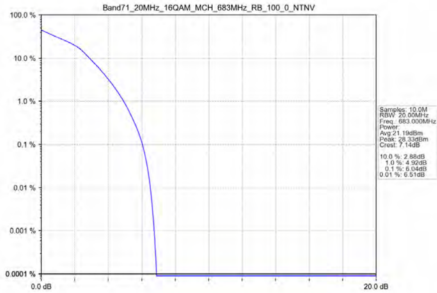
Band71_20MHz_16QAM_MCH_683MHz_RB_100_0_NTNV
