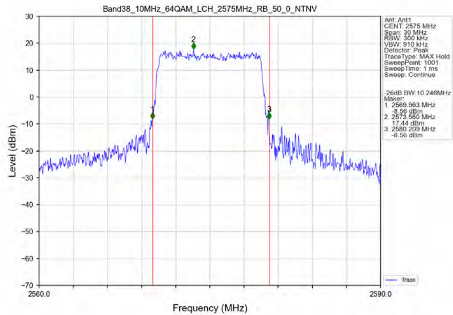
Band38_10MHz_64QAM_LCH_2575MHz_RB_50_0_NTNV
