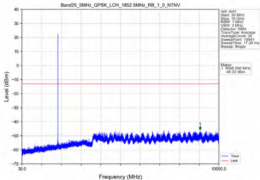
Band25 5MHz QPSK LCH 1852.5MHz RB 1 0 NTNV
