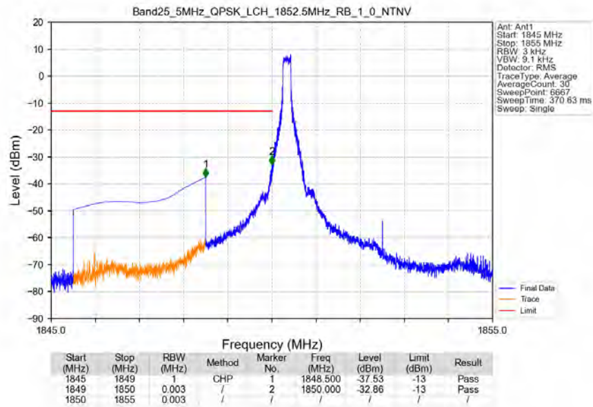
Band25 5MHz QPSK LCH 1852.5MHz RB 1 0 NTNV
