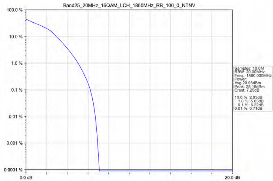
Band25_20MHz_16QAM_LCH_1860MHz_RB_100_0_NTNV
