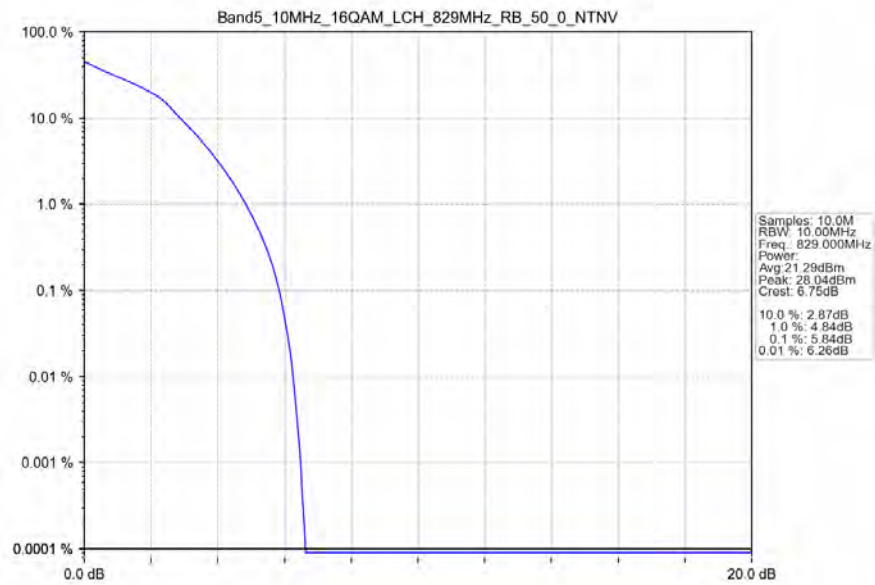
Band5_10MHz_16QAM_LCH_829MHz_RB_50_0_NTNV
