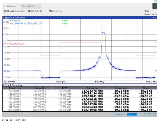
Band14-5MHz-QPSK-23305-6RB#0
