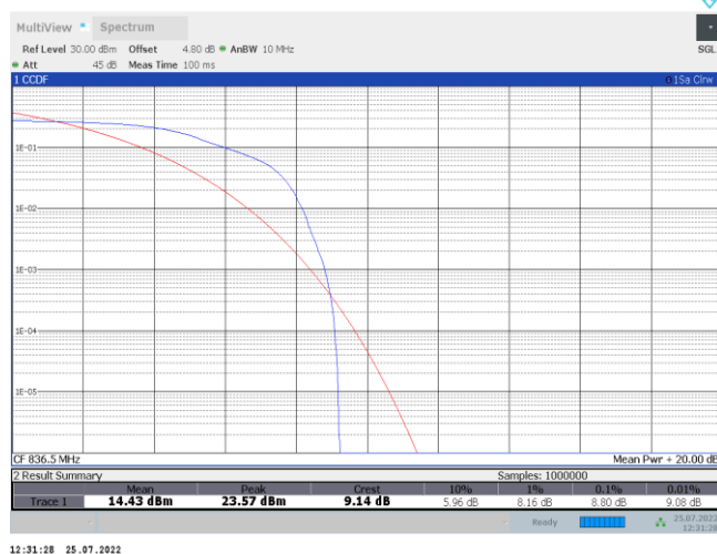
Band5-5MHz-QPSK-20525-6RB#0
