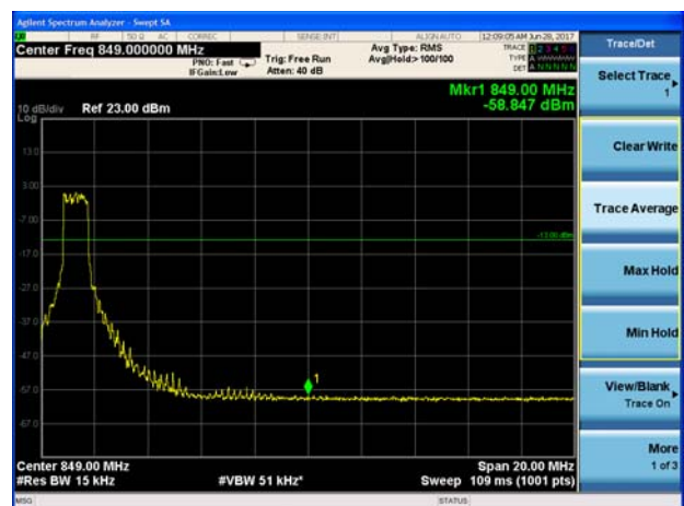
LTE Band 5 16QAM 10MHz CH-High 100%RB
