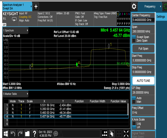
11AX80MIMO_Ant1_Low_5530_Peak
