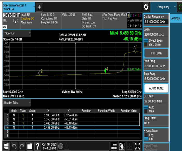
11AC40MIMO_Ant1_Low_5510_Peak
