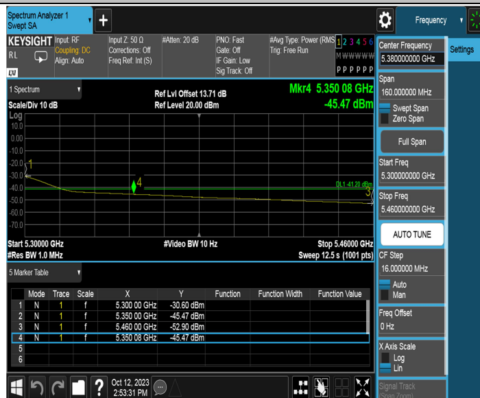
11N40MIMO_Ant2_High_5310_Peak
