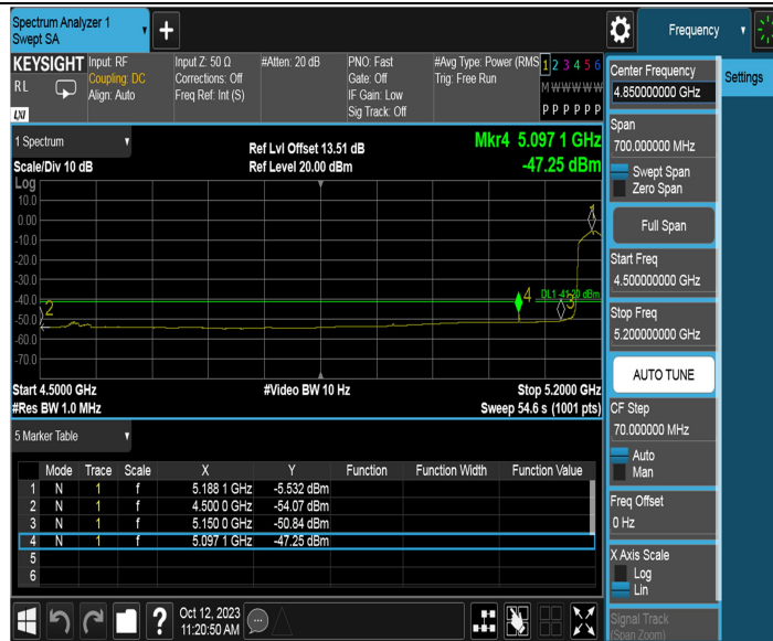
11N40MIMO_Ant1_Low_5190_Peak
