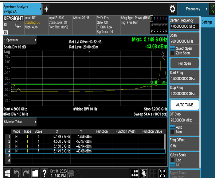
11N20MIMO_Ant2_Low_5180_Peak
