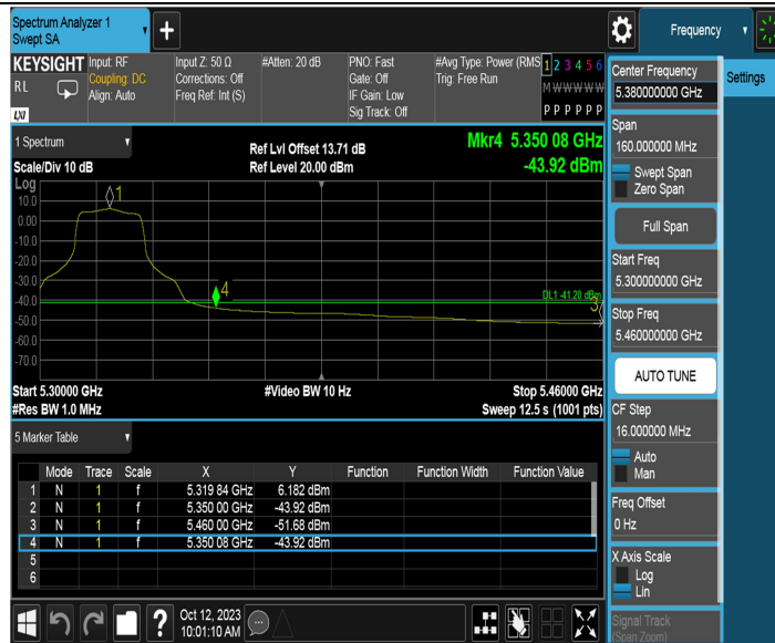
11N20MIMO_Ant2_High_5320_Peak
