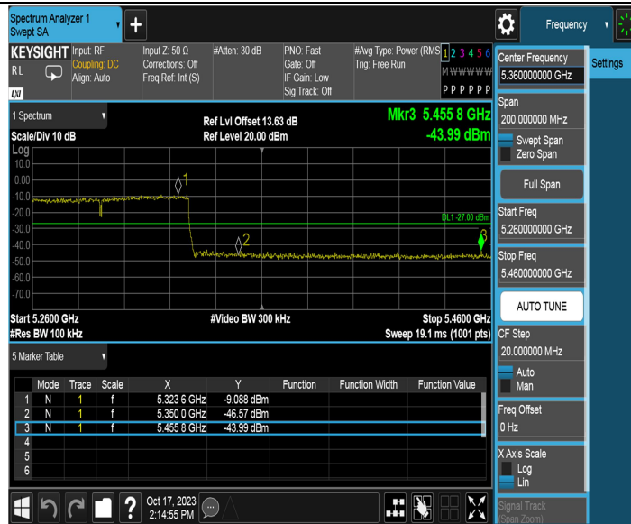
11AC80MIMO_Ant2_High_5290
