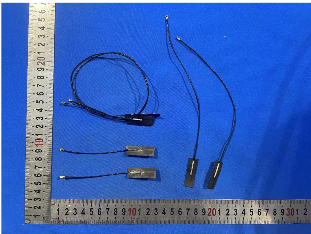
Photo 4: Internal View for WiFi Antenna
