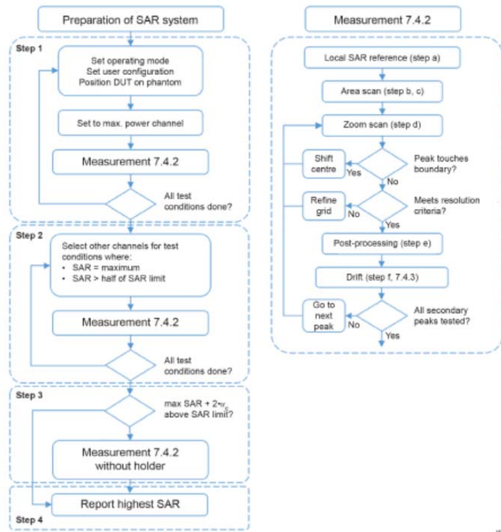
Fig 11.1 Block diagram of the tests to be performed
