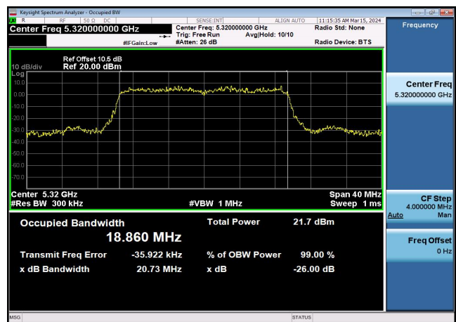
U-NII-2a 99%&26dB Bandwidth-802.11ax(20MHz )5320MHz,Ant1
