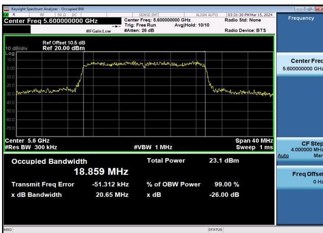
U-NII-2c 99%&26dB Bandwidth-802.11ax(20MHz ) ,5600MHz,Ant1
