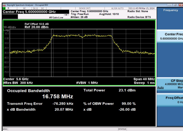
U-NII-2c 99%&26dB Bandwidth-802.11a(20MHz) ,5600MHz,Ant1
