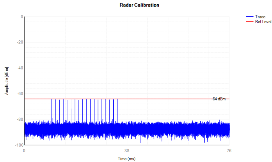
Radar Signal 5260
