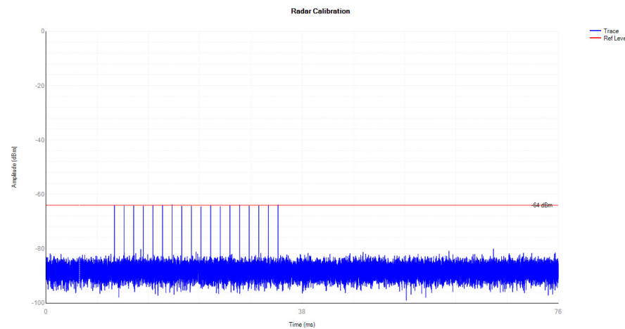
Radar Signal 5500
