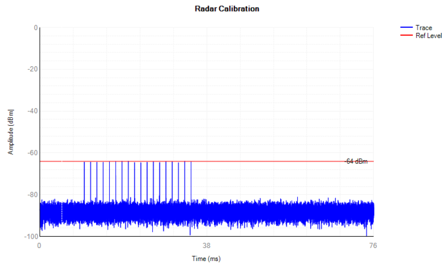
Radar Signal 5270
