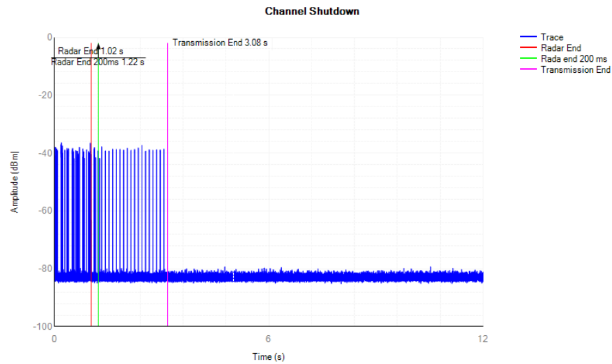
802.11n40 channel 54 5270MHz
