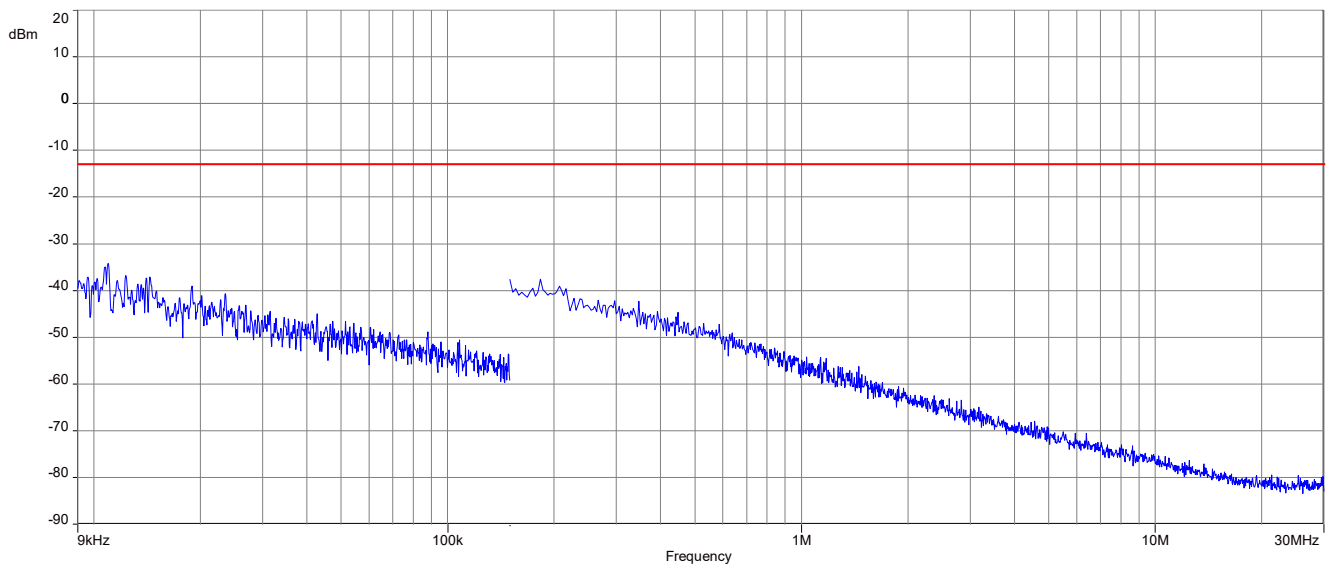
Plot 4: Middle channel (9 kHz - 30 MHz)
