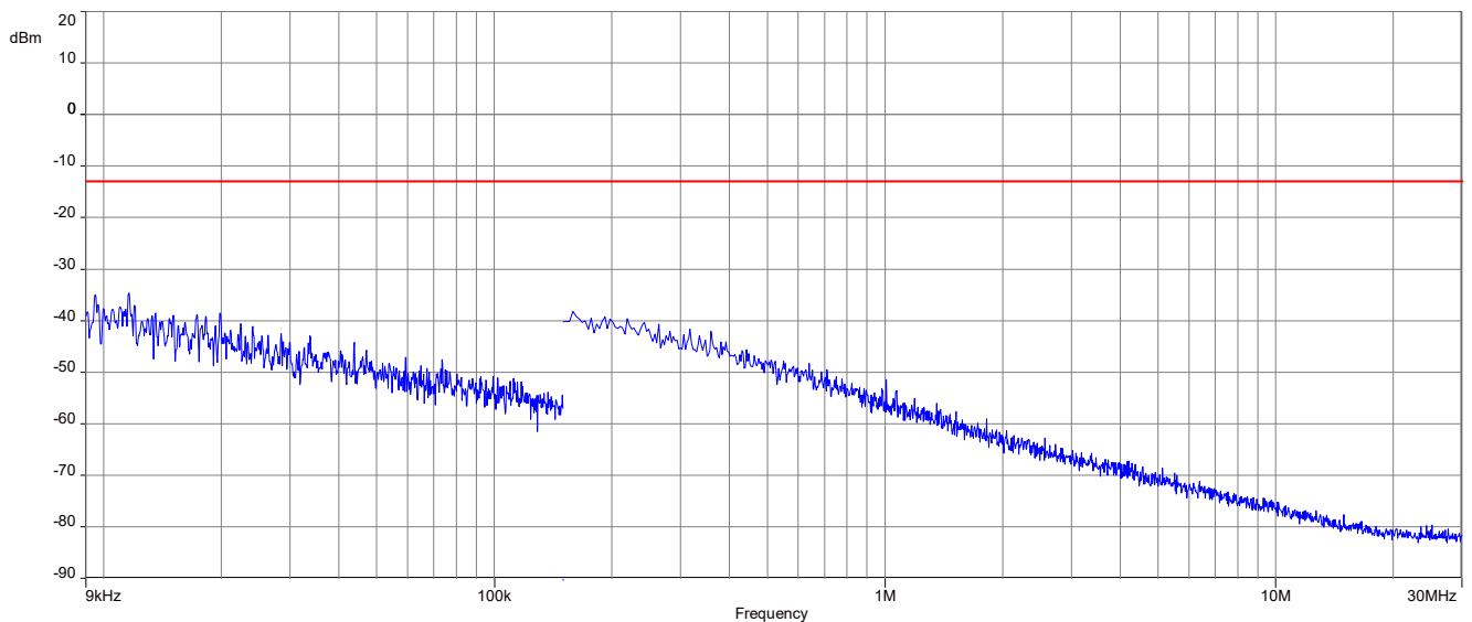
Plot 4: Middle channel (9 kHz - 30 MHz)
