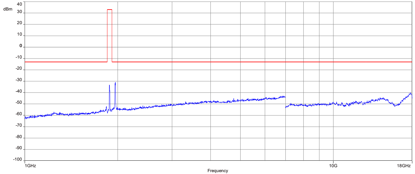
Plot 7: Middle channel (1 GHz – 18 GHz)
