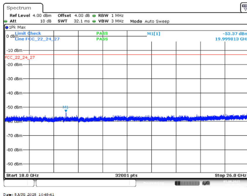
Plot 4: Middle channel, 18 GHz to 26 GHz, valid for both modulations
