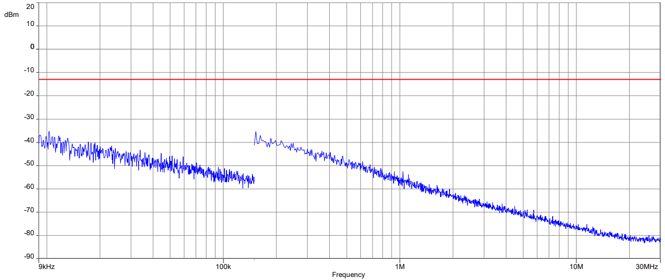
Plot 5: Middle channel (9 kHz - 30 MHz)
