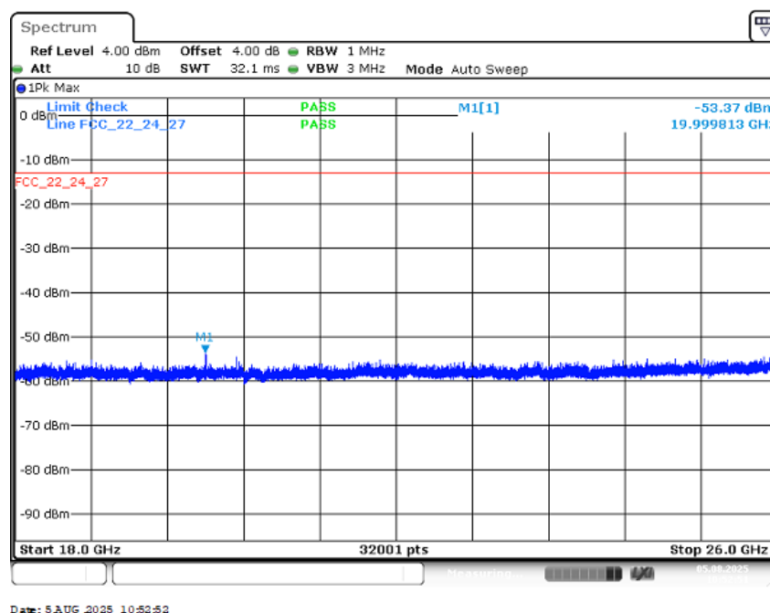
Plot 4: Middle channel (18 GHz – 26 GHz); , valid for both modulations
