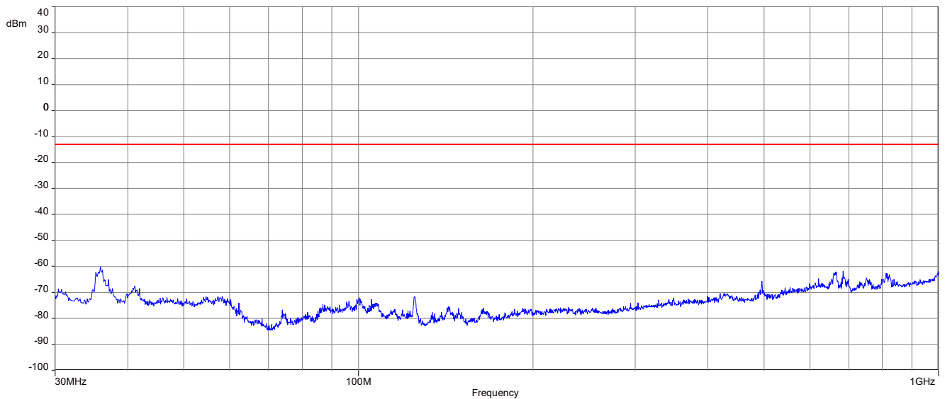
Plot 6: Middle channel (30 MHz – 1 GHz)
