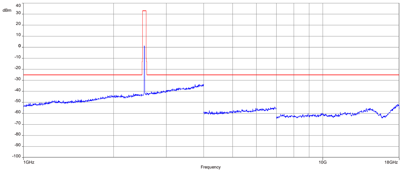
Plot 7: Middle channel (1 GHz – 18 GHz)
