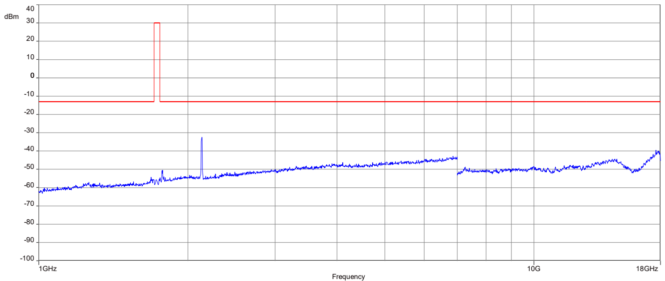
Plot 6: Middle channel (1 GHz – 18 GHz)
