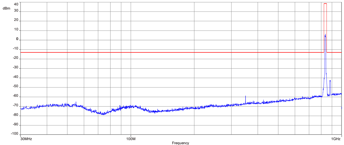
Plot 5: Middle channel (30 MHz – 1 GHz)
