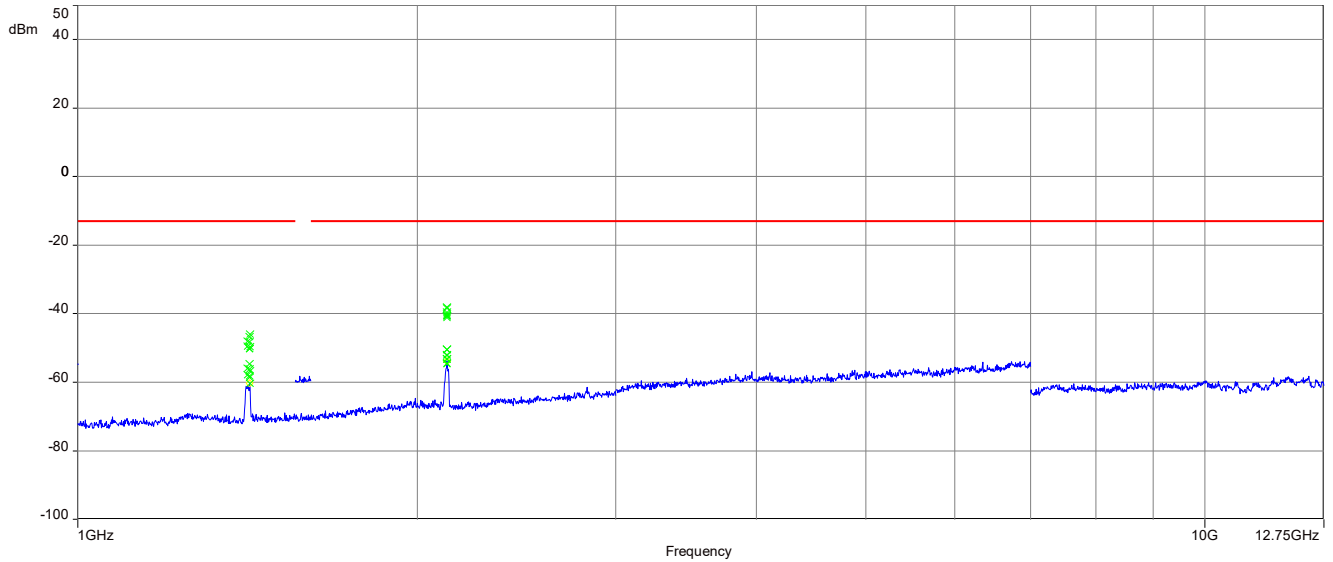
Plot 3: Middle channel (1 GHz – 12.75 GHz)
