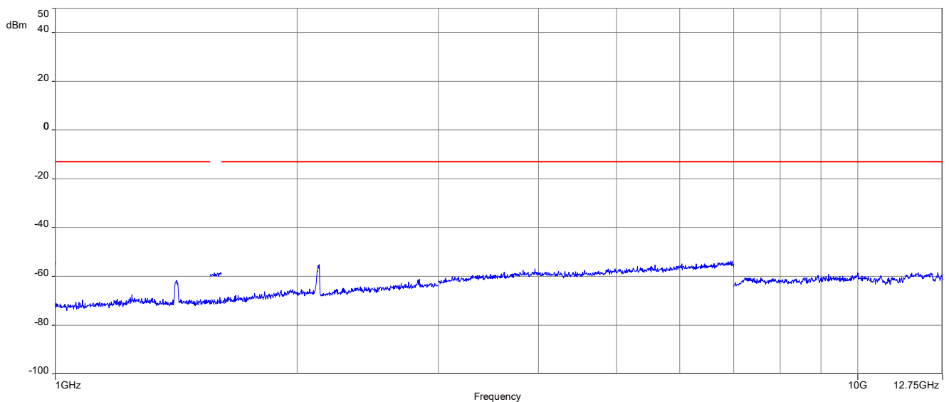
Plot 6: Middle channel (1 GHz – 12.75 GHz)
